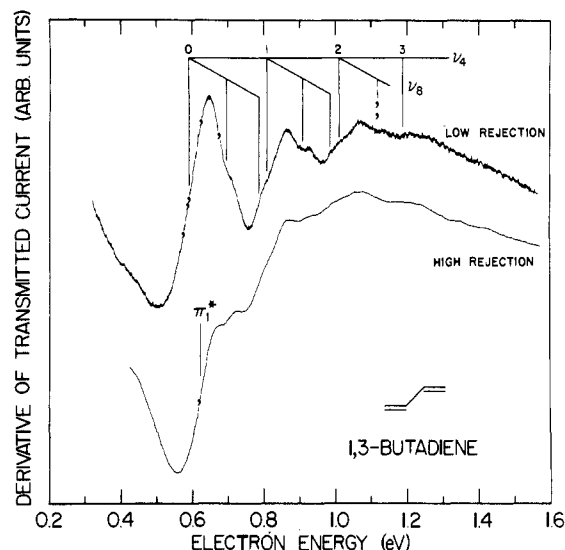
Figure 6. Expanded view of the electron transmission spectrum of 1,3-butadiene near the lowest shape resonance. The curve labeled "high rejection" displays the structure as derived from the total scattering cross section. The "low rejection" curve is derived from a partial cross section integrated over scattering angles around the back direction.
