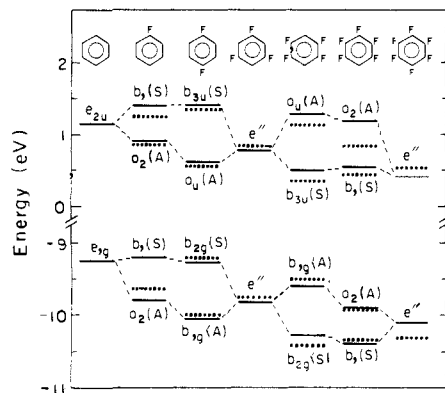
Figure 32. Correlation diagram for the vertical EA's and IP's of benzene and various fluorosubstituted benzenes. The solid lines refer to the experimental values and the dots to the values obtained from the two-parameter induction-resonance model. The orbitals are labeled S or A, depending on whether they are symmetric or antisymmetric on reflection in the plane passing through the C_1 and C_4 carbons and perpendicular to the plane of the ring. Reprinted with permission from ref 154. Copyright 1979 American Institute of Physics.
