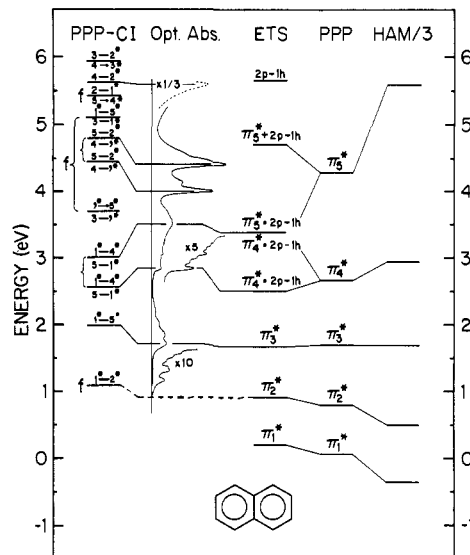
Figure 17. Comparison of naphthalene anion energies derived from ETS, CI, and PPP calculations. The energy scale for the optical absorption data has been shifted so that its zero lies at +0.19 eV in agreement with ETS. On the left, energies from PPP-CI calculations are shown along with the major contributing configurations. The \pi orbitals are abbreviated by 1-5 (bonding) and 1*-5* (antibonding). Optically forbidden transitions from the anion ground state are labeled with "f". States of the same configuration are connected with brackets. Reprinted with permission from ref 109. Copyright 1987 American Institute of Physics.
