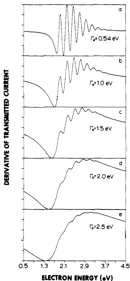
Figure 3. Derivative of transmitted current in N_2 as a function of energy computed with the boomerang model: (a) all parameters as derived by Dubé and Herzberg for a best fit to the experimental data; (b–e) show the effect of increasing the width of the resonance to the values shown. Reprinted with permission from ref 24. Copyright 1981 American Institute of Physics.
