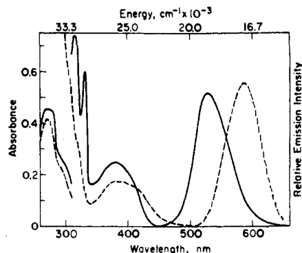
Figure 15. Electronic absorption (left) and emission (right) spectra of \text{ClRe}(\text{CO})_3(\text{phen}) in EPA at 77 K (—) and 298 K (---). Room temperature absorption maxima are at 26\,100 \text{ cm}^{-1} ( \epsilon 4000) and 37\,030 \text{ cm}^{-1} ( \epsilon 30600). The low-temperature spectrum is uncorrected for solvent contraction, and the emissions at 77 and 298 K were not recorded at the same sensitivity. Reproduced with permission from ref 130. Copyright 1974 American Chemical Society.
