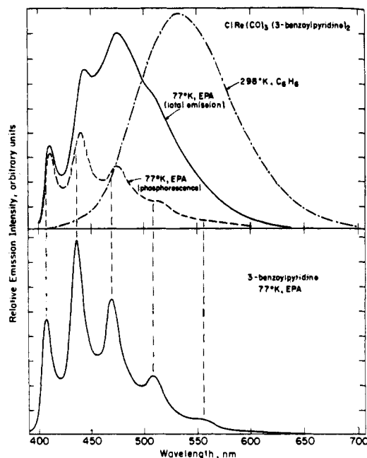
Figure 22. Corrected emission spectra of \sim 10^{-4} M \text{ClRe}(\text{CO})_3(3\text{-BN-py})_2 and \sim 10^{-4} M 3-BN-py following excitation at 330 nm. The spectra are not shown at the same sensitivity. All spectra are total emission spectra except the one marked "phosphorescence", which was recorded with a phosphoroscope in place during spectral acquisition. The phosphoroscope allows only the detection of emission longer than \sim 1.0 ms. Reproduced with permission from ref 181. Copyright 1978 American Chemical Society.
