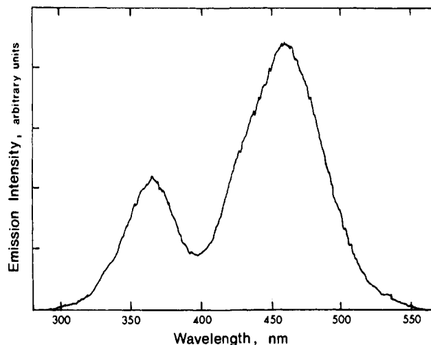
Figure 9. Emission excitation spectrum of 10^{-4} \text{ M Mo}(\text{CO})_5(4\text{-BN-py}) in benzene at 298 K. The excitation spectrum was recorded with emission monitored at 640 nm. Reproduced with permission from ref 82. Copyright 1986 American Chemical Society.
