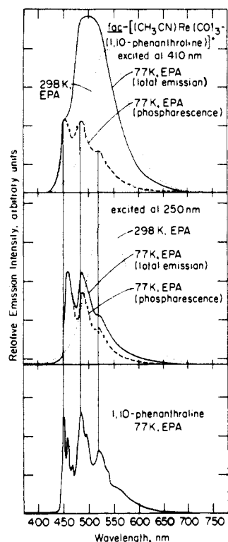
Figure 16. Emission spectra excited at 410 nm (top) and 250 nm (middle) for \sim 10^{-4} M fac-[(CH_3CN)Re(CO)_3(phen)](CF_3SO_3)^+ in EPA. The total emission of phen (bottom) is shown for comparison. The spectra are not shown at the same sensitivity. All spectra are total emission spectra except the two marked "phosphorescence", which were recorded with the phosphoroscope attachment in place. The phosphoroscope allows only the detection of emissions longer than \sim 50 \mu s. Reproduced with permission from ref 163. Copyright 1979 American Chemical Society.
