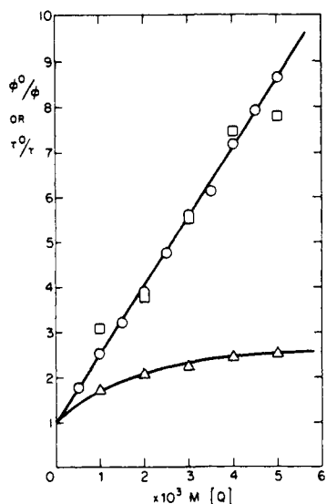
Figure 8. Quenching of \text{W}(\text{CO})_5(4\text{-CN-py}) photosubstitution quantum yields ( \phi ) and emission lifetimes ( \tau ) at 298 K by anthracene in methylcyclohexane containing 0.05 M ethanol (O \tau^0/\tau ; \square \phi^0/\phi ; \Delta \phi^0/\phi ). Excitation wavelengths are (O) 530, ( \square ) 520, and ( \Delta ) 430 nm. The 530-nm wavelength corresponds to MLCT excitation; the 430-nm wavelength corresponds to excitation into overlapping LF and MLCT states. Reproduced with permission from ref 80. Copyright 1982 American Chemical Society.
