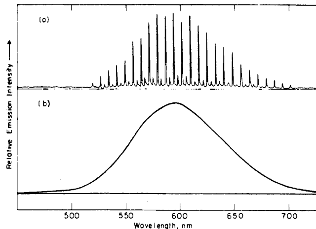
Figure 36. (a) Electrogenerated chemiluminescence from a 0.1 M ( n -Bu 4 N)ClO 4 CH 3 CN solution of fac -ClRe(CO) 3 (phen). The potential of the working Pt electrode was stepped from +1.6 to -1.6 V (vs. Ag wire) at a frequency of 0.2 Hz. (b) Optically (420 nm) excited luminescence from solution in (a). Figure reproduced with permission from ref 164. Copyright 1978 American Chemical Society.
