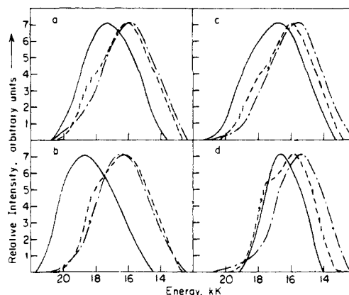
Figure 7. Corrected emission spectra at 298 K of (a) W(CO)_5(4\text{-AC-py}) , (b) W(CO)_5(4\text{-BN-py}) , (c) W(CO)_5(4\text{-CN-py}) , and (d) W(CO)_5(4\text{-FM-py}) ; (—) solid, (---) (6-8) \times 10^{-5} M W(CO)_5L in methylcyclohexane and (-·-) (4-6) \times 10^{-5} M W(CO)_5L in benzene. Intensities are scaled to make maxima equal. Excitation wavelength is 400 nm. Reproduced with permission from ref 80. Copyright 1982 American Chemical Society.
