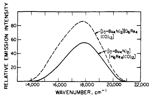
Figure 25. Corrected emission spectra for [n-Bu_4N]_2[H_6Re_4(CO)_{12}] (—) and [n-Bu_4N]_2[D_6Re_4(CO)_{12}] (---) in 2-methyltetrahydrofuran at 77 K. The excitation wavelength is 375 nm. Reproduced with permission from ref 195. Copyright 1981 American Chemical Society.
