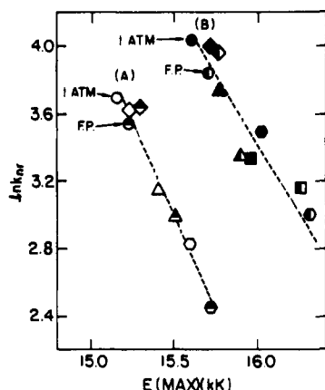
Figure 17. Plot of \ln k_{nr} vs. energy of emission band maxima for (A) \text{ClRe}(\text{CO})_3(4,7\text{-Ph}_2\text{-phen}) and (B) \text{ClRe}(\text{CO})_3(\text{phen}) in various solvents (O DMF, \diamond \text{CH}_3\text{CN} , \Delta heptanol, \circ m -xylene) in the liquid phase. F.P. represents value immediately before freezing. Open and solid symbols represent 1-atm data; half-filled symbols represent data just before freezing. Reproduced with permission from ref 169. Copyright 1982 American Institute of Physics.
