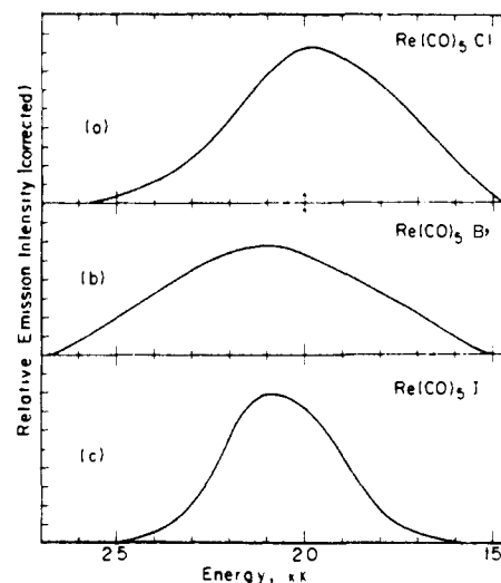
Figure 14. Corrected emission spectra of pure powdered XRe(CO)_5 at 25 K. Excitation wavelength is 370 nm. Reproduced with permission from ref 146. Copyright 1976 American Chemical Society.
