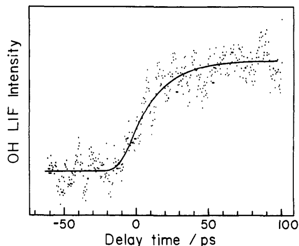
Figure 6. Time-resolved appearance of the OH fragment, measured by LIF, following photochemical initiation of the H + CO_2 reaction in the CO_2-HI complex. The solid curve is a fit of an exponential rise (eq 1) (adapted from ref 93 with permission.)
