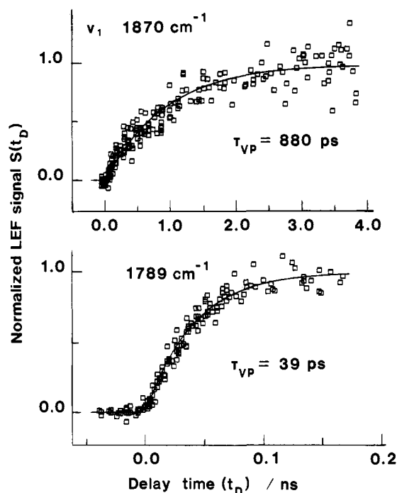
Figure 2. Time-resolved appearance of NO fragments in the X^2\Pi_{3/2} state following excitation of the \nu_1 and \nu_4 fundamentals of (NO)_2 . The solid curves are least-squares fits of eq 1.
