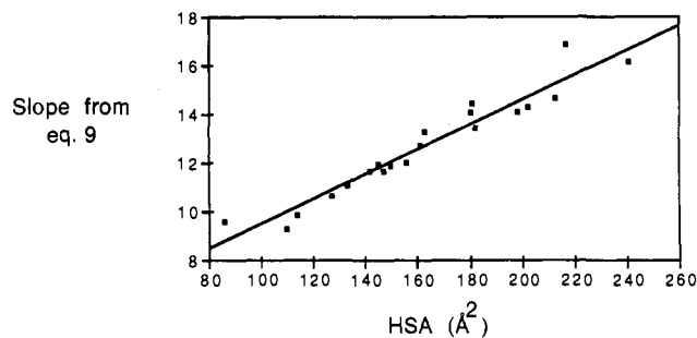
Figure 7. Slopes of plots from eq 9 vs hydrocarbonaceous surface area (HSA) of solutes, verifying the linear dependence on n . Sepralyte C 18 column, acetonitrile/water mobile phases.
