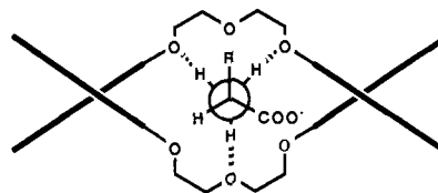
Figure 5. Energetically favored diastereomeric complex between a chiral crown ether and an amino acid zwitterion. Space-filling models of the two diastereomeric complexes predicted this to be the more stable diastereomeric complex based primarily on steric interactions between the R and carboxylate groups of the amino acid zwitterion and the naphthyl rings of the crown ether (see ref 63–70). Amino acids with the largest R groups show the highest degree of chiral recognition with the chiral crown ether.
