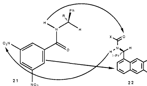
Hydrogen-bonding model (non-intercalative)
