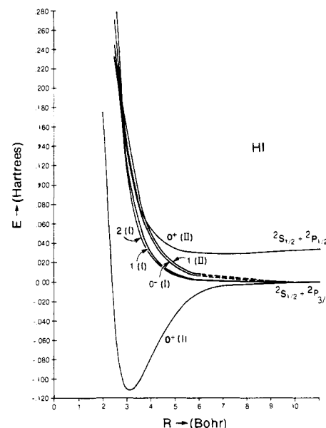
Figure 19. Potential energy curves for six low-lying states of HI (reprinted from ref 122; copyright 1985 Elsevier Science Publishers B.V.). See Table 11 for assignments of known states.
