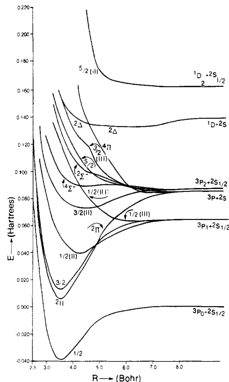
Figure 29. RCI potential energy curves of the low-lying states of \text{BiH}^+ (reprinted from ref 182; copyright 1986 American Chemical Society).
