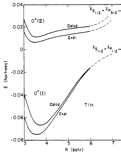
Figure 22. Comparison of the theoretical and experimental potential energy curves of two electronic states of TIH (reprinted from ref 28; copyright 1982 American Institute of Physics). See Table 12 for assignments of known states.
