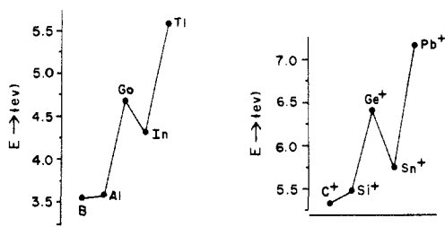
Figure 48. (ns^2np^1)^2P-(ns^1np^2)^4P energy separations of B-Tl and C^+-Pb^+ (reprinted from ref 13; copyright 1989 American Chemical Society).
