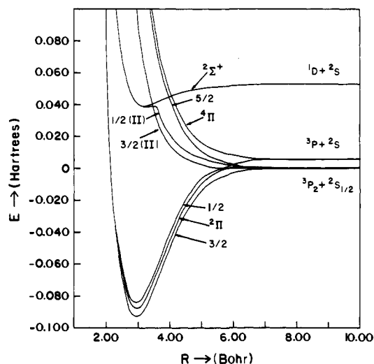
Figure 5. Potential energy curves of low-lying electronic states of SeH (reprinted from ref 75; copyright Elsevier Science Publishers B.V.). See Table 5 for assignments of known states.
