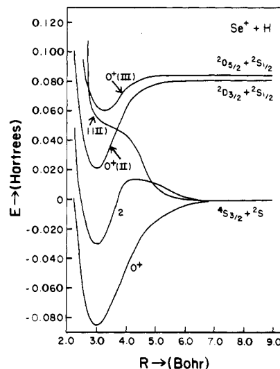
Figure 6. Potential energy curves of low-lying electronic states of SeH + (reprinted from ref 75; copyright 1987 Elsevier Science Publishers B.V.). See Table 5 for assignments of known states.
