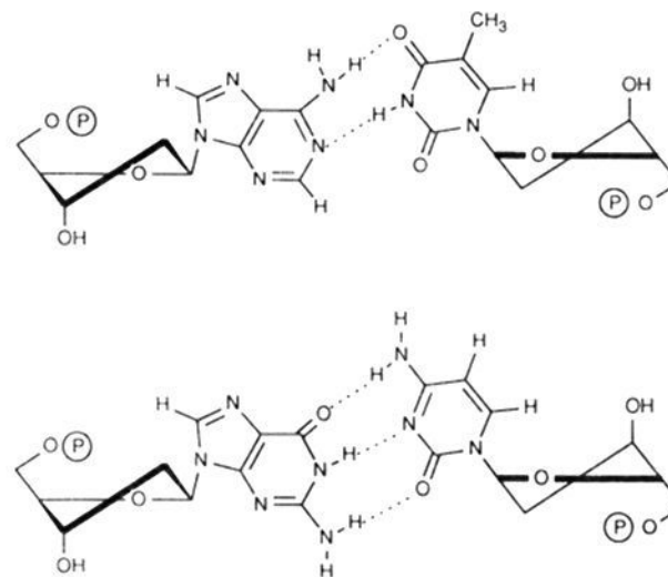
Figure 1. Watson-Crick base pairing.
