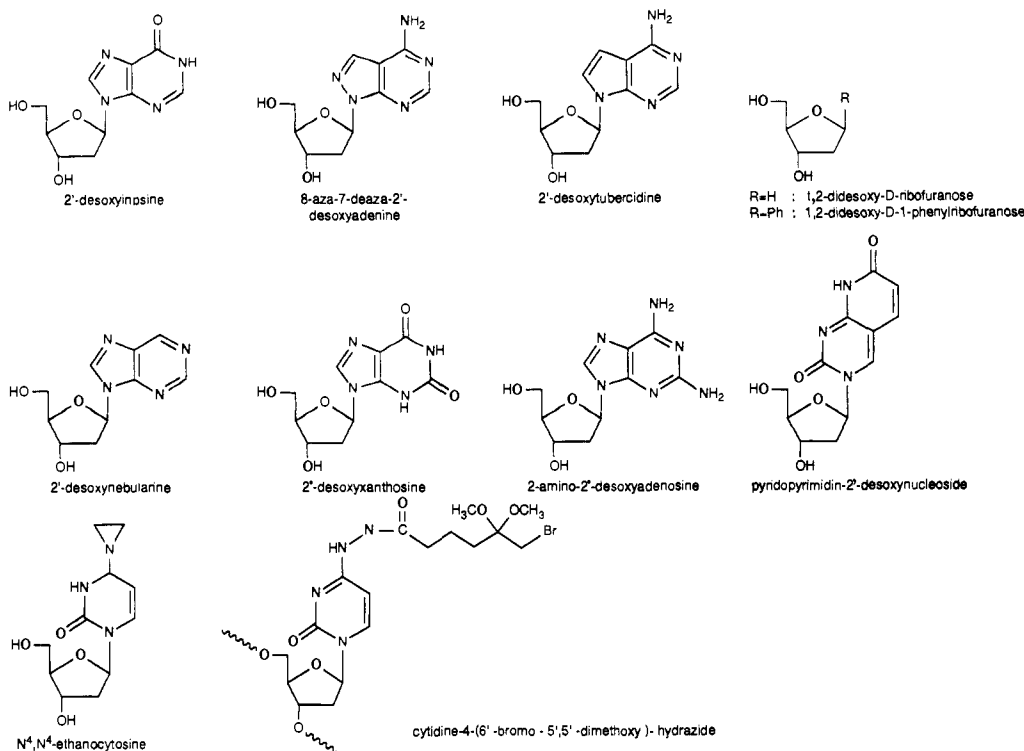
Figure 33. Base-modified nucleosides.
