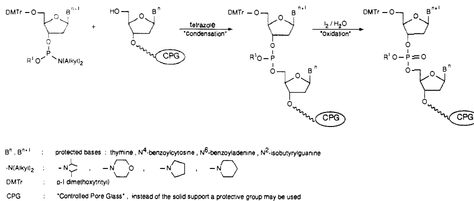
Figure 3. Amidite method.
