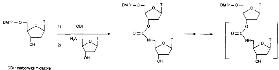
Figure 28. Synthesis of carbamate-bridged oligonucleotides.
