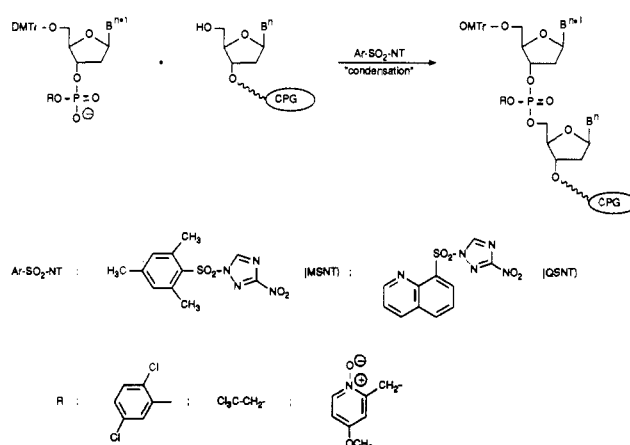
Figure 5. Phosphotriester method.
