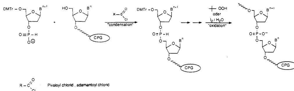
Figure 4. H-Phosphonate method.
