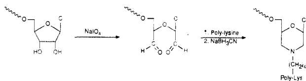
Figure 42. Synthesis of a 3'-polylysine conjugate.
