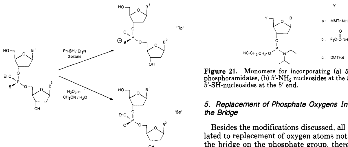
Figure 20. Assignment of configuration of phosphotriesters by stereoselective conversion of thiono triesters to thioates or phosphotriesters.
