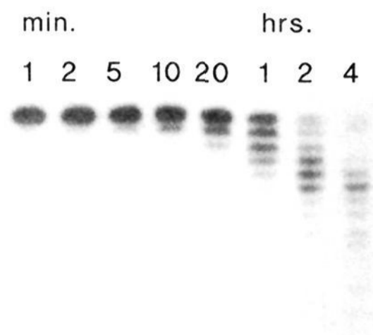
Figure 46. Kinetics of exonucleolytic cleavage of a radiolabeled 20-mer oligonucleotide in fetal calf serum (12% polyacrylamide gel).
