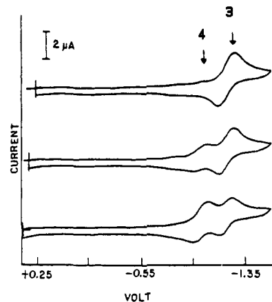
Figure 7. Cyclic voltammograms of 3.5 \times 10^{-4} M \text{Cp}_3\text{Rh}_3(\mu_2\text{-CO})_2(\text{CO}) (3) ( \text{Cp} = \eta^5\text{-C}_5\text{H}_5 ) in tetrahydrofuran as a function of initial potential: +0.25 V (top), +0.30 V (middle), and +0.35 V (bottom). Conditions: T = 298 \text{ K} , v = 0.20 \text{ V/s} . The small feature at ca. +0.30 V is due to an impurity. Reprinted from ref 164; copyright 1989 American Chemical Society.
