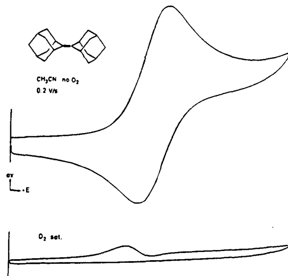
Figure 6. Cyclic voltammograms of adamantylideneadamantane in 0.1 M \text{Bu}_4\text{NClO}_4 /acetonitrile at 200 mV/s. Note that increasingly positive potentials are plotted to the right and anodic currents are directed upward. Potential range: +1.15 (left) to +1.75 V (right) vs SCE. Top: no oxygen. Bottom: oxygen-saturated solution. Reprinted from ref 161; copyright 1981 American Chemical Society.
