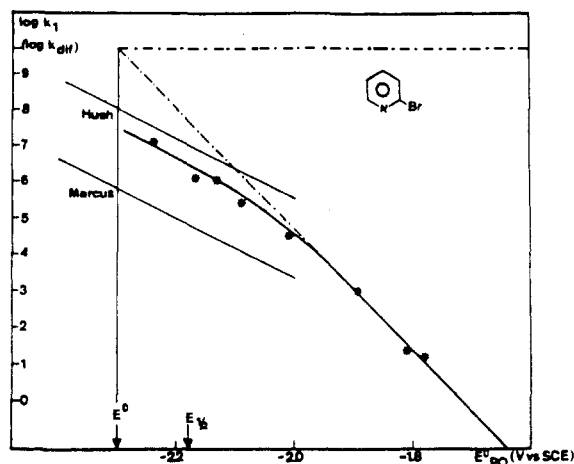
Figure 3. Rate constants for forward reaction 17 (here labeled k_1 ) vs standard potentials of various catalyst couples, reaction 16 (here labeled E_{PQ}^{\circ} ). E^{\circ} is the value of the standard potential for substrate reduction (2-bromopyridine) obtained by extrapolation to the diffusion-limited rate constant, k_{dir} . E_{1/2} is the observed irreversible half-wave potential for reduction of 2-bromopyridine. Experiments conducted with 0.1 M Bu_4NI in dimethylformamide at a hanging mercury drop electrode; T = 295 K. Reprinted from ref 62; copyright 1979 American Chemical Society.
