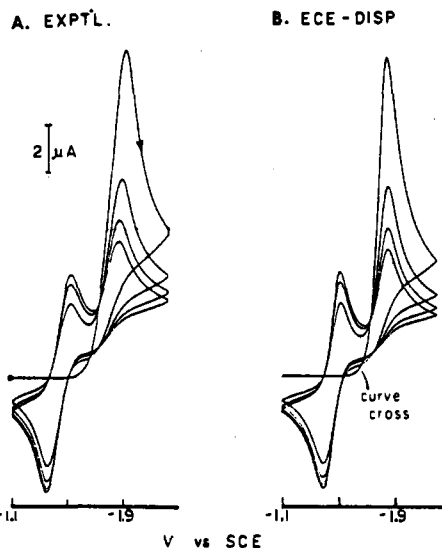
Figure 4. (A) Initial negative scan (four cycle) cyclic voltammogram of 5 \times 10^{-3} M [ trans -Mn(CO) 2 ( \eta^2 -DPPE) 2 ][PF 6 ] - (DPPE = 1,2-bis(diphenylphosphino)ethane) in 0.3 M Bu 4 NClO 4 /tetrahydrofuran at a platinum electrode at 500 mV/s. (B) Digital simulation based on eqs 23 and 24. Reprinted from ref 125; copyright 1988 American Chemical Society.
