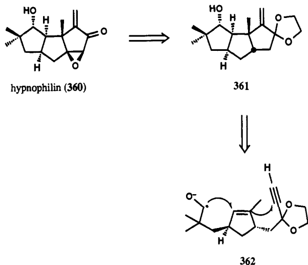
SCHEME 92
