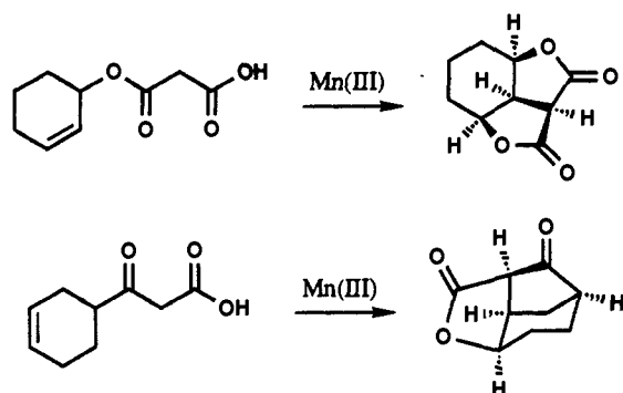
SCHEME 106
