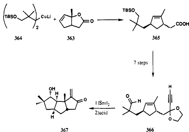
SCHEME 93
