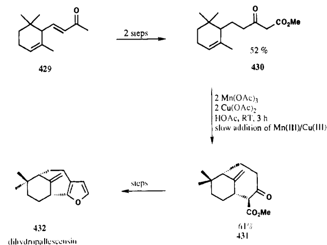
SCHEME 115
