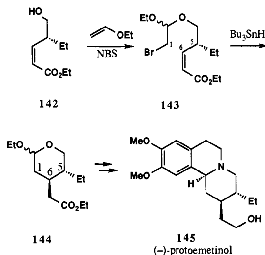
SCHEME 30
