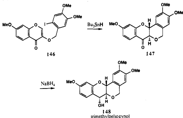
SCHEME 31
