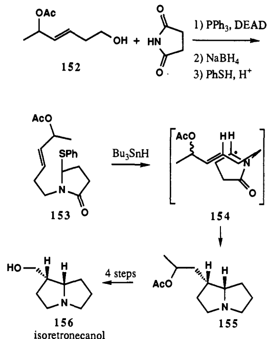
SCHEME 33
