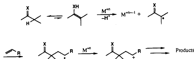
SCHEME 105
