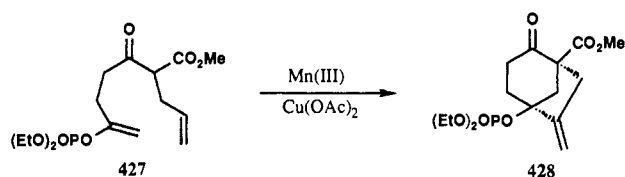
SCHEME 114
