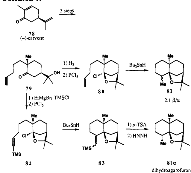
SCHEME 17
