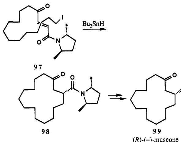
SCHEME 21
