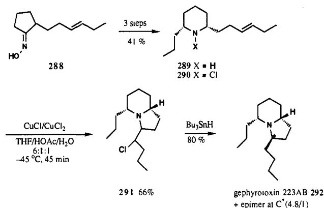
SCHEME 68
