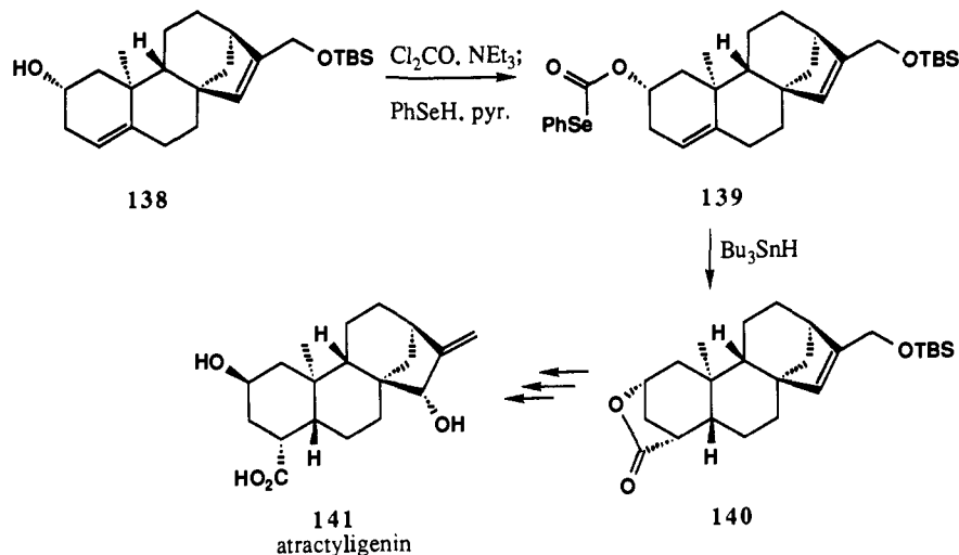
SCHEME 30
