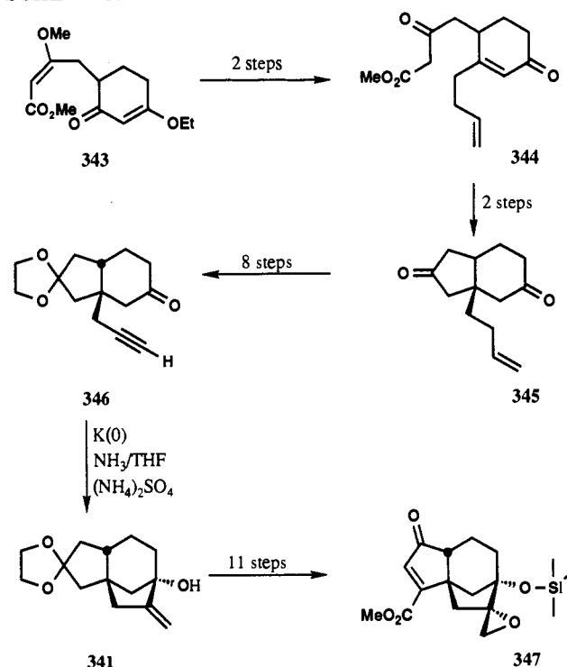
SCHEME 89
