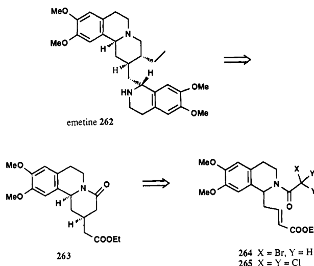
SCHEME 59
