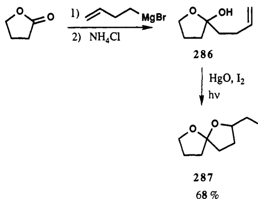
SCHEME 67
