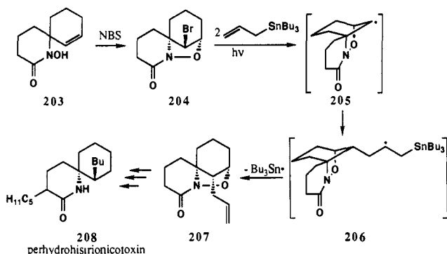
SCHEME 42
