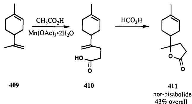
SCHEME 109
