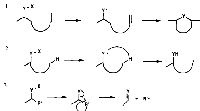
SCHEME 66
