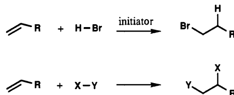
SCHEME 51
