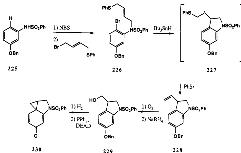
SCHEME 48
