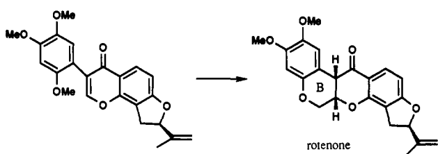
SCHEME 82
