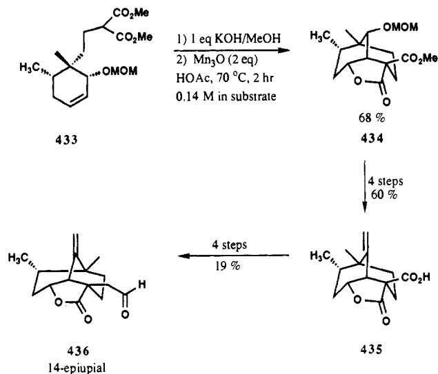
SCHEME 116
