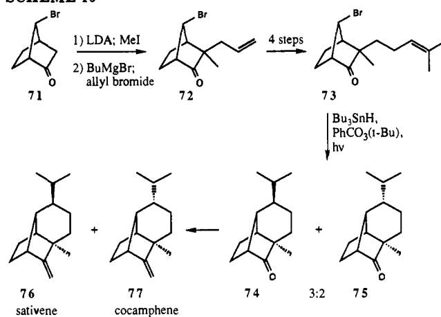
SCHEME 16
