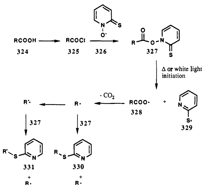
SCHEME 80
