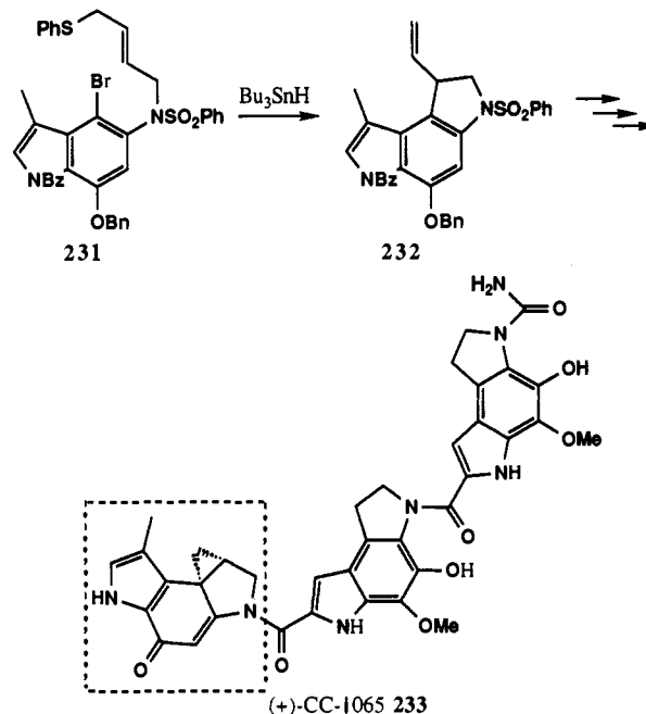
SCHEME 48
