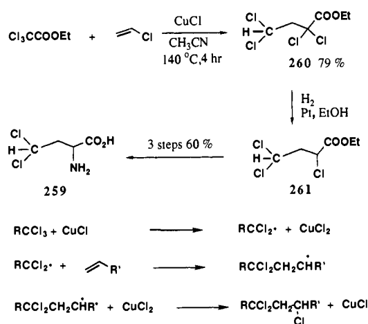
SCHEME 58
