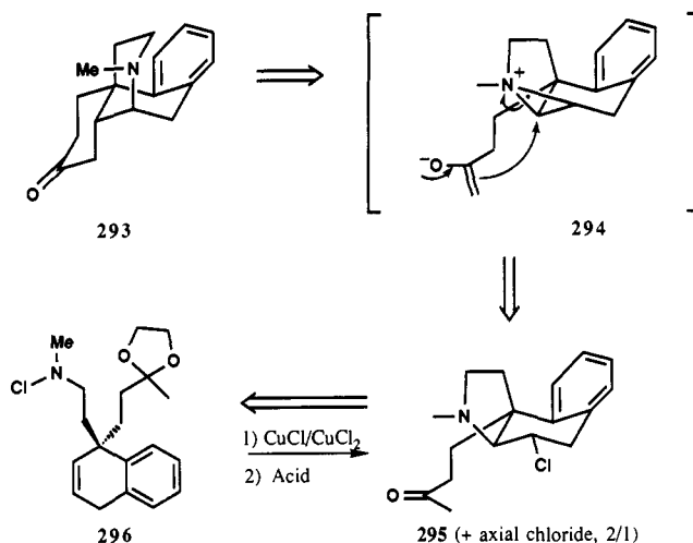
SCHEME 69
