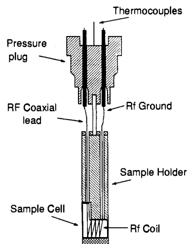
Figure 3. High-resolution sample insert of Heaton, Jonas, and co-workers. 12,13 This sample insert, described in the text, is placed inside a cylindrical high-pressure vessel.
