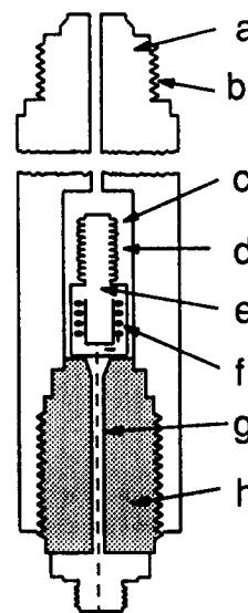
Figure 1. High-pressure NMR probe of Benedek and Purcell. 3 (a) main body of pressure bomb, (b) thread for connection to high-pressure press, (c) pressurizing fluid, led into probe via \frac{1}{8} -in. hole down along axis of probe, (d) bellows which is deformed by pressurizing fluid, (e) sample chamber, (f) rf coil, (g) rf coil leads, (h) bottom plug.
