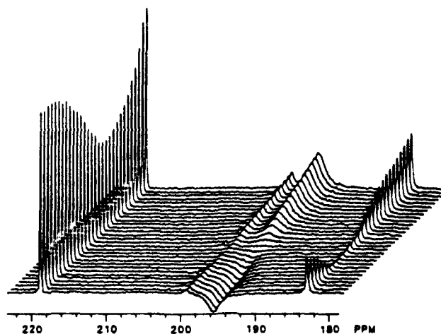
Figure 12. Observed ^{13}\text{C} NMR spectral response to selective inversion of the \text{Co}(\text{CO})_4 signal (197.1 ppm) of \text{CH}_3\text{C}(\text{O})\text{Co}(\text{CO})_4 in methylcyclohexane- d_{14} at 70^\circ\text{C} (reprinted from ref 30; copyright 1987 American Chemical Society).
