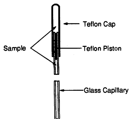
Figure 2. High pressure NMR sample cell of Earl, Vanni, and Merbach. 9 A glass capillary (Wilmad) and teflon cap are pressurized by an external pressurizing fluid to transmit pressure to a sample contained within (see text).
