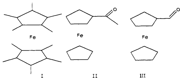
Figure 9. The molecular structures of the most representative complexes listed in Table IV: I, (\eta^5\text{-C}_5\text{Me}_5)_2\text{Fe} ; II, (\eta^5\text{-C}_5\text{H}_4\text{COMe})\text{Fe}(\eta^5\text{-C}_5\text{H}_5) ; III, (\eta^5\text{-C}_5\text{H}_4\text{COH})\text{Fe}(\eta^5\text{-C}_5\text{H}_5) .
