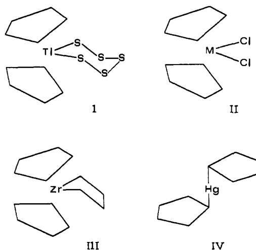
Figure 10. The molecular structures of the most representative complexes listed in Table V: I, ( \eta^5 -C 5 H 5 ) 2 TiS 5 ; II, ( \eta^5 -C 5 H 5 ) 2 MCl 2 (M = Ti, Mo, Zr); III, ( \eta^5 -C 5 H 5 ) 2 Zr( \eta^4 -C 4 H 6 ); IV, ( \eta^1 -C 5 H 5 ) 2 Hg.
