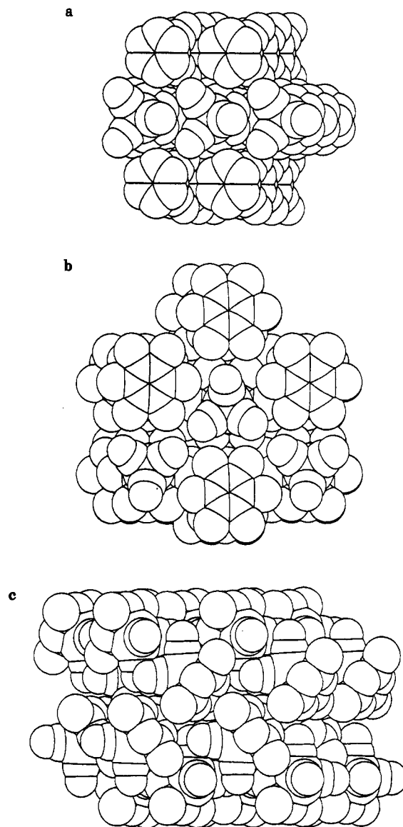
Figure 6. Comparison of the molecular organization in crystalline (\eta^6\text{-C}_6\text{H}_6)\text{Cr}(\text{CO})_3 (a), (\eta^6\text{-C}_6\text{Me}_6)\text{Cr}(\text{CO})_3 (b), and (1,3,5\text{-}\eta^6\text{-C}_6\text{H}_3\text{Me}_3)\text{Mo}(\text{CO})_3 (c) (H-atoms are omitted for clarity). In a and b the organic fragments have a roughly diskoidal shape that permits facile reorientation in the solid state, while in c the triangulated mesitylene fragments interact at almost right angle with neighboring arenes; reorientation is forbidden (reprinted from ref 84; copyright 1991 American Chemical Society).
