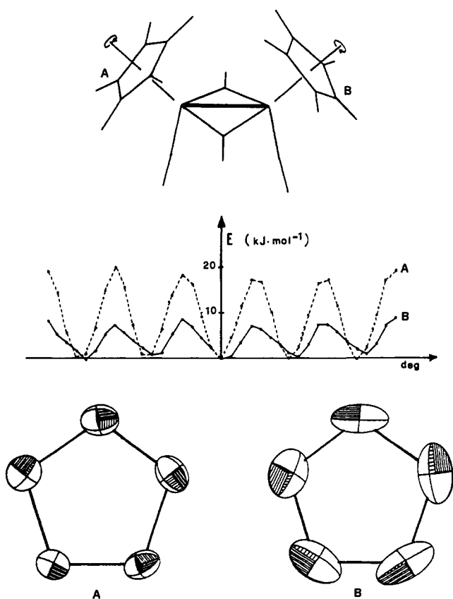
Figure 11. Ring reorientation in crystalline cis -(η 5 -C 5 H 5 ) 2 Fe 2 -(μ-CO) 2 (CO) 2 . Relationship between the reorientational barriers obtained by AAPEB calculations and the C-atom ADP patterns for the two crystallographically independent cyclopentadienyl rings.
