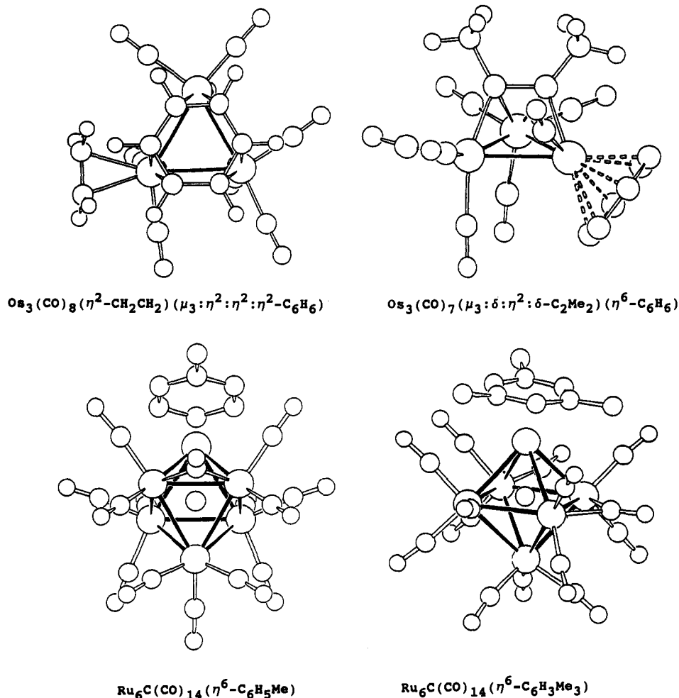
Figure 16. The molecular structures of some arene carbonyl clusters listed in Table IX (see also Figures 17 and 18).
