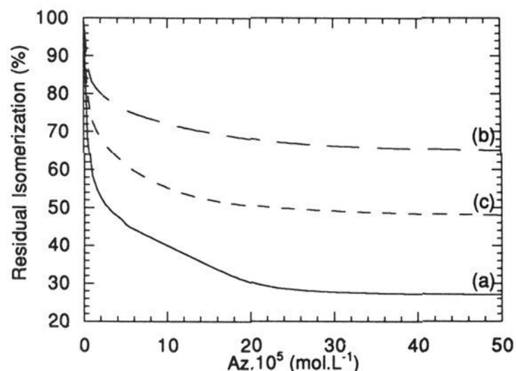
Figure 11. Different contribution of the “in-cage” [TP + CS •+ ] isomerization to the total yield as determined by Az quenching in homogeneous CH 2 Cl 2 solution using TPT (a), or heterogeneous conditions using TP + adsorbed within Y zeolite (TPY) (b), or extralarge pore zeolitic aluminosilicate (TPMCM-41) (c). (Adapted from refs 94 and 97.)
