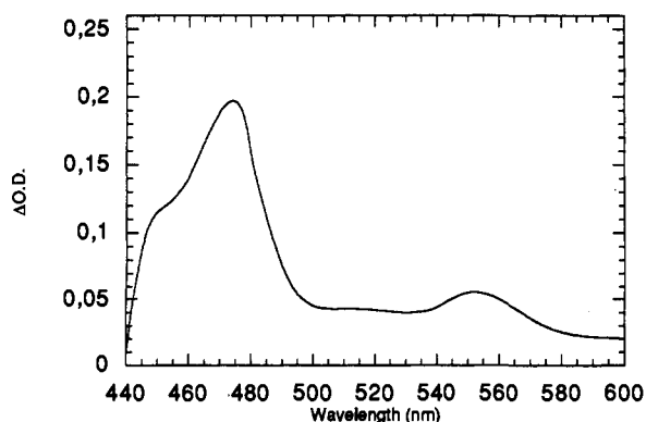
Figure 9. Transient absorption spectrum assigned to dimeric trans -stilbene radical cation obtained upon 408-nm excitation of a solution of TPT ( 6.2 \times 10^{-5} M) and trans -stilbene ( 4.3 \times 10^{-2} M) in \text{CH}_2\text{Cl}_2 . (Adapted from ref 71.)
