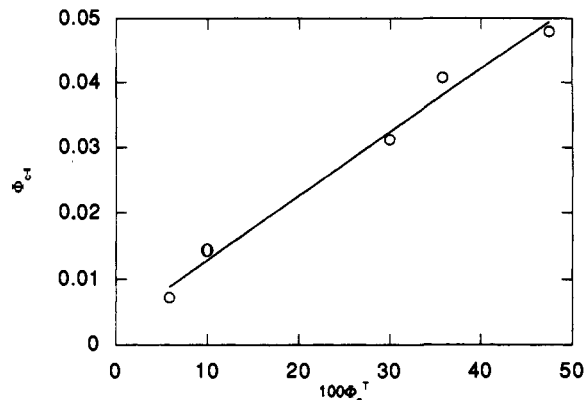
Figure 10. Plot of the quantum yield for the cis -stilbene isomerization ( \Phi_{c \rightarrow t} ) vs the quantum yield for the quenching of TPT triplet by CS ( \Phi_q^T ). The experimental points correspond to different CS concentrations in the range 9.4 \times 10^{-4} to 8.4 \times 10^{-2} M. (Adapted from ref 66.)
