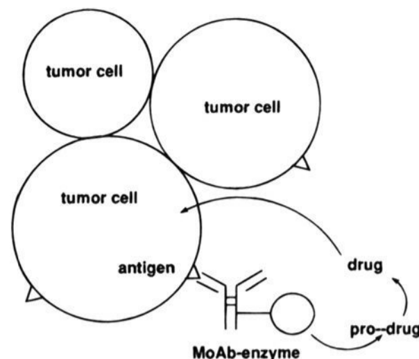
Figure 2. Antibody–directed catalysis.
