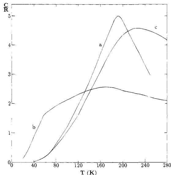
Figure 3. The rotational heat capacity of the ammonium ion in (a) \text{NH}_4\text{ReO}_4 , (b) (\text{NH}_4)_2\text{SnCl}_6 , and the borohydride ion in (c) \text{CsBH}_4 .
