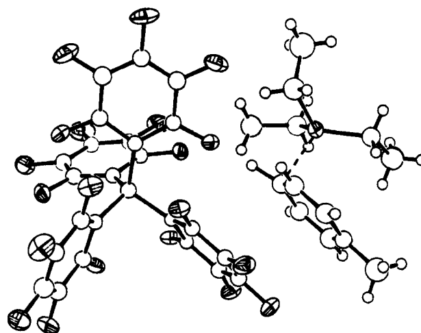
Figure 1. Molecular structure of triethylsilylium-toluene tetrakis(pentafluorophenyl)borate. Silylium cation, upper right; TFPFB anion, left; toluene, lower right. (Reprinted with changes from ref 44. Copyright 1993 American Association for the Advancement of Science.)
