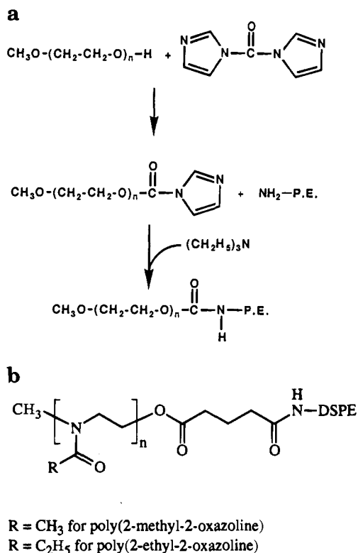
Figure 4. (a) Chemical formula and chemical synthesis scheme for the methoxy polyoxyethylene carbamate derivative of phosphatidylethanolamine and (b) structural formula for poly(2-acyl-2-oxazoline).
