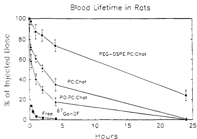
Figure 3. Blood clearance rates of different liposome preparations as measured by the radioactive tracers. For details see ref 20.
