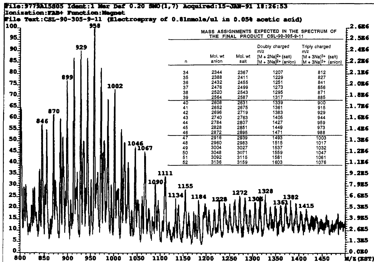
Figure 5. Mass spectra of methoxy PEG 2000 Da (a) and, after its coupling to DSPE, of 2000 PEG-DSPE (b). Spectra were recorded on VG Tribid (EBEEQQ geometry) at sample flow rate 4 \mu L/mL (curtain gas 0.3L/min at 100 ^{\circ} C) and voltages at interface plate, nozzle, and needle were 3.17, 3.13, and 8.9 kV, respectively. At accelerating voltage 2.9 kV mass range m/z = 800 to m/z = 1500 were scanned (* s/scan, signal averaged for 20 min). Spectra as well as tabulated mass assignments, as expected from the spectra of both compounds, show that chemical reaction only shifts molecular weight for 772 Da. (Courtesy of J. Guthrie and S. Greenwald.)
