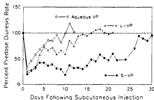
Figure 23. Antidiuretic effect of peptide vasopressin at 50 \mu\text{g}/\text{rat} , administered as free drug (○), in conventional liposomes (Δ), or in Stealth liposomes (■). For details see ref 157.
