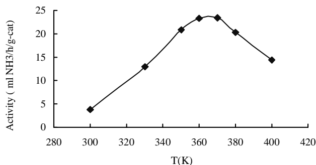
Figure 1 Ammonia synthesis activity of Ru-K/carbon nanotubes
