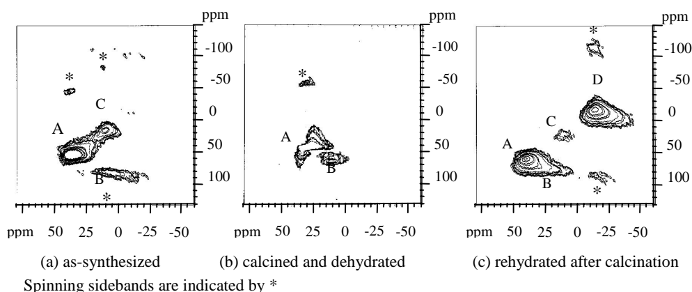
Figure 2 ^{27}\text{Al} 3Q MAS NMR spectra of SAPO-34
