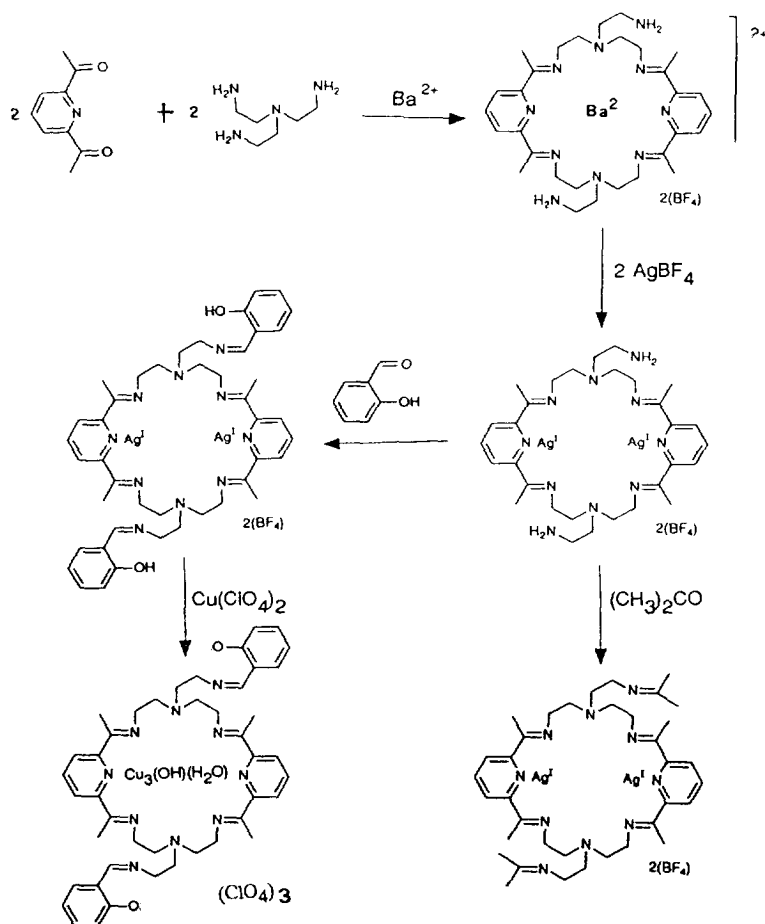
Scheme 36. Reaction pathway for the formation of mononuclear, homodinuclear and homotrinnuclear complexes.
