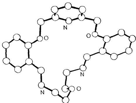
Fig. 38. Structure of 59 .
