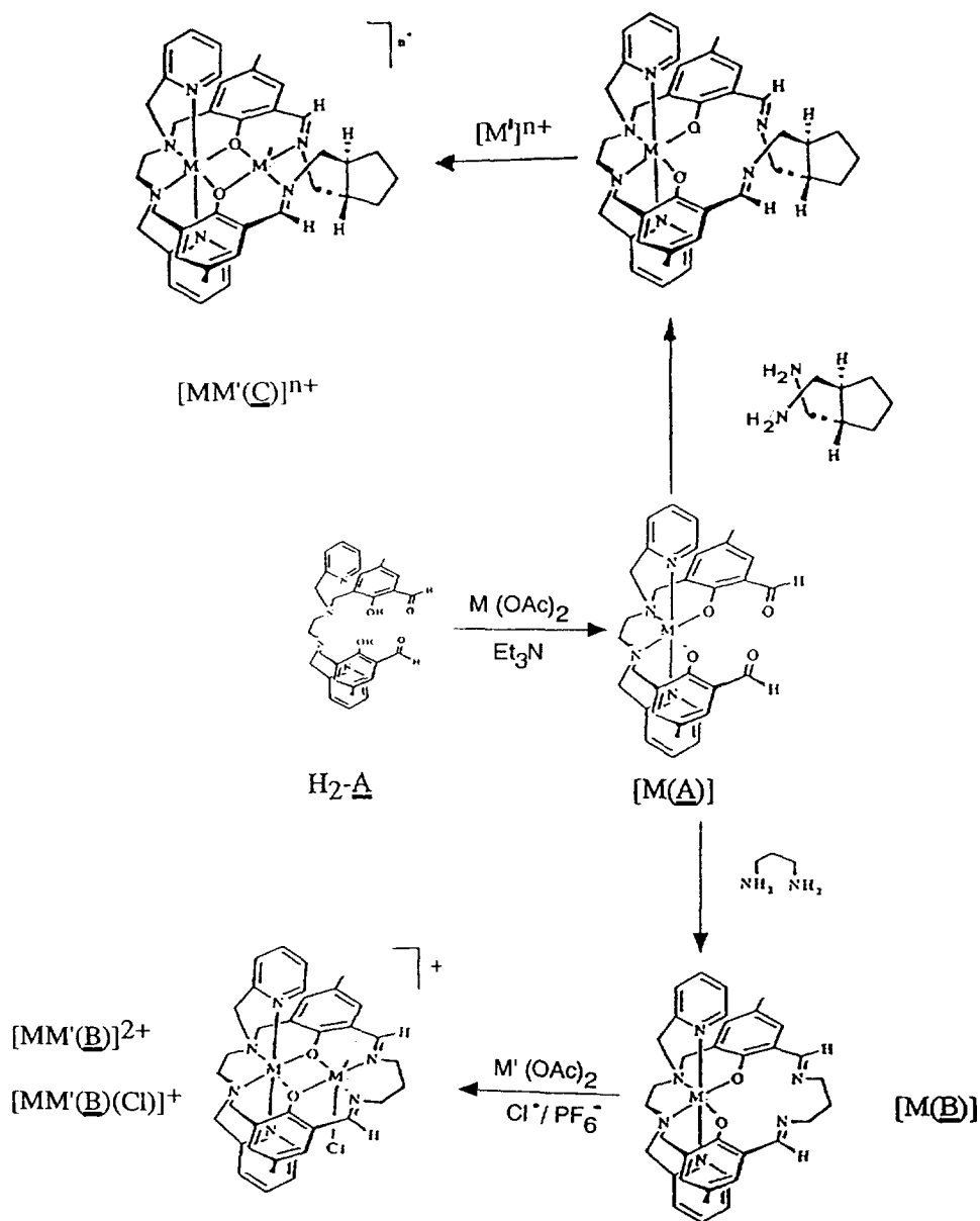
Scheme 34. Mononuclear, homo- and heterodinuclear complexes prepared from a macrocyclic compartmental ligand containing a six- and a four-coordinate site.
