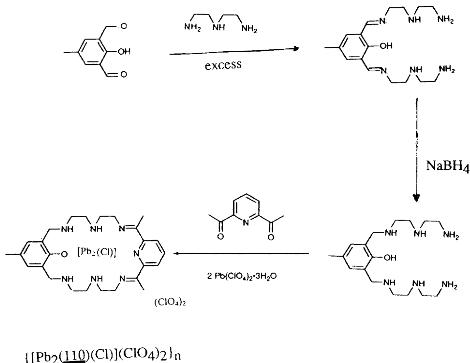
Scheme 38.
