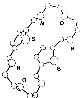
Fig. 11. Structure of 27 .
