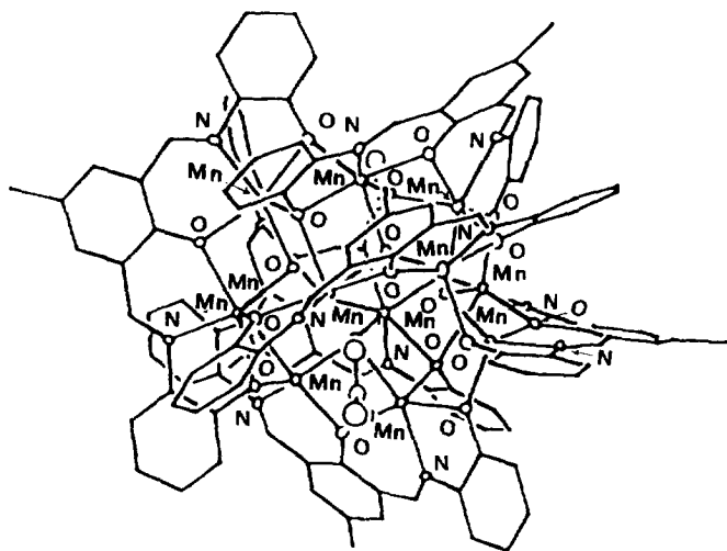
Fig. 92. View of the dodecanuclear aggregate [(\text{Mn})_{12}(\mathbf{116})_6(\text{OH})_4(\text{CH}_3\text{COO}_2)_2] .
