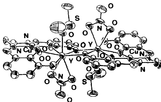
Fig. 69. Structure of [\text{CuY}(\mathbf{81})(\text{NO}_3)_3(\text{dmsO})]_2 .
