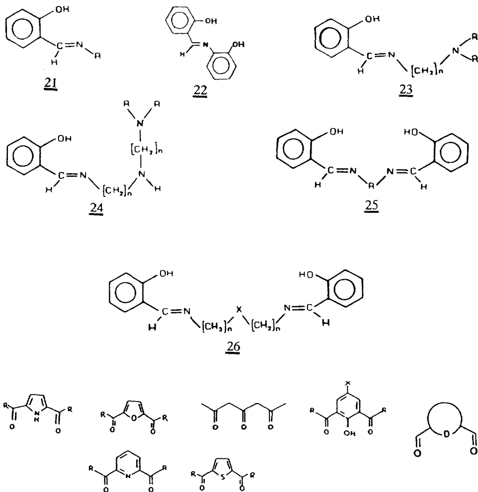
Scheme 4.
