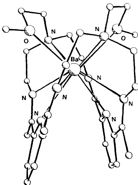
Fig. 18. Structure of [Ba(37)] 2+ .
