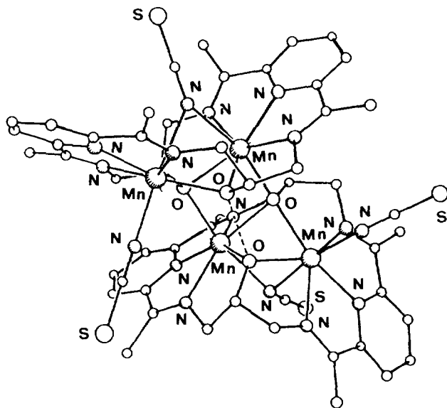
Fig. 105. Structure of [\text{Mn}_4(\mathbf{45-2H})(\mathbf{45-H})(\text{NCS})_4]^+ .
