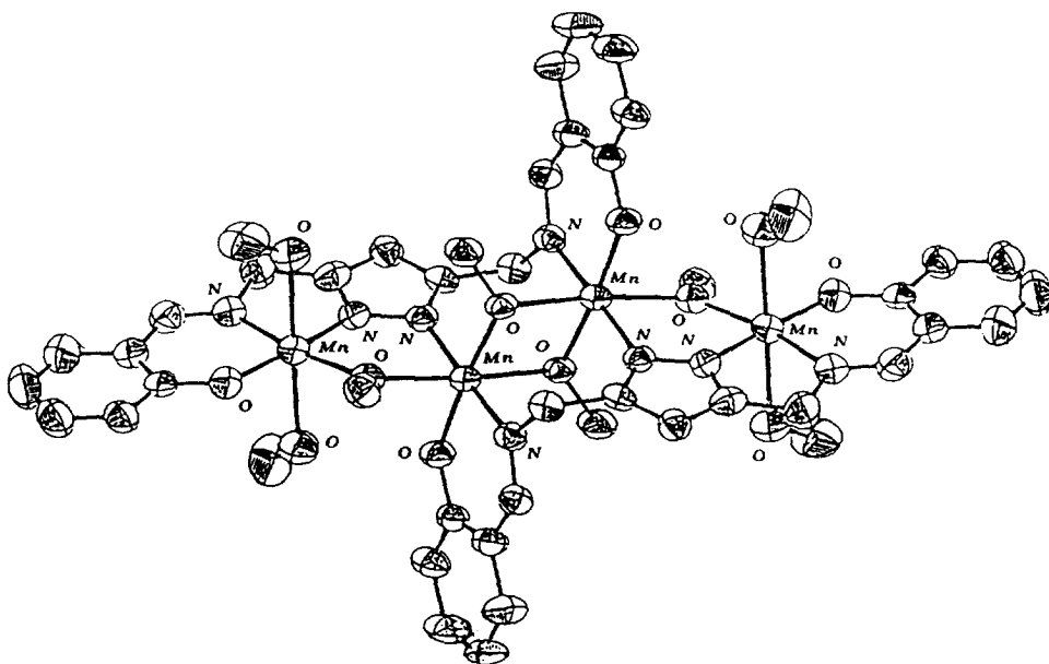
Fig. 96. Structure of [(Mn 4 (121) 2 (CH 3 O) 4 (CH 3 OH) 4 ] 2- .
