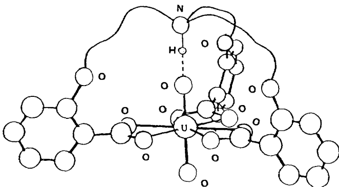
Fig. 56. Schematic diagram of a stereognostic ligand for \text{UO}_2^{2+} incorporating three donor carboxylate groups and an ammonium hydrogen bond donor.
