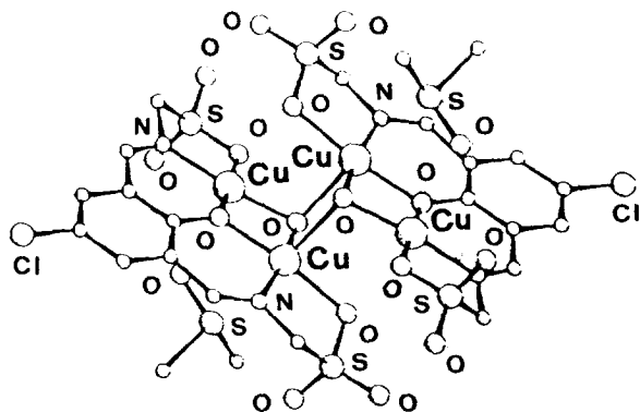
Fig. 93. Structure of [\text{Cu}_2(\mathbf{117})(\text{OH})(\text{dmsO})(\text{H}_2\text{O})]_2 .
