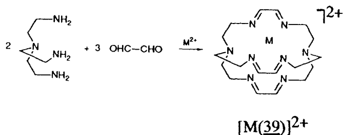
Scheme 11.
