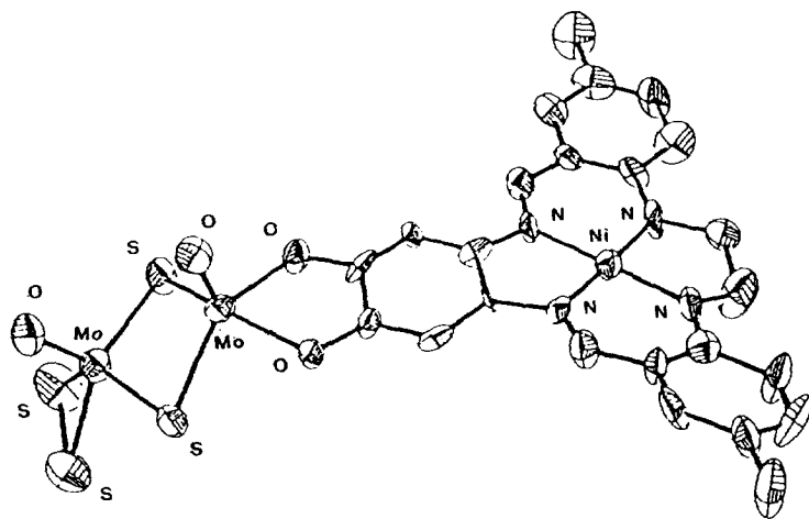
Fig. 129. Structure of \{[Ni(\text{macro})]_2[Mo_2O_2S_2]\}^{2+} .
