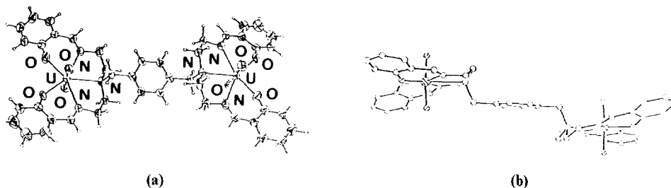
Fig. 124. (a) The molecular structure and (b) the three step conformation of the complex (\text{UO}_2)_2(\text{143}) .
