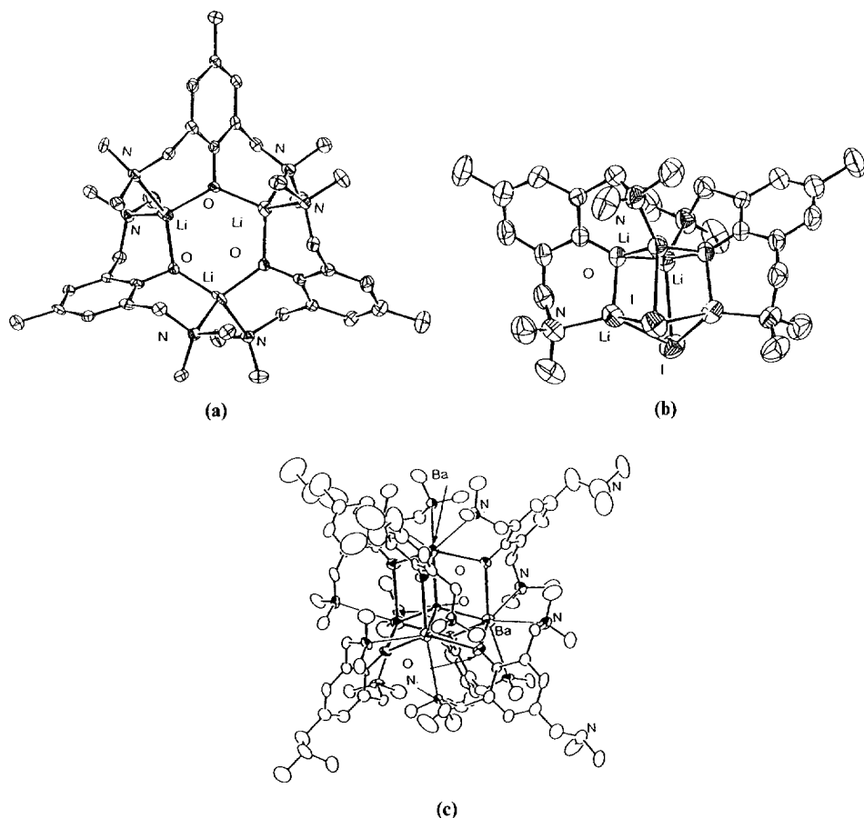
Fig. 101. Structures of (a) [\text{Li}(\mathbf{123}')_3]_3 , (b) [\text{Li}_4(\mathbf{123}')_2(\text{I})_2] and (c) [\text{Ba}_4(\mathbf{123}')(\mu_4\text{-O})_6] \cdot 3 toluene.
