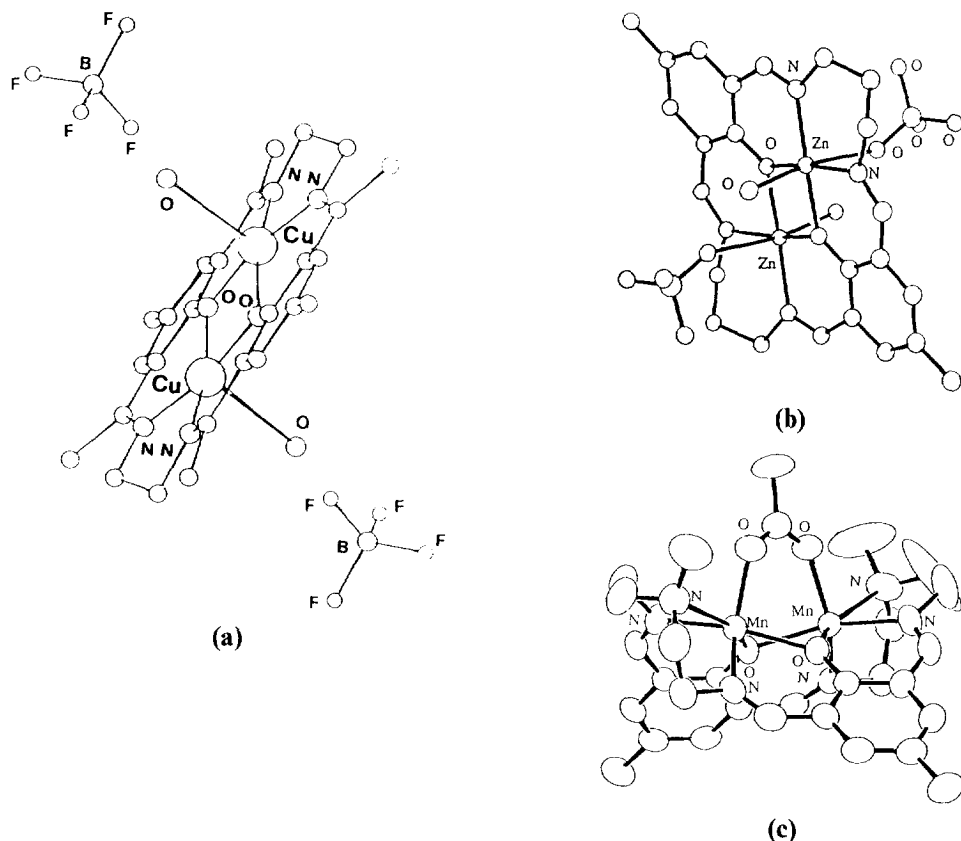
Fig. 58. Structures of (a) [\text{Cu}_2(\mathbf{75})(\text{H}_2\text{O})_2](\text{BF}_4)_2 , (b) [\text{Zn}_2(\mathbf{75}')(\text{H}_2\text{O})_2(\text{ClO}_4)_2] and (c) [\text{Mn}_2(\mathbf{75}'')(\text{CH}_3\text{COO})]^+ .
