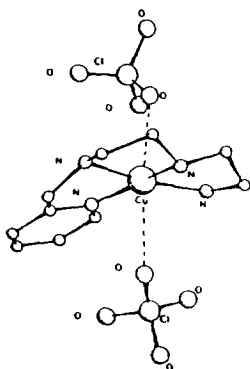
Fig. 34. Structure of [\text{Cu(52)(ClO}_4)_2] .
