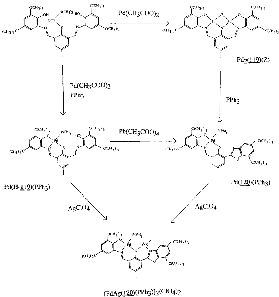
Scheme 39.
