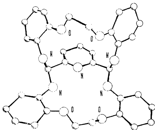
Fig. 14. Structure of 32.
