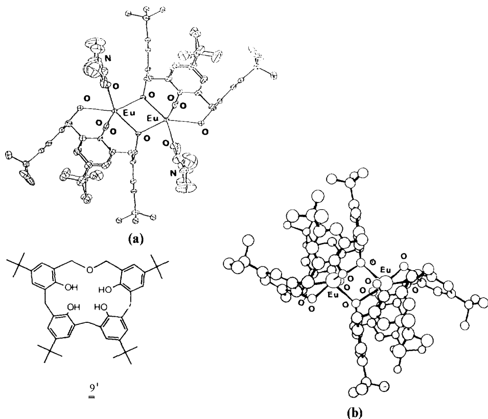
Fig. 10. Structures of (a) \text{Eu}_2(9\text{-}3H)_2(\text{dmf})_4 and (b) [\text{Eu}_2(9'\text{-}3H)(\text{dmsO})_2] \cdot 2\text{acetone} .
