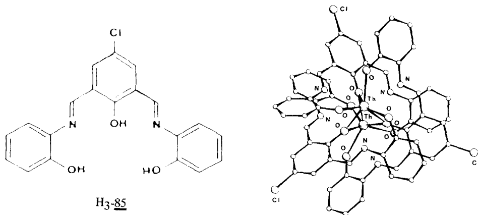
Fig. 66. Structure of [\text{Th}_2(\mathbf{85})_3]_2^{2-} .
