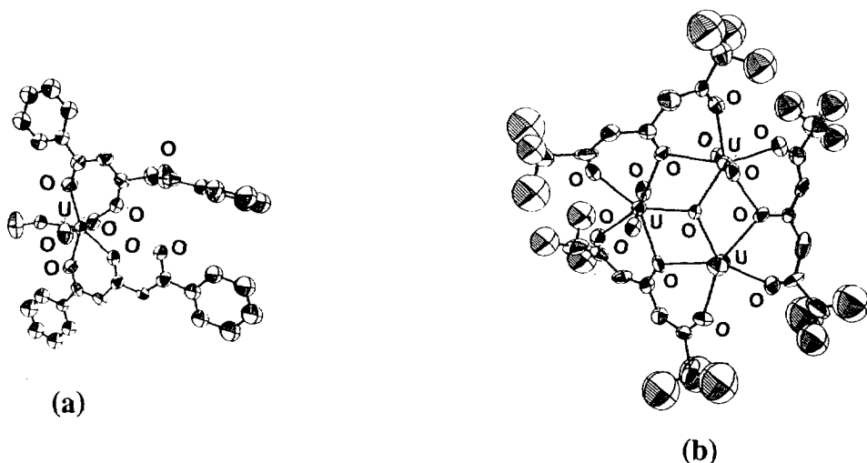
Fig. 86. (a) The molecular structure of bis[1,5-diphenyl-1,3,5-pentanetrionato](methanol)bisdioxo-uranium(VI) (b) The trinuclear structure of the anion of the complex bis(triethylammonium)-tris(2,2',8,8'-tetramethyl-3,5,7-nonanetrionato)- \mu_3 -oxo-tris(dioxouranate).
