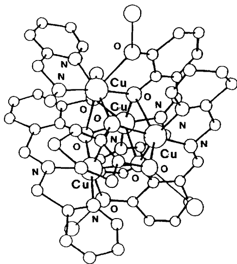
Fig. 90. Structure of [\text{Cu}(\text{H-113})(\text{NO}_3)_4]_4 .
