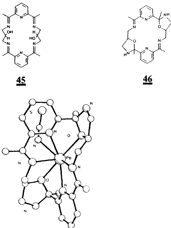
Fig. 30. Structure of [\text{Pb}(\mathbf{46})(\text{NCS})]^+ .
