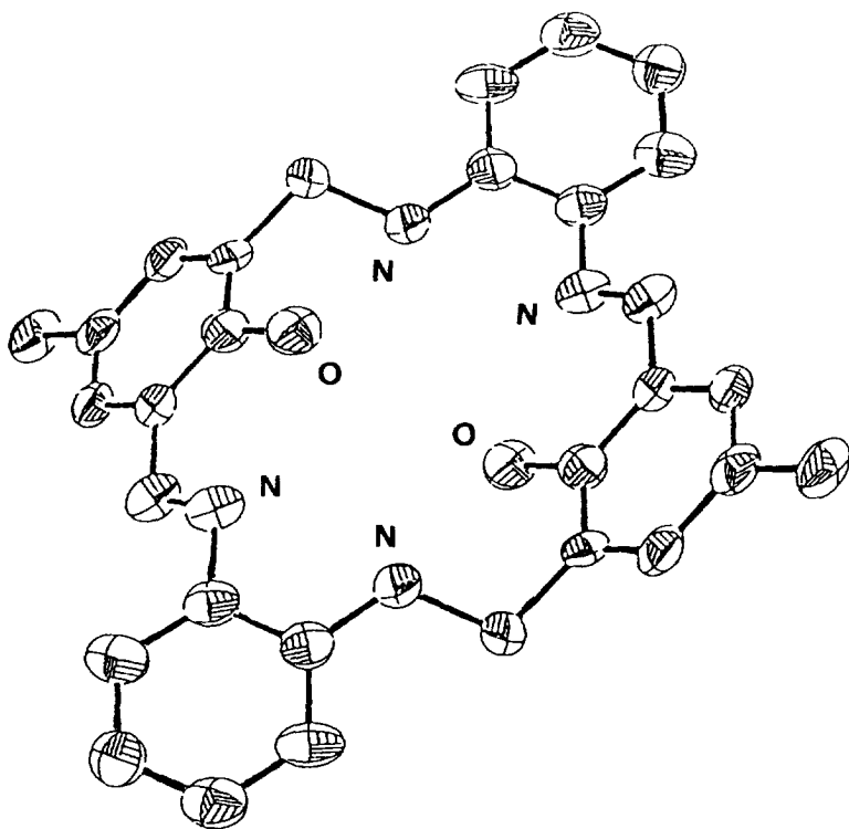
Fig. 13. Structure of 29 .
