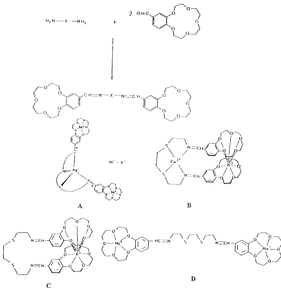
Scheme 54.
