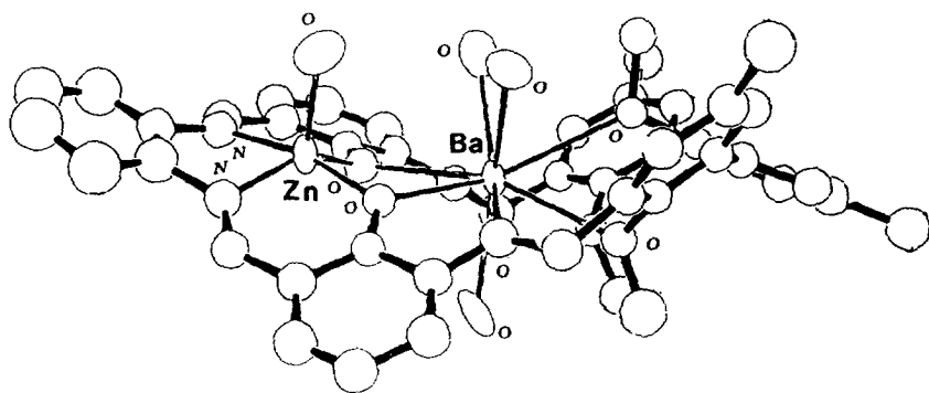
Fig. 75. Structure of \text{ZnBa}(\mathbf{100})(\text{CF}_3\text{SO}_3)_2 \cdot 3\text{dmf} (only the coordinated oxygen atoms of the three dimethylformamide molecules and of the coordinated anion are shown for clarity).
