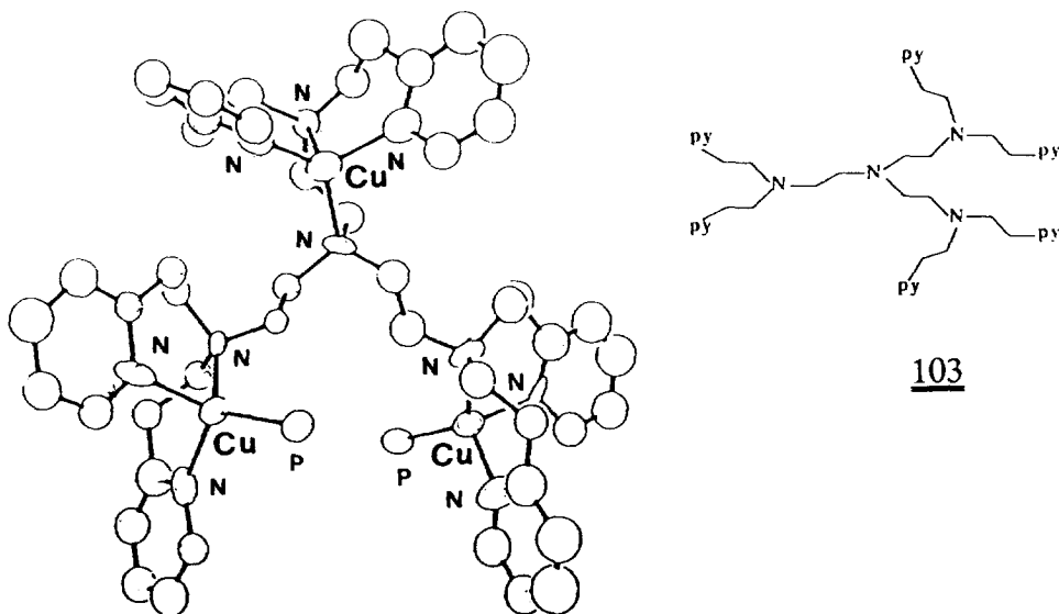
Fig. 77. Structure of [\text{Cu}_3(\mathbf{103})(\text{PPh}_3)_2]^{3+} .
