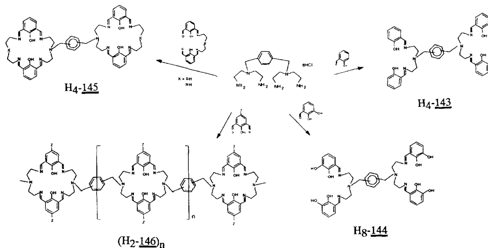
Scheme 48.
