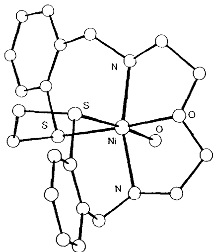
Fig. 44. Structure of [\text{Ni}(\mathbf{62f})(\text{H}_2\text{O})]^{2+} .
