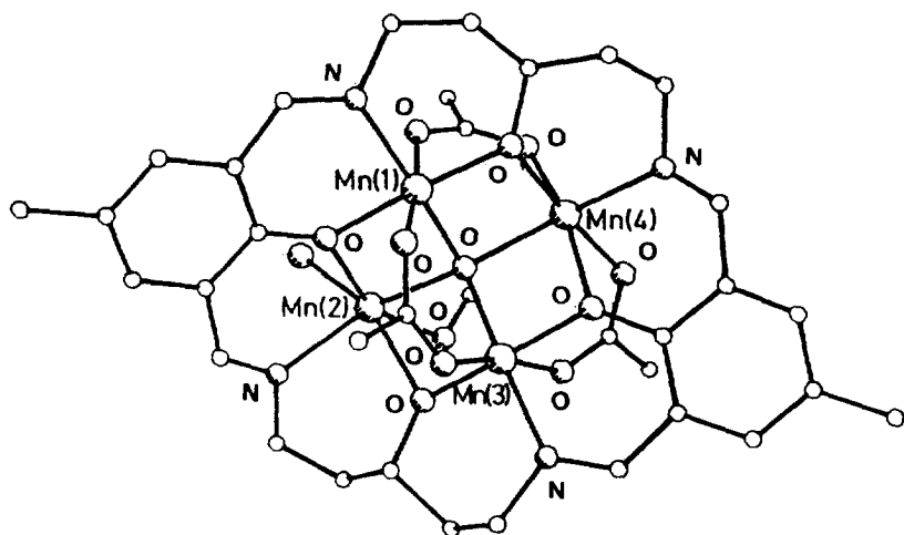
Fig. 111. Structure of [\text{Mn}^{\text{II}}_2\text{Mn}^{\text{II}}_2(128)(\text{O})(\text{CH}_3\text{COO})_3(\text{Cl})(\text{MeOH})] .
