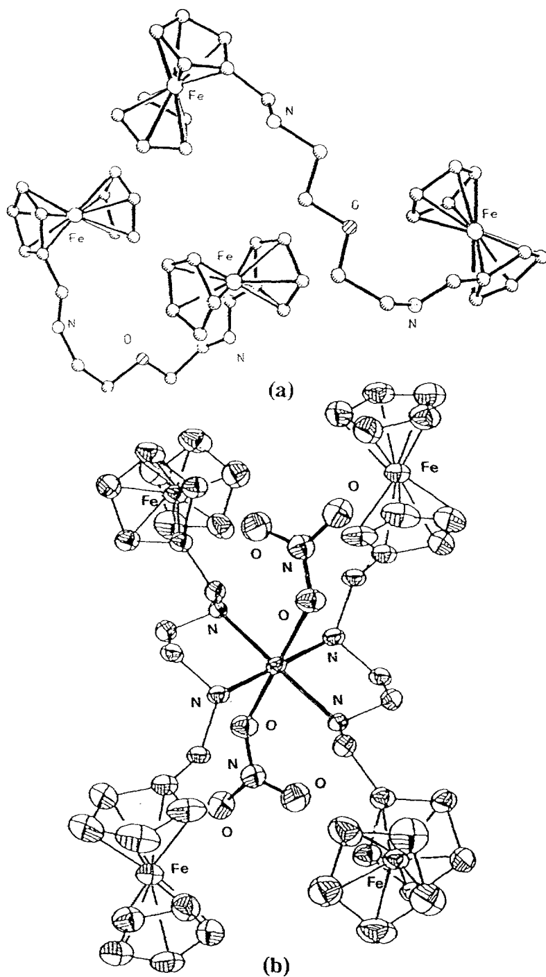
Fig. 125. Structures of (a) diferrocenyl Schiff base reported in Scheme 52 ( R \equiv -(\text{CH}_2)_2\text{O}(\text{CH}_2)_2- ) and (b) bis( N,N' -ethylene bis[(ferrocenylmethyl)amine]);copper(II) dinitrate.
