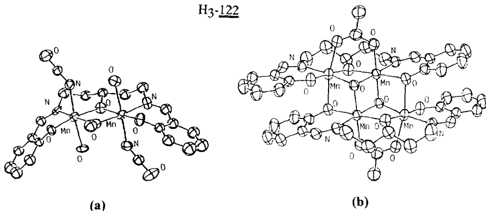
Fig. 97. Structures of (a) [\text{Mn}_2(\mathbf{122})(\text{CH}_3\text{O})(\text{NCO})_2(\text{H}_2\text{O})_2] and (b) [\text{Mn}_4(\mathbf{122})_2(\text{O})_2(\text{CH}_3\text{COO})_2] .
