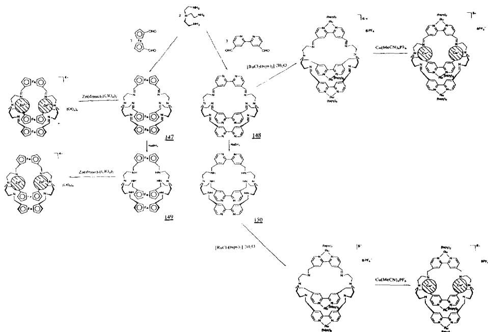
Scheme 51.
