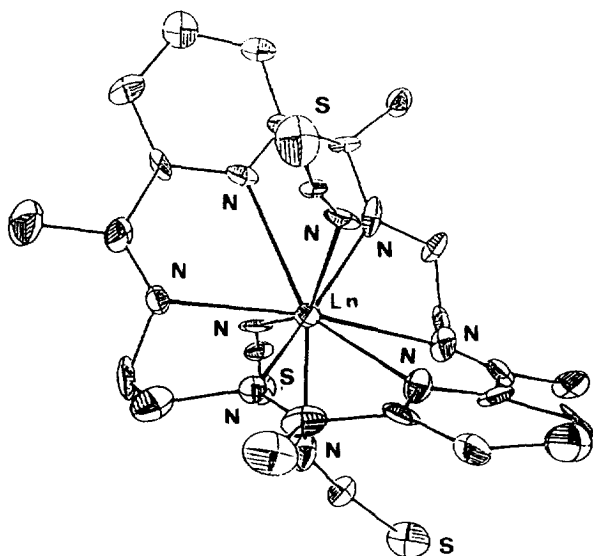
Fig. 54. Structure of [\text{Ln}(\mathbf{38})(\text{NCS})_3] ( \text{Ln} \equiv \text{Y}(\text{III}), \text{Eu}(\text{III}) ).
