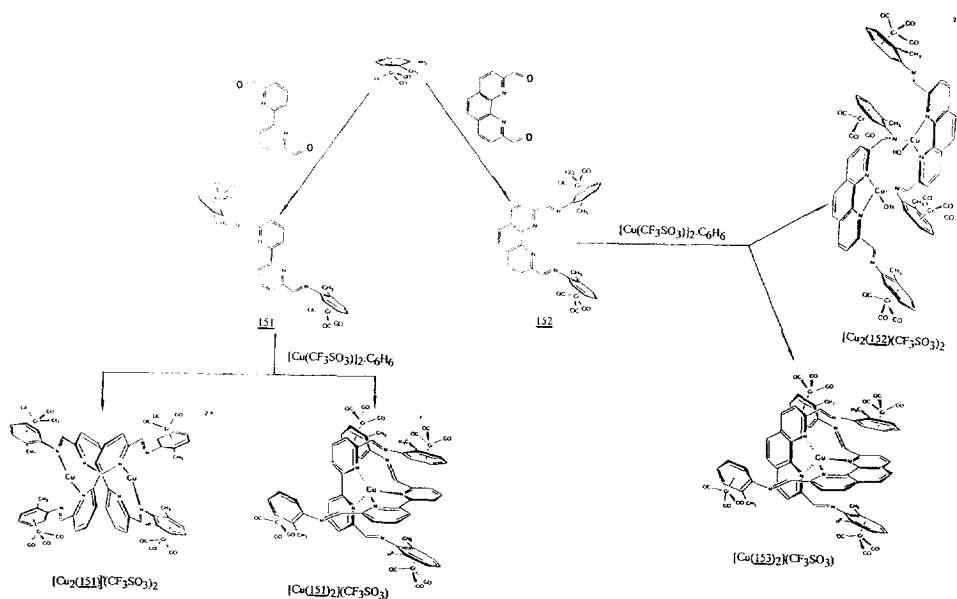
Scheme 56.
