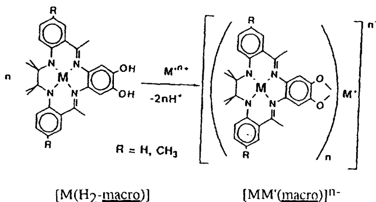
Scheme 59.
