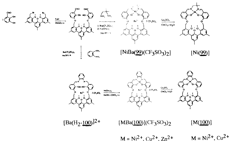
Scheme 33.
