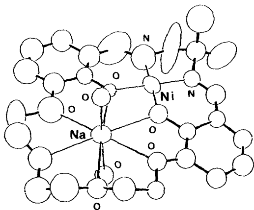
Fig. 74. View of \text{NaNi}(\mathbf{98})(\text{picrate}) (only the coordinated oxygen atoms of the two picrate anions are shown for clarity).
