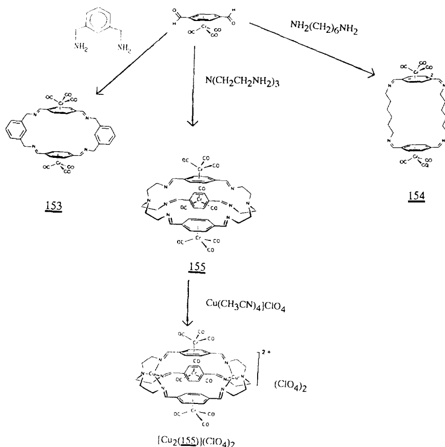
Scheme 57.
