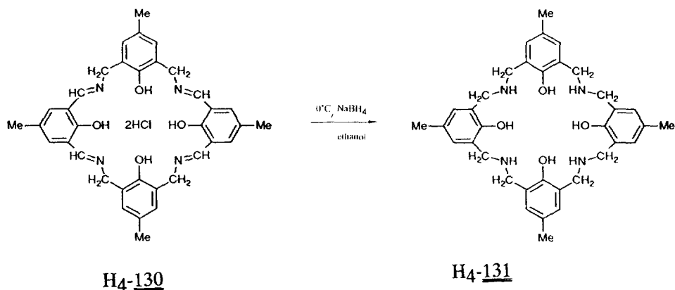
Scheme 42.
