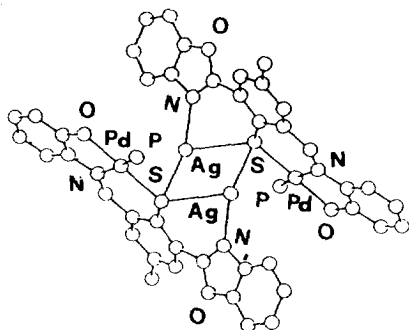
Fig. 95. Structure of [PdAg(120)(PPh 3 )] 2 2+ .
