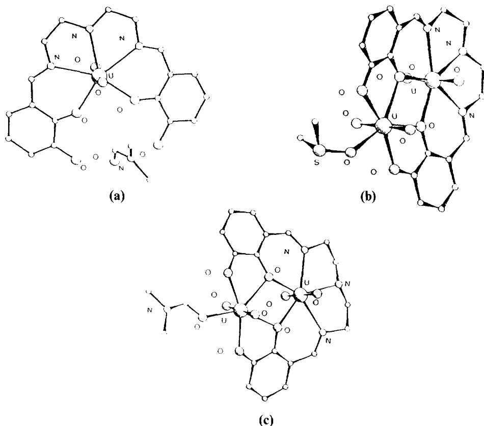
Fig. 71. Structures of (a) \text{UO}_2(\text{H}_2\text{-94}) , (b) (\text{UO}_2)_2(\text{94})(\text{dmsO}) and (c) (\text{UO}_2)_2(\text{94})(\text{dmf}) .
