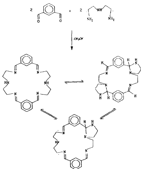
Scheme 15.
