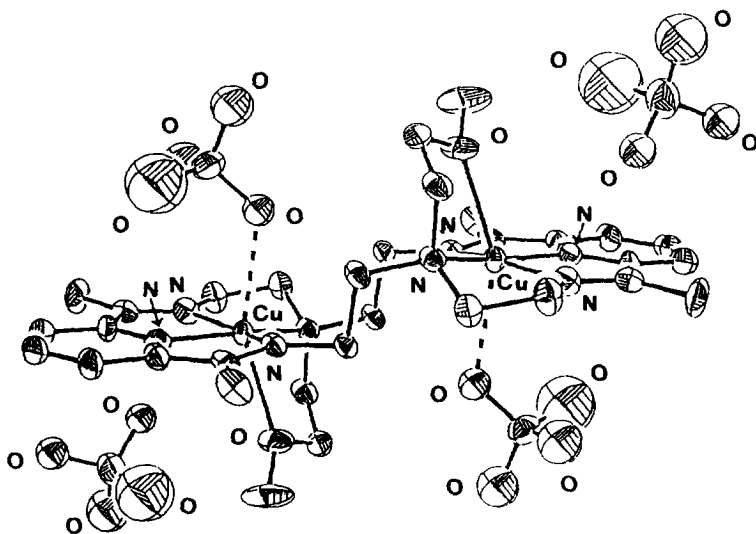
Fig. 21. Structure of [\text{Cu}_2(\mathbf{37})](\text{ClO}_4)_4 .
