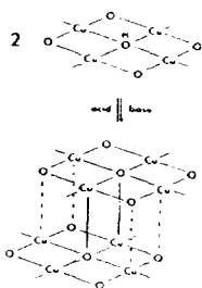
Scheme 43.
