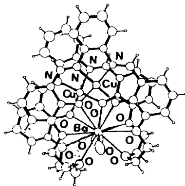
Fig. 81. Structure of \text{Cu}_2\text{Ba}(\text{108})(\text{CF}_3\text{SO}_3)_2 \cdot 2\text{H}_2\text{O} .
