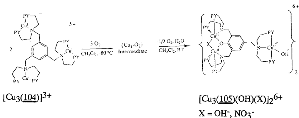
Scheme 35.
