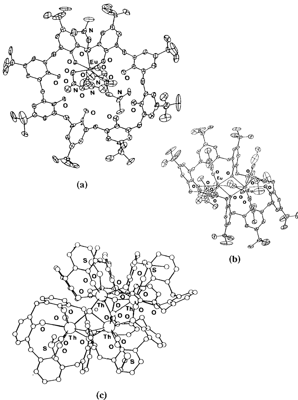
Fig. 9. Structures of (a) \text{Eu}(\mathbf{13-2H})(\text{NO}_3)\text{dmf}_4 , (b) [\text{Eu}_2(\mathbf{13-6H})(\text{dmf})_5] and (c) [\text{Th}_4(\mathbf{13-7H})(\mathbf{13-6H})(\text{dmsol})_4(\text{OH})_3(\text{OH})_2] .
