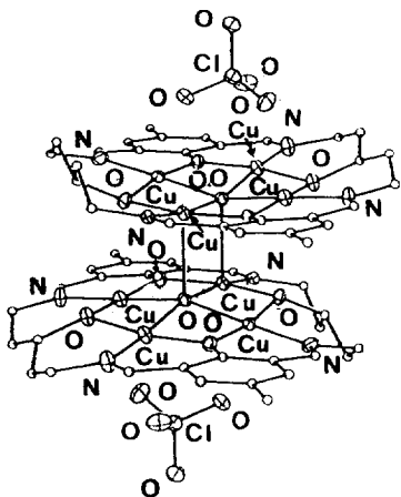
Fig. 116. Perspective view of [\text{Cu}_4(\mathbf{128})(\mu_5\text{-O})(\text{ClO}_4)_2]^{2+} .
