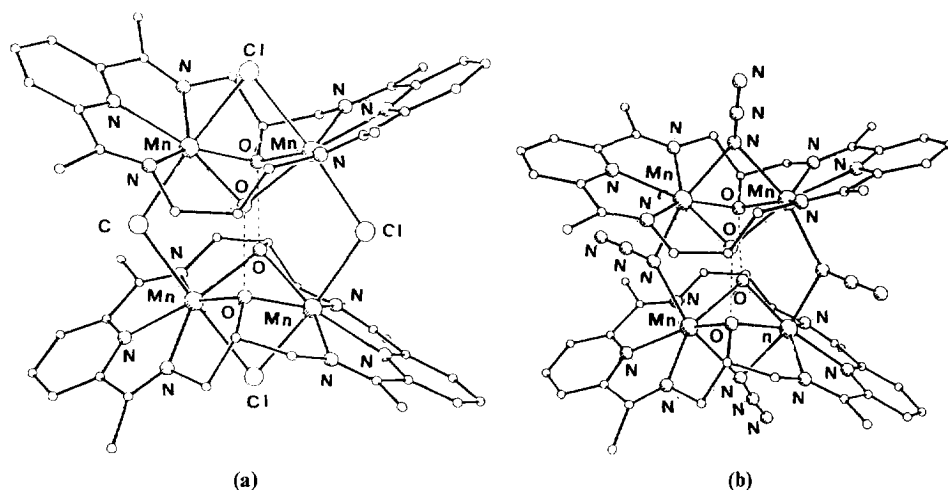
Fig. 104. Structures of (a) [\text{Mn}_2(\mathbf{45-H})(\text{Cl})_2]_2^{2+} and (b) [\text{Mn}_2(\mathbf{45-H})(\text{N}_3)_2]_2^{2+} .
