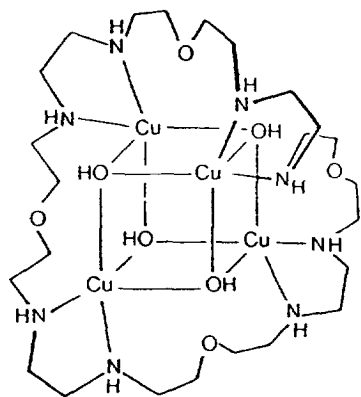
Fig. 133. Probable structure of [\text{Cu}_4(\mathbf{160})(\text{OH})_4]^{4+} .
