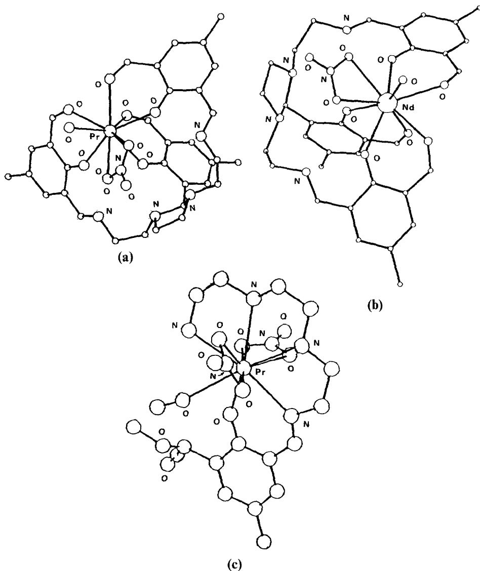
Fig. 68. Structures of (a) [\text{Pr}(\text{H}_3\text{-89})(\text{NO}_3)(\text{OH})_2]^{2-} , (b) [\text{Nd}(\text{H}_3\text{-89})(\text{NO}_3)(\text{OH})_2][\text{NO}_3]_2 and (c) \text{Pr}(\text{89}')(\text{NO}_3)_2 \cdot \text{CH}_3\text{OH} .
