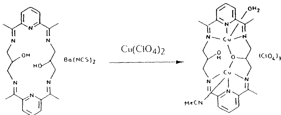
Scheme 40.
