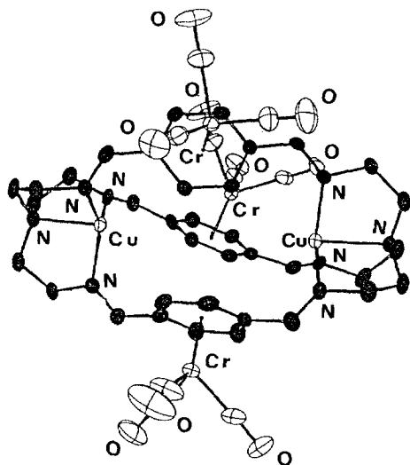
Fig. 128. Structure of [\text{Cu}_2(\mathbf{155})]^{2+} .
