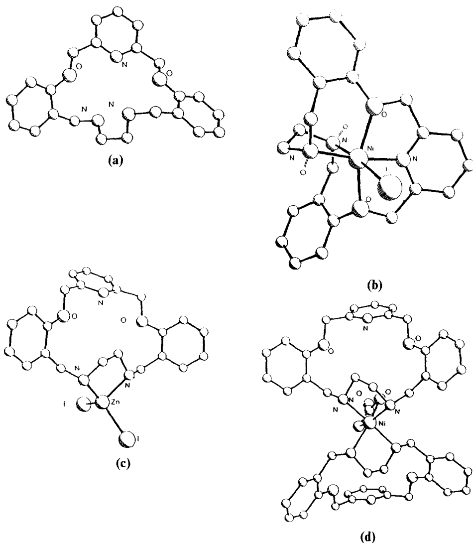
Fig. 39. Structures of (a) 61a , (b) [\text{Ni}(\mathbf{61a})(\text{I})]^+ as an example of 1:1 complex with the metal inside the macrocycle, (c) [\text{Zn}(\mathbf{61a})(\text{I})_2] as an example of 1:1 complex with the metal ion coordinated exocyclically and of (d) the complex [\text{Ni}(\mathbf{61a})_2(\text{NO}_3)] \cdot (\text{NO}_3) with the metal ion coordinated exocyclically.
