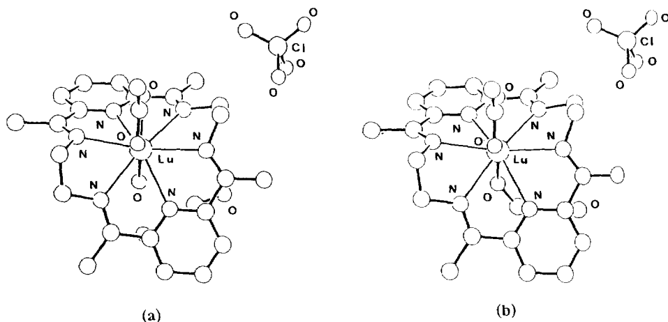
Fig. 52. Perspective views of (a) [\text{Lu}(\mathbf{38})(\text{CH}_3\text{COO})(\text{H}_2\text{O})](\text{CH}_3\text{OH})(\text{OH})(\text{ClO}_4) and (b) [\text{Lu}(\mathbf{38})(\text{CH}_3\text{COO})(\text{CH}_3\text{OH})](\text{OH})(\text{ClO}_4) .
