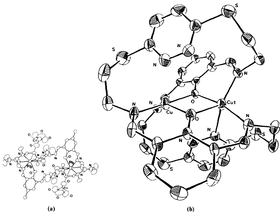
Fig. 118. Structures of (a) [\text{Pb}_2(\text{H}_2\text{-86}'')(\text{dmf})_4(\text{ClO}_4)_2]^{2+} and (b) [\text{Cu}_2(86''')]^{2-} .
