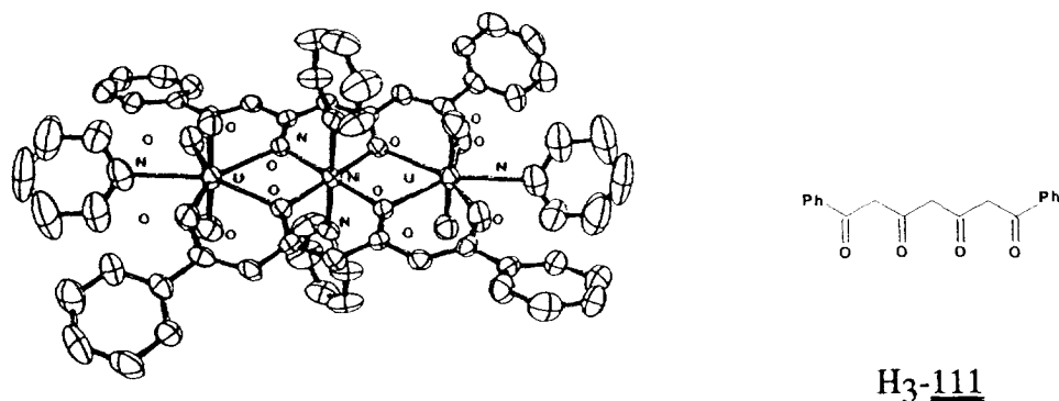
Fig. 87. Structure of [(\text{UO}_2)_2\text{M}(\mathbf{111})_2(\text{py})_4] ( \text{M} \equiv \text{Zn}^{2+}, \text{Cu}^{2+}, \text{Ni}^{2+}, \text{Co}^{2+}, \text{Fe}^{2+}, \text{Mn}^{2+} ).
