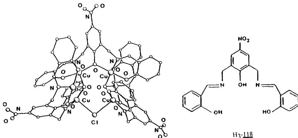
Fig. 94. Structure of \{[Cu_3(118)(dmf)]_2(\mu-Cl)(\mu-118)\} .
