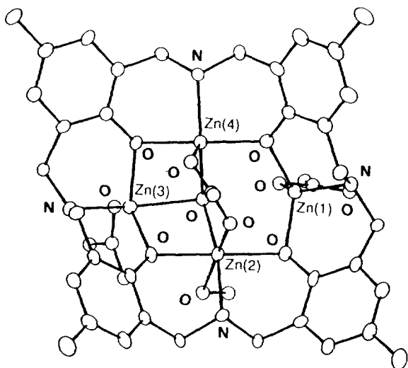
Fig. 114. The structure of \text{Zn}_4(\mathbf{131})(\text{OH})(\text{CH}_3\text{COO})_3 .
