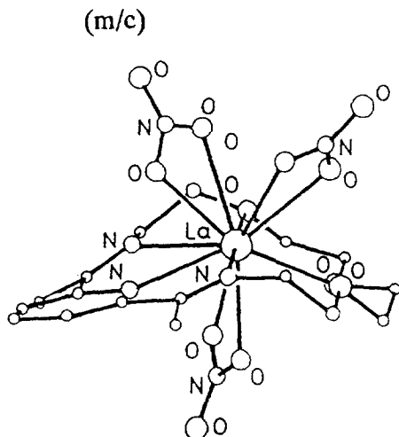
Fig. 55. Structure of [La(72a)](NO_3)_3 .
