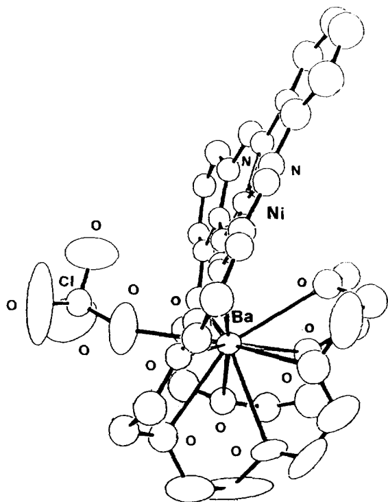
Fig. 72. Structure of NiBa(97)(ClO 4 ) 2 · MeOH.
