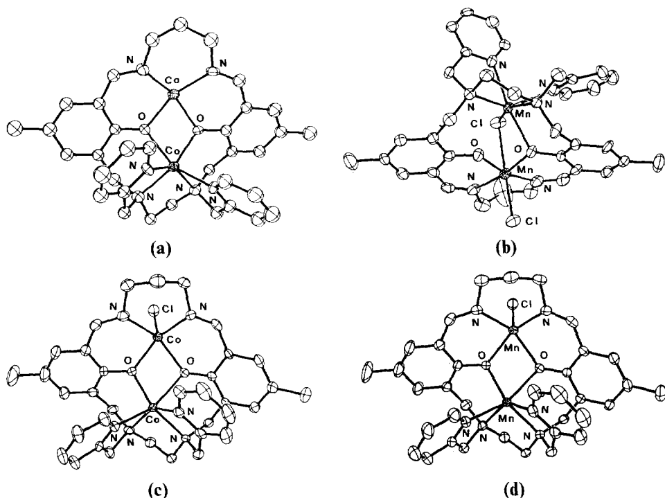
Fig. 76. Structures of (a) [\text{Co}_2(\mathbf{B})](\text{PF}_6)_2 , (b) [\text{Mn}_2(\mathbf{B})(\mu\text{-Cl})(\text{Cl})]\text{PF}_6 , (c) [\text{Co}_2(\mathbf{B})(\text{Cl})]\text{PF}_6 and (d) [\text{Mn}_2(\mathbf{B})(\text{Cl})]\text{PF}_6 ( \text{H}_2\text{-B} is the macrocycle reported in Scheme 34).
