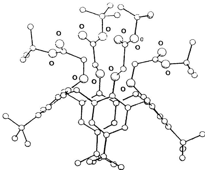
Fig. 5. Structure of 11 .
