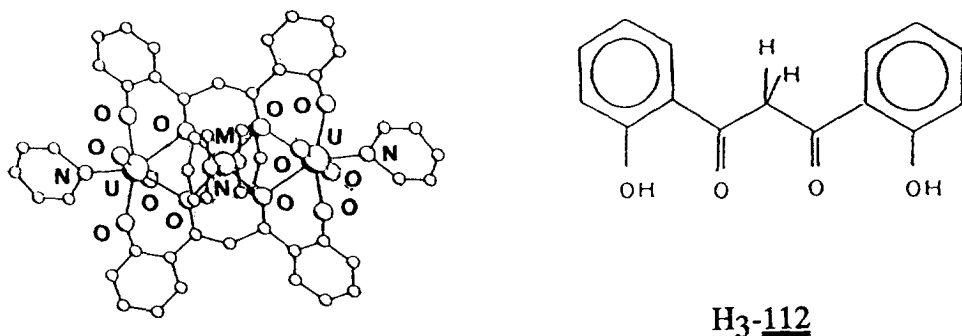
Fig. 88. Perspective view of [(\text{UO}_2)_2\text{M}(\underline{112})_2(\text{py})_4] \cdot 2\text{py} ( \text{M} \equiv \text{Co}, \text{Ni} ).
