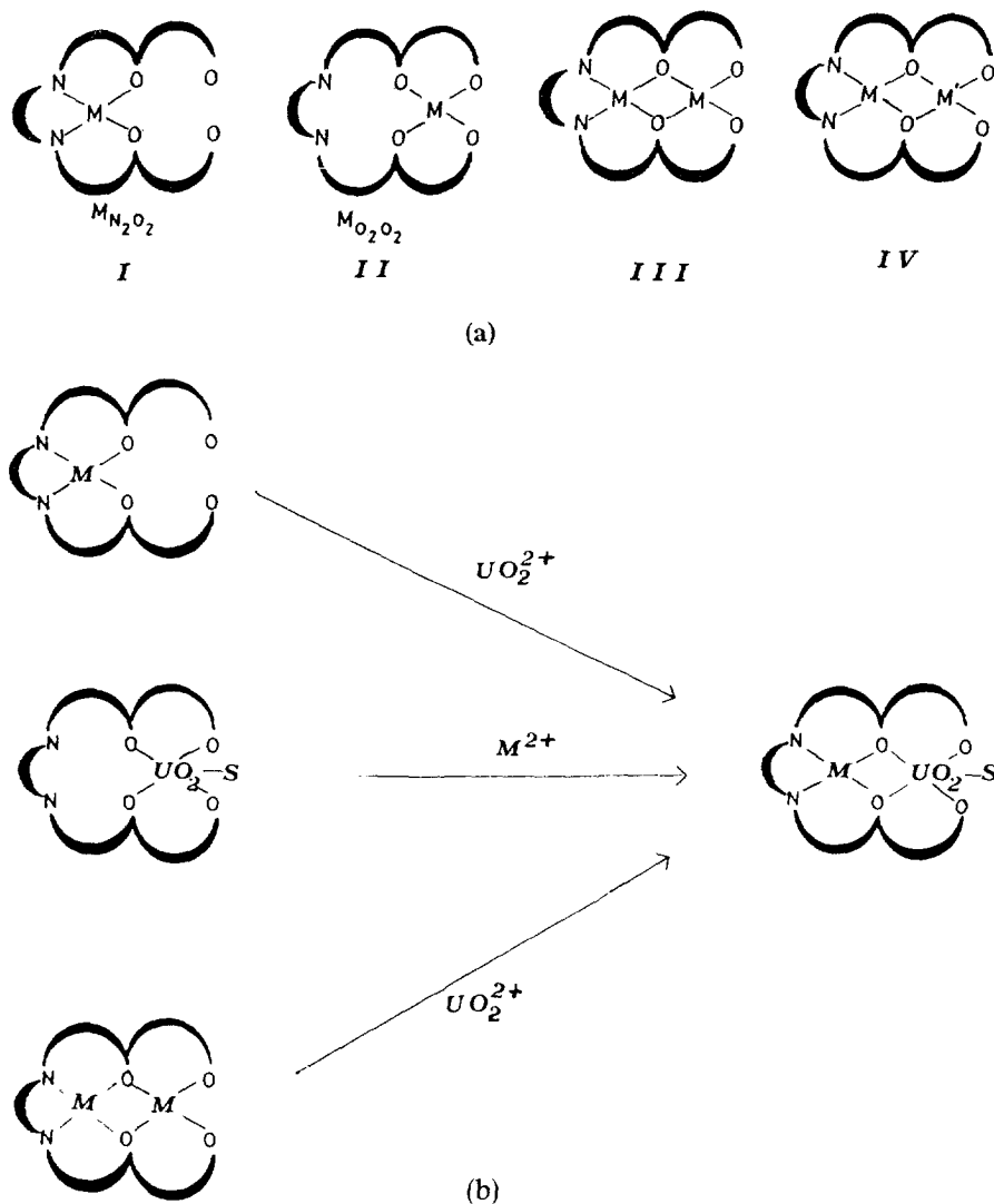
Scheme 28. (a) Schematic representation of mononuclear (I and II) and heterodinuclear (III and IV) positional isomers. (b) The possible pathways for the formation of heterodinuclear complexes containing \text{UO}_2^{2+} .
