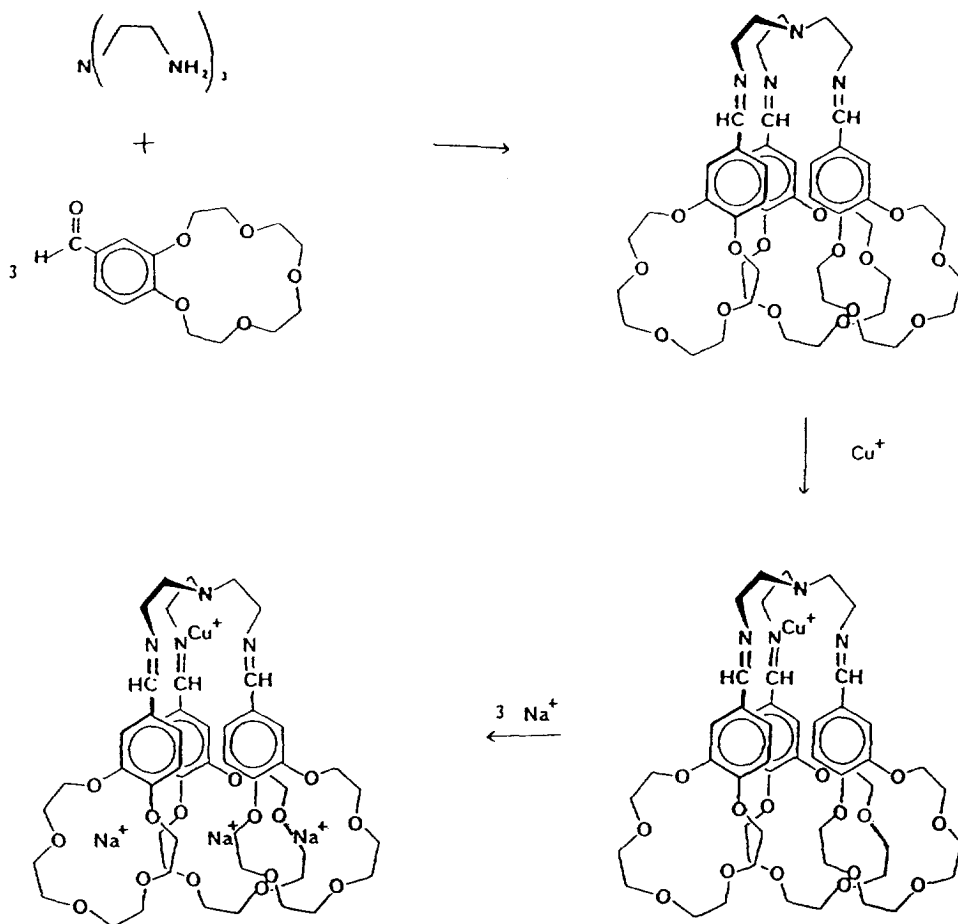
Scheme 55.
