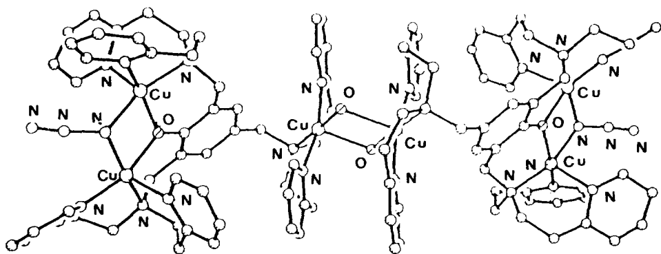
Fig. 78. Perspective view of \{[\text{Cu}_3(\text{105})(\text{N}_3)(\text{OH})]\}_2^{6+} .
