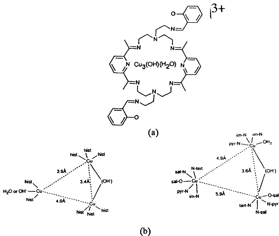
Scheme 2. (a) The trinuclear copper complex with a functionalized hexaimine Schiff base and (b) structure resemblance between this trinuclear copper and the triangulo -Cu 3 site in ascorbate oxidase.
