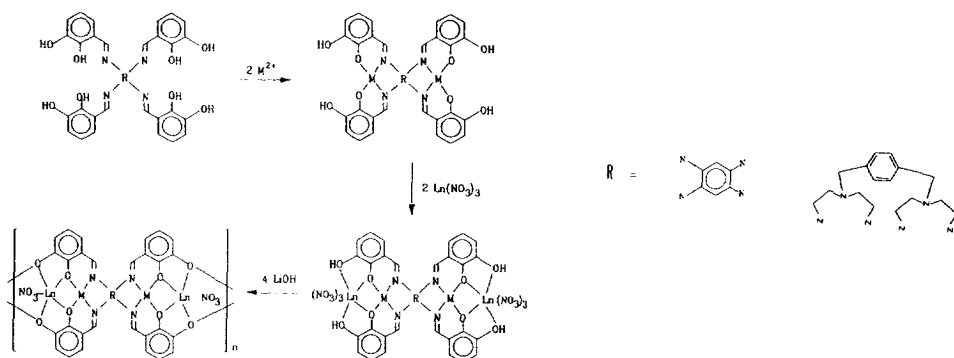
Scheme 50.
