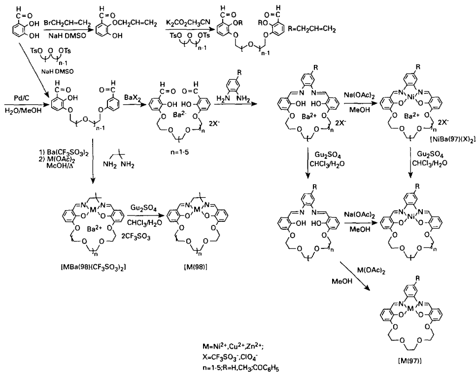
Scheme 32.
