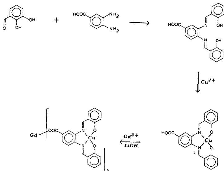
Scheme 58.
