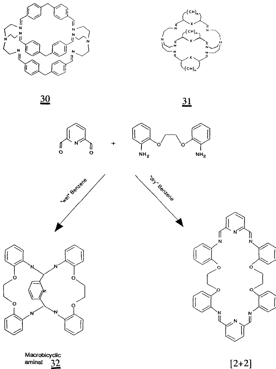
Scheme 6.
