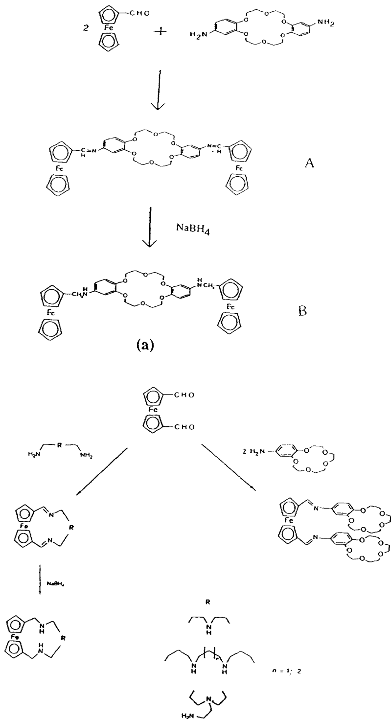
Scheme 53.
