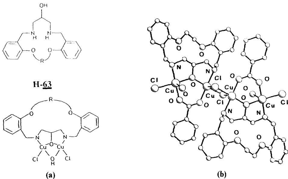
Fig. 45. (a) The proposed structure of the homodinuclear complex \text{Cu}_2(\mathbf{63})(\text{Cl})_2(\text{OH}) . (b) The molecular structure of the tetranuclear complex [\text{Cu}_2(\mathbf{63})(\mu\text{-O}_2\text{CPh})(\text{H}_2\text{O})(\text{Cl})_2]_2 \cdot 2\text{PhCH}_2\text{OH} .
