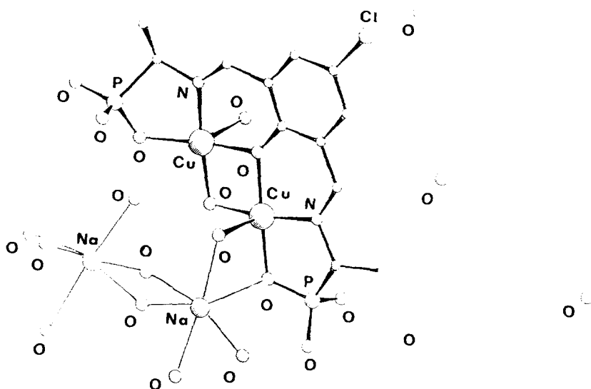
Fig. 64. Structure of [Na 2 Cu 2 ( 83 )(OH)] · 11H 2 O.
