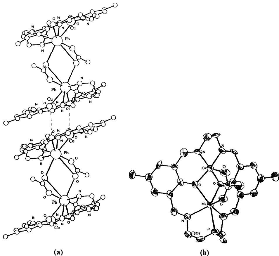
Fig. 84. Structures of (a) [CuPb(109')(CH_3COO)]_n^+ and (b) [CuMn(109')(CH_3COO)]^+ .
