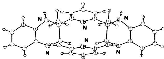
Fig. 15. Structure of 33.
