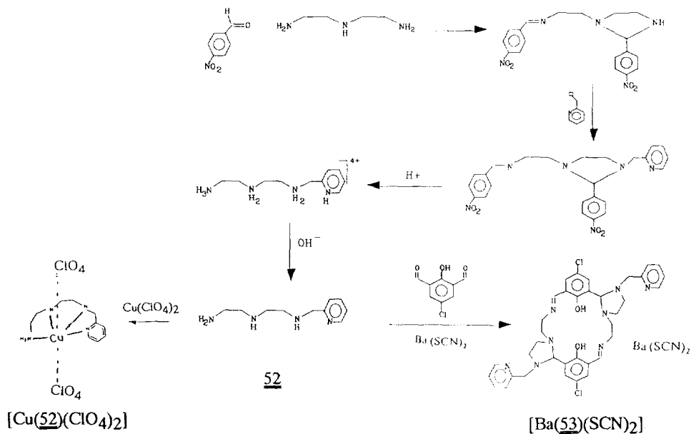
Scheme 20. Preparation of the polyamine 52 and related [\text{Cu(52)(ClO}_4)_2] and [\text{Ba(53)(SCN)}_2] complexes.
