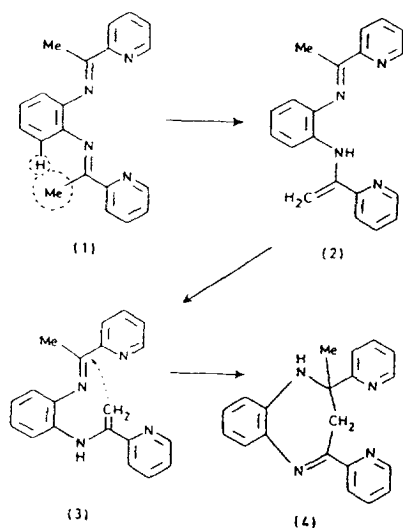
Scheme 7.
