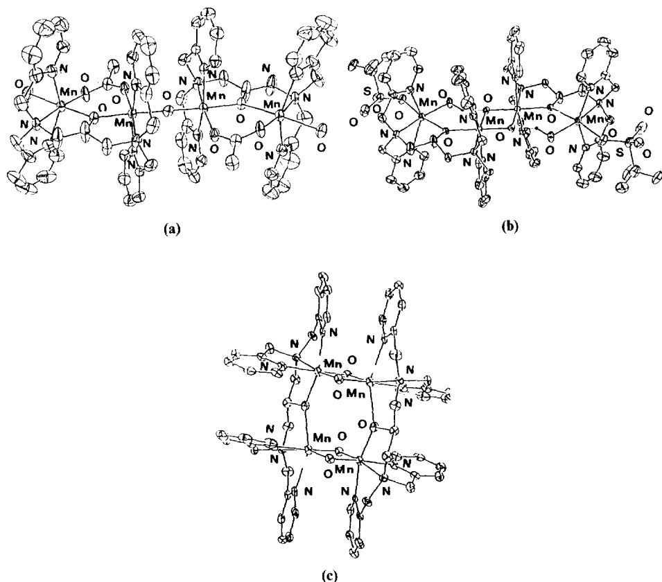
Fig. 100. Structures of (a) \{[\text{Mn}_2(\mathbf{123})(\text{CH}_3\text{COO})(\text{H}_2\text{O})_2]\text{O}\}^{4+} , (b) [\text{Mn}_4\text{O}_2(\mathbf{123})(\text{H}_2\text{O})_2(\text{CF}_3\text{SO}_3)_2]^{3+} and (c) [\text{Mn}_2\text{O}_2(\mathbf{123})_2]^{4+} .
