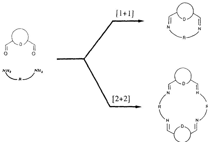
Scheme 5. Schematic representation of the [1+1] and [2+2] Schiff base macrocycles.
