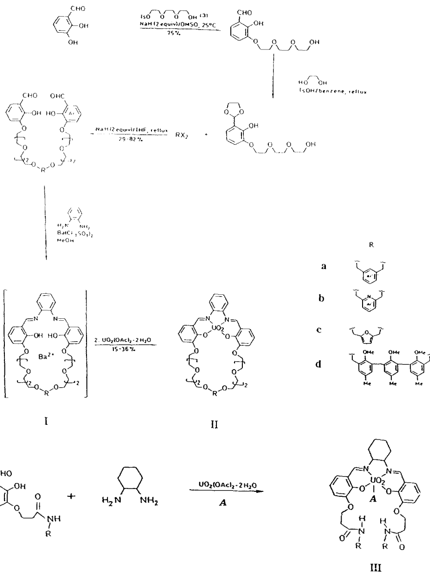
Scheme 13.
