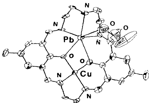
Fig. 59. Structure of [\text{CuPb}(\mathbf{76})(\text{CH}_3\text{COO})][\text{BPh}_4] \cdot \text{CH}_3\text{CN} .
