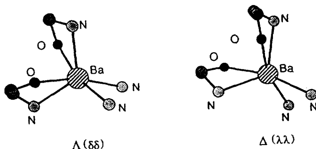
Fig. 19. Representation of two enantiomeric forms of [\text{Ba}(\mathbf{37})]^{2+} .
