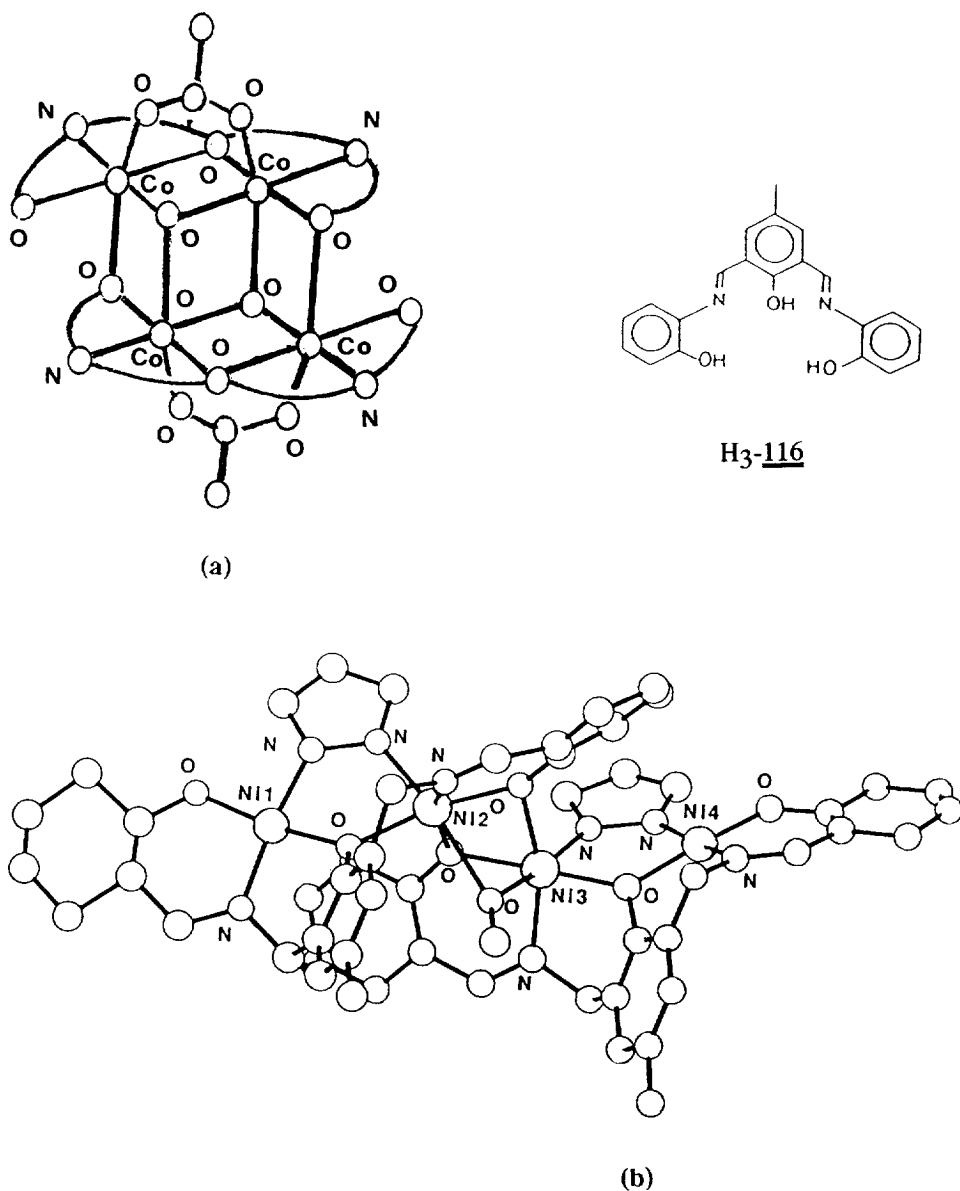
Fig. 91. Structures of (a) [\text{Co}^{\text{II}}\text{Co}^{\text{III}}(\mathbf{116})(\text{OH})(\text{CH}_3\text{COO})]_2 and (b) [\text{Ni}_4(\mathbf{116})(\text{pyrazolate})_2(\text{CH}_3\text{OH})] .
