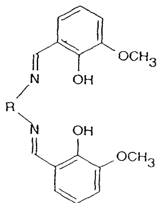
Fig. 70. Structures of (a) [\text{Ni}(\mathbf{92a}) \cdot \text{Sn}(\text{CH}_3)_2(\text{Cl})_2(\text{H}_2\text{O})] and (b) [\text{Ni}(\mathbf{92b}) \cdot \text{Sn}(\text{CH}_3)_2(\text{Cl})_2(\text{H}_2\text{O})_2] .
