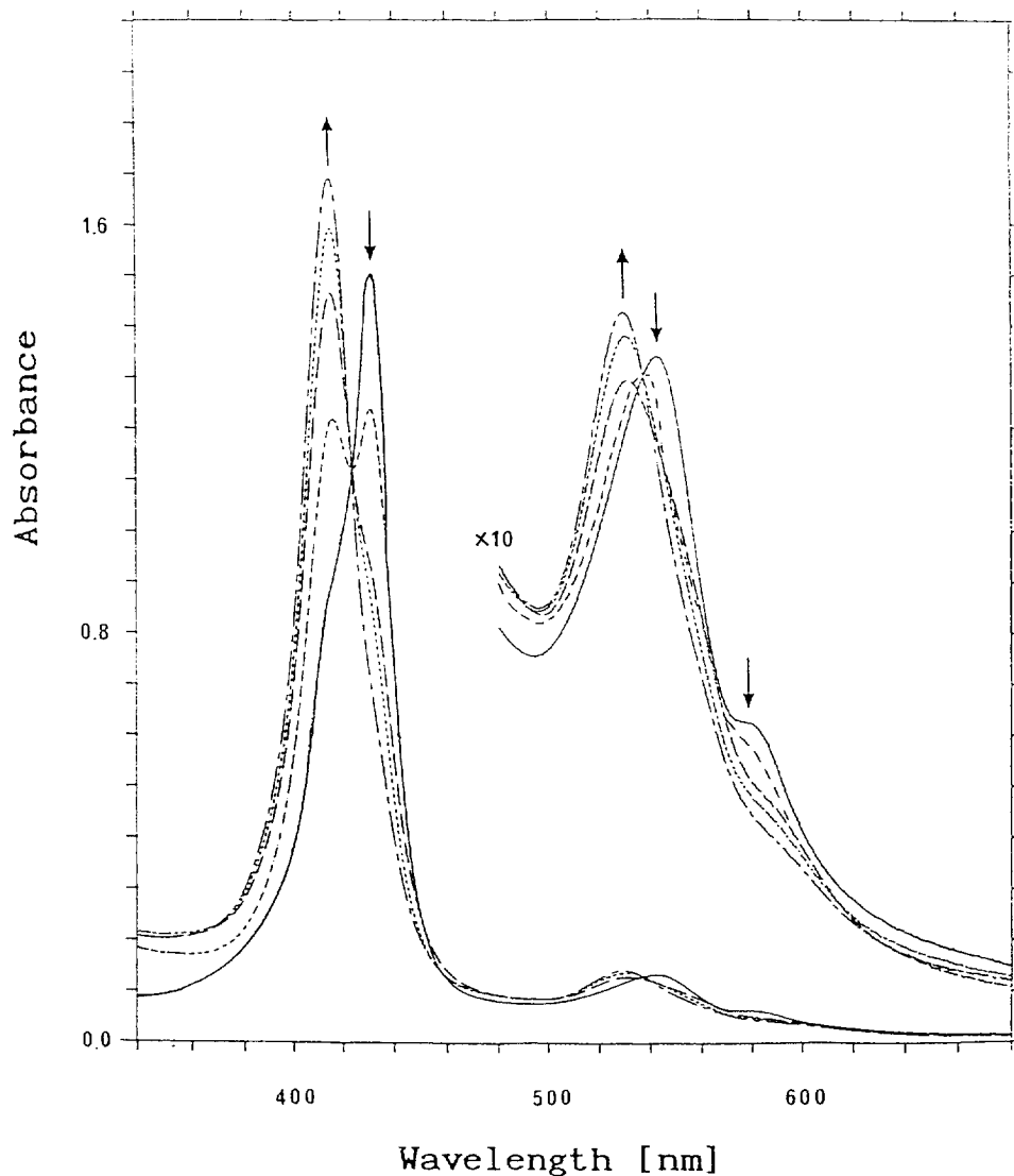
Fig. 5. Photolytic conversion of [\text{Co}(\text{TPP}) (\text{AF})_2] (\text{BF}_4) into \text{Co}(\text{TPP}) in DMF. Arrows indicate the change in absorbance during irradiation at \lambda > 350 \text{ nm} . (With permission from Ref. [20].)
