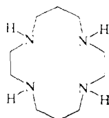
cyclam
