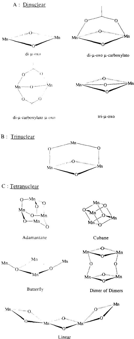
Fig. 5. Structural types of high-valent oxomanganese clusters: A, dinuclear; B, trinuclear; C, tetranuclear.
