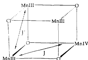
Fig. 15. Exchange couplings in different oxomanganese clusters: A, dinuclear; B, trinuclear; C, cubane. In trinuclear and cubane-type clusters, a vector-coupling model has been used to fit to the magnetic data.
