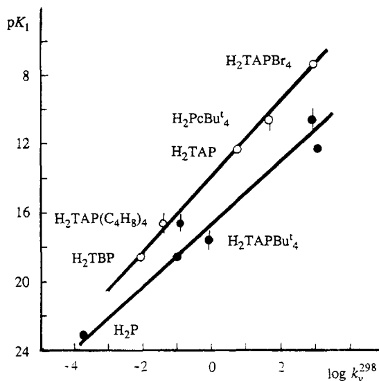
Fig. 6. Correlation between acidity ( pK_1^{298\text{ K}} in DMSO) of porphyrin and tetraazaporphyrin ligands and their reactivity in complexation with Zn (O) and Cu (●) acetates in pyridine ( k_v^{298\text{ K}} ). ( [M(OAc)_2]^0 = 3 \times 10^{-4}\text{ M} ).
