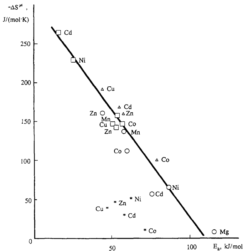
Fig. 12. Kinetic compensation effect in the complexation of tetraazaporphyrin ligands with metal acetates in pyridine: ○, \text{H}_2\text{TAP} ; Δ, \text{H}_2\text{TAP}(\text{C}_4\text{H}_8)_4 ; □, \text{H}_2\text{TAPPh}_8 ; *, \text{H}_2\text{Pc}'\text{Bu}_4 .
