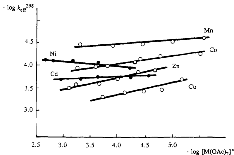
Fig. 10. Dependence of \log k_{\text{eff}}^{298} from \log[M(\text{OAc})_2]^0 for the complexation of \text{H}_2\text{TAPPh}_8 with metal acetates in pyridine.
