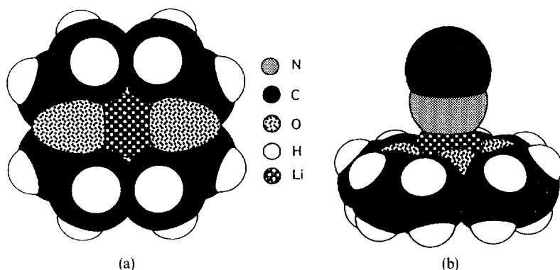
Fig. 6. Optimised structures of (a) the (12\text{-crown-4}) \cdot \text{Li}^+ complex with D_{2d} symmetry and (b) the (12\text{-crown-4}) \cdot \text{Li}(\text{NCS}) complex with C_{4v} symmetry.
