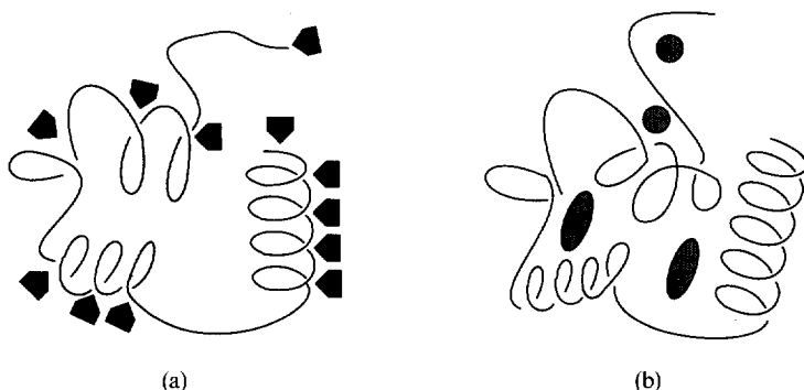
Fig. 12. Schematic illustration of supramolecular assemblies with biopolymers.
