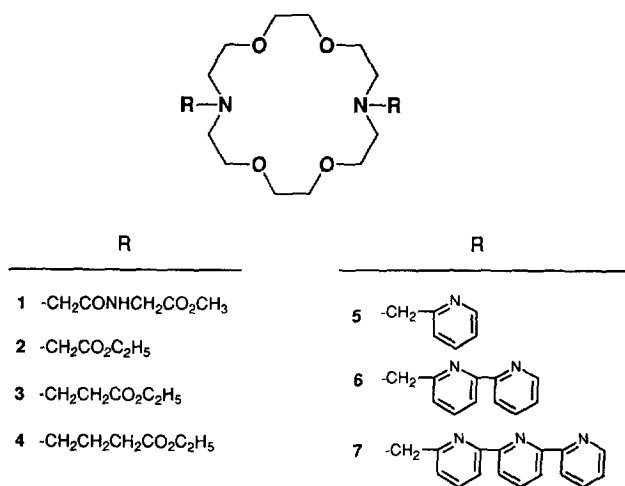
Fig. 3. Typical examples of double-armed crown ether ionophores.
