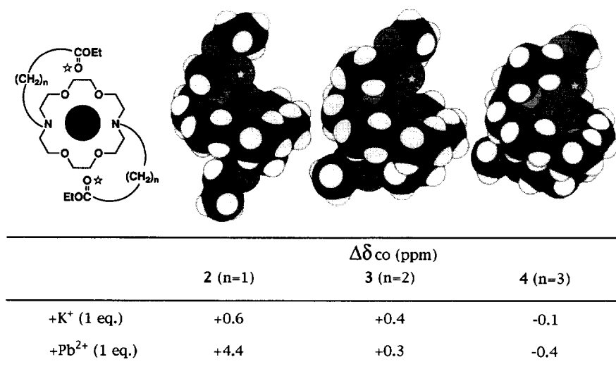
Fig. 4. Optimised structures of ester-armed diaza-18-crown-6 · K + complexes and cation-induced values of ester carbon NMR shifts.
