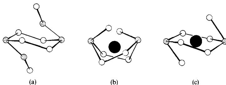
Fig. 2. Skeletal drawings of (a) double-armed crown ether 1 and its (b) \text{Na}^+ and (c) \text{K}^+ complexes.
