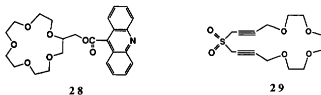
Fig. 14. Typical examples of armed crown ethers for binding of nucleic acids.
