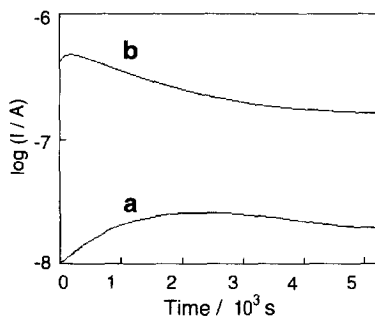
Fig. 7. Isothermal transient ionic currents for composite film of PPFS–Li + –OOEAc–1 ( n=1 ) [35]: (a) under dark conditions; (b) under visible-light-irradiated conditions.
