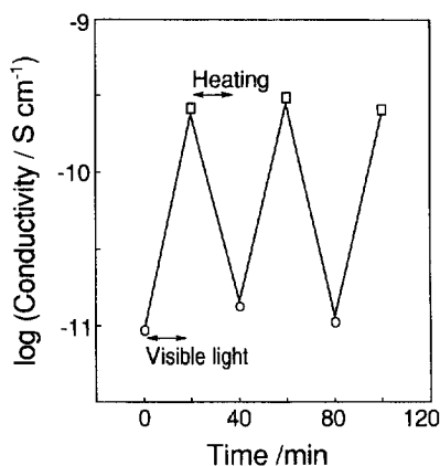
Fig. 6. Photoinduced ionic-conductivity changes in composite film of \text{PPFS-Li}^+ –OOEAc– 1 ( n=1 ) on turning visible light on and off while being heated at 70^\circ\text{C} under dark conditions [35].
