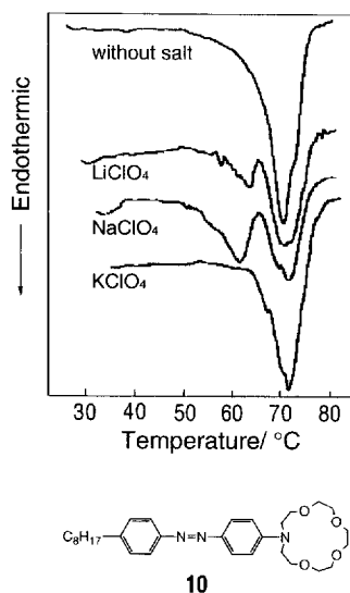
Fig. 12. DSC thermograms for composite films of polyester-crowned azobenzene 10 - \text{MClO}_4 [51].
