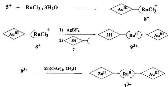
Fig. 3. Stepwise formation of the asymmetrical ruthenium(II) complex 1 3+ .
