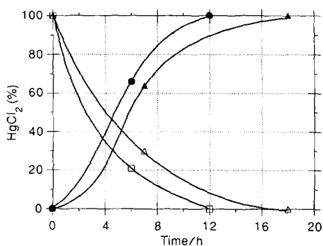
Fig. 14. Transport of \text{Hg}^{2+} with 20e using 2 M HCl and 5 M HCl; \triangle , \text{Hg}^{2+} remaining in 2 M HCl; \bullet , \text{Hg}^{2+} transported in 2 M HCl; \square , \text{Hg}^{2+} remaining in 5 M HCl; \blacktriangle , \text{Hg}^{2+} transported in 5 M HCl.
