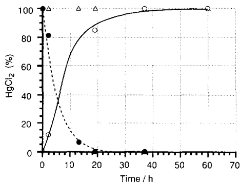
Fig. 12. Extraction and transfer experiments of \text{Hg}^{2+} with 15e in the presence of \text{Cu}^{2+} ; ○, \text{Hg}^{2+} transported; ●, \text{Hg}^{2+} remaining; △, \text{Cu}^{2+} remaining.
