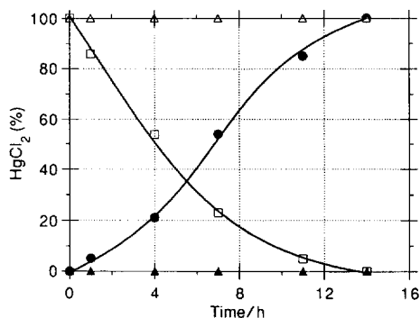
Fig. 17. Selective transport of \text{Hg}^{2+} with 20e; \square , \text{Hg}^{2+} remaining; \bullet , \text{Hg}^{2+} transported; \triangle , \text{Cu}^{2+} remaining; \blacktriangle , \text{Cu}^{2+} transported.
