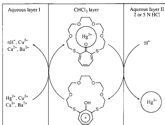
Fig. 19. Transport mechanism.
