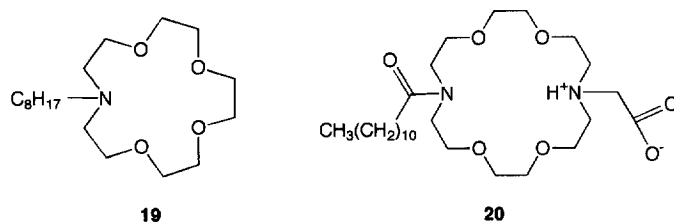
Fig. 9. N -octylmonoaza-15-crown-5 ( 19 ). Zwitterion-type diazacrown ether ( 20 ) reported by Shinkai et al. [30].
