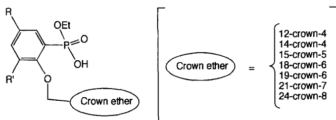
Fig. 2. Some armed crown ethers with phosphonomethyl and phosphonyl functional groups.
