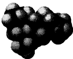
Fig. 5. Side view of computer generated molecular model of crown ether 10 .
