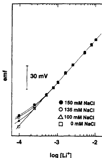
Fig. 13. Typical \text{Li}^+ response curves of the electrodes based on crown ether 10 with different \text{Na}^+ background concentrations. Reproduced from Ref. [43] with permission.
