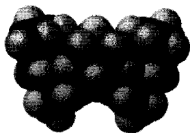
Fig. 4. Side view of computer generated molecular model of crown ether 9 .
