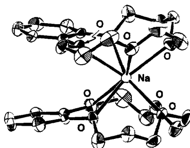
Fig. 9. ORTEP drawing of the 22 –NaClO 4 complex. Hydrogen atoms and perchlorate anion are omitted for clarity.
