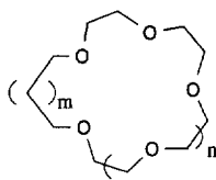
3: m=1, n=1 4: m=2, n=1 5: m=1, n=2 6: m=2, n=2
