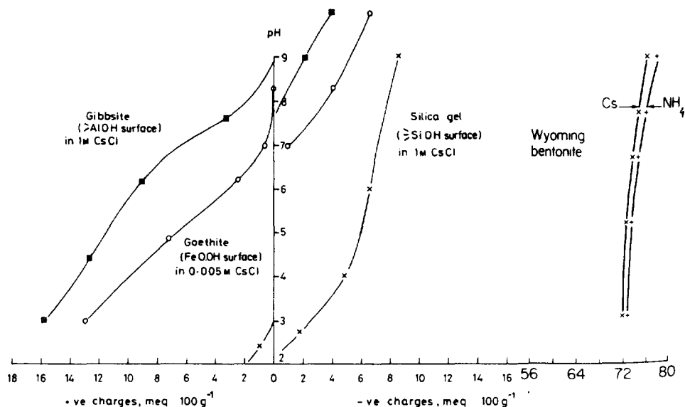
Fig. 15. Charges on gibbsite, goethite, silica and bentonite surfaces in the pH range 3–9. (After Ref. [6]).
