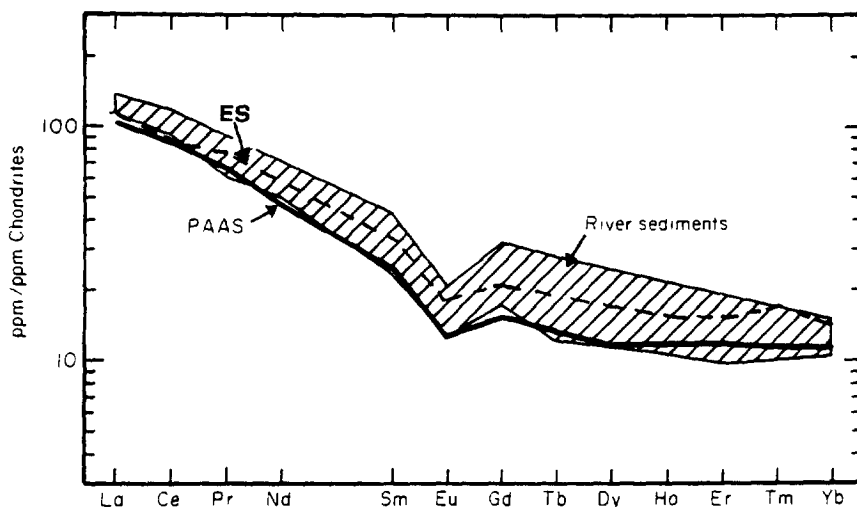
Fig. 14. Chondrite-normalized diagram of post-Archean shale composites (PAAS, ES) and modern river sediments. The uniformity of the patterns support the view that sedimentary REE patterns reflect the upper continental crust exposed to weathering and erosion. Such patterns would best compare to granodioritic composition. (After Ref. [4], modified).
