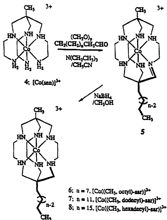
Fig. 7. New synthesis of cage surfactants.
