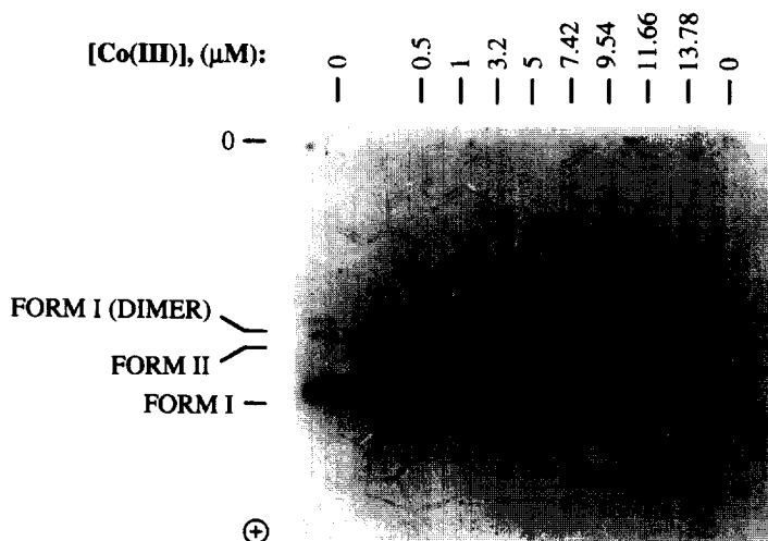
Fig. 16. Effect of [Co(III)anthracenyl cage] 3+ ( 2 ) on electrophoretic mobility of negatively supercoiled plasmid DNA (pUC-9, 32.6 \mu\text{M} ): form I, supercoiled DNA; form II, relaxed circular DNA.
