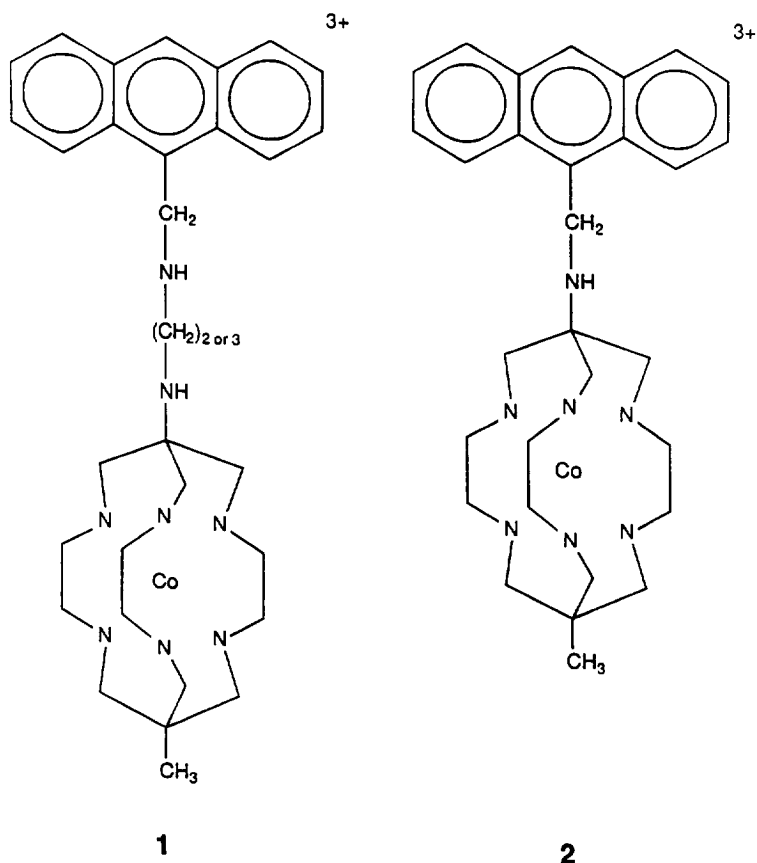
Fig. 13. Anthracenyl cage complexes from reductive alkylations.
