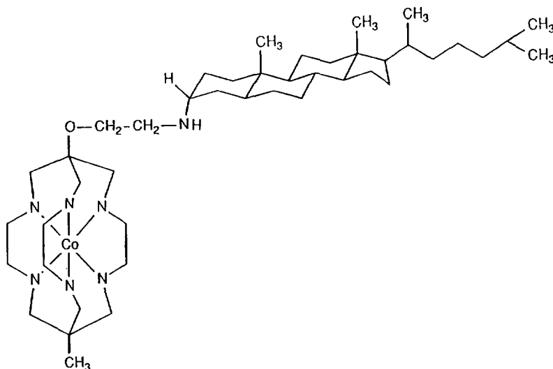
Fig. 5. Cage substituted with a cholestane residue.
