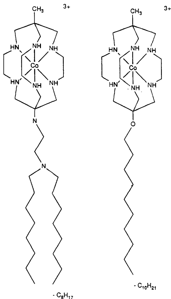
Fig. 6. Examples of cage surfactants.
