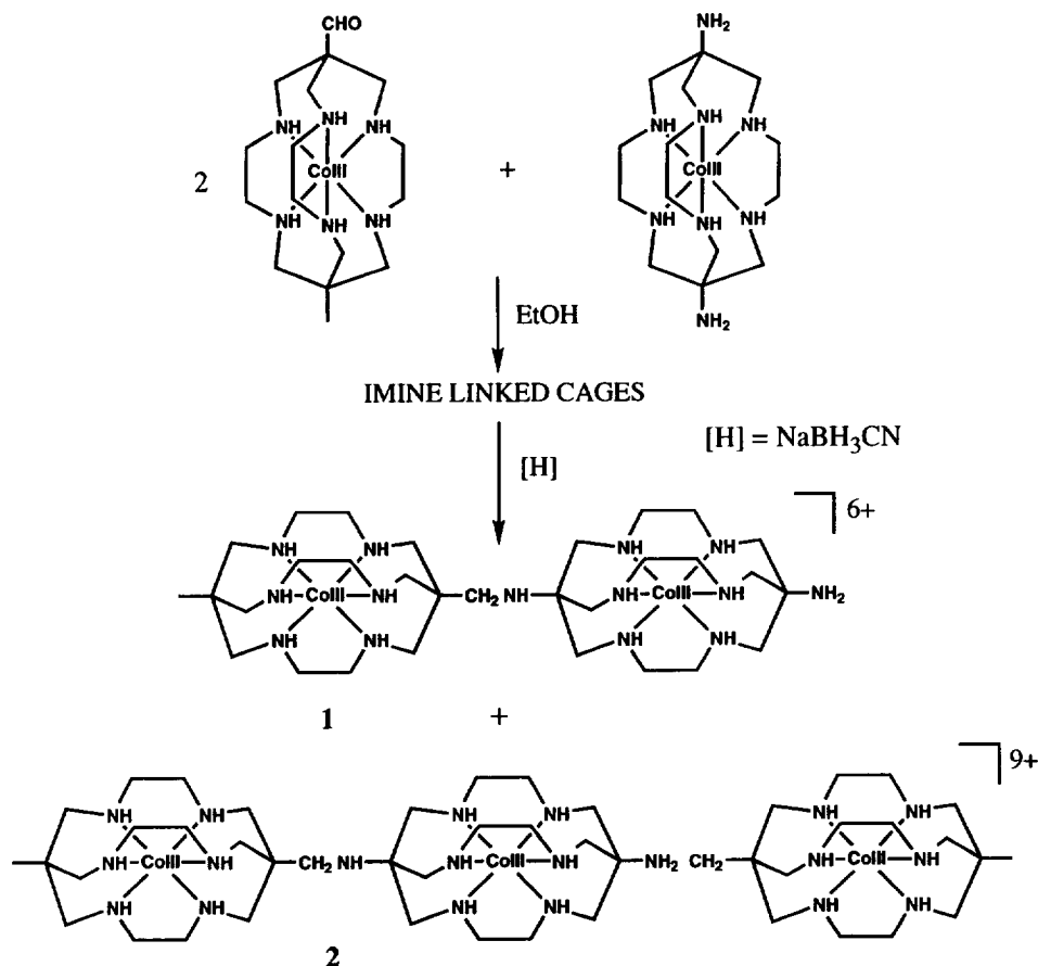
Fig. 18. Coupling of cage complexes by reductive alkylation.
