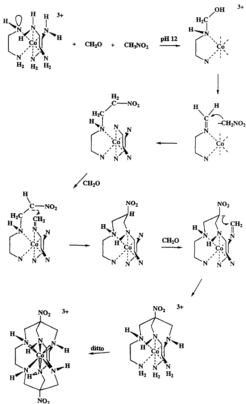
Fig. 2. Template synthesis of [\text{Co}((\text{NO}_2)_2\text{-sar})]^{3+} ion.
