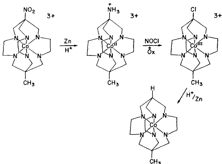
Fig. 3. Variation in substituents for sar-type cages.
