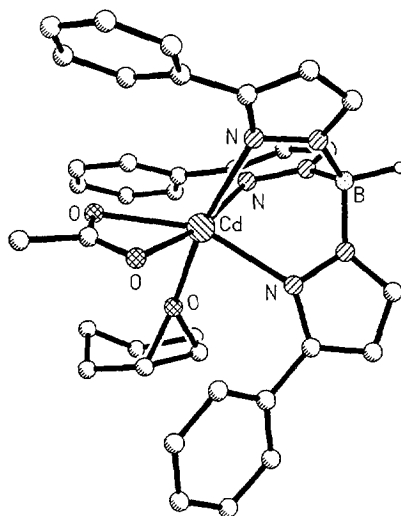
Fig. 1. Ball-and-stick representation of ( \eta^3 -HB(3-Phpz) 3 )Cd(acetate)cyclohexene oxide.
