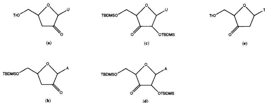
Fig. 6. Derivatives of uridine, adenosine and 2-deoxythymidine.
