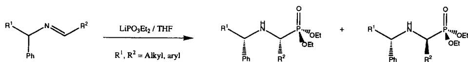
Scheme 8. Phosphonylation of chiral imines.
