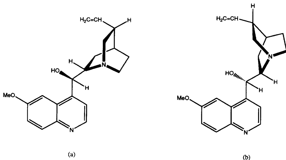
Fig. 11. Non-metal-based catalysts used in asymmetric variants of the Pudovik reaction.
