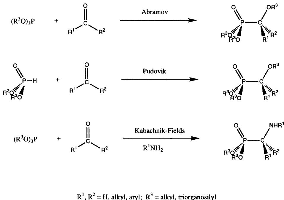
Scheme 3. Three common phonylation processes of prochiral substrates.
