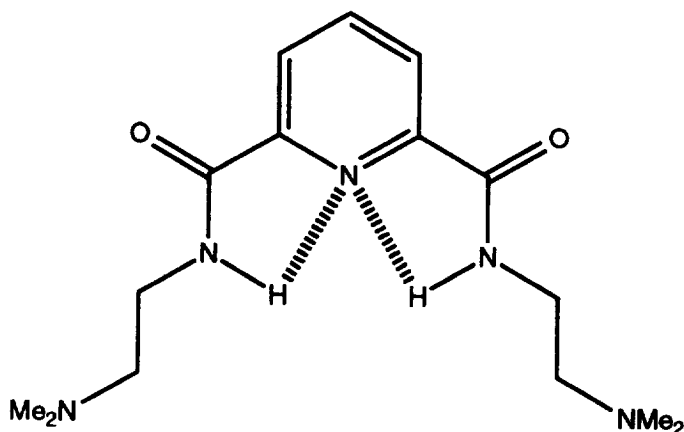
Fig. 12. Amphoteric receptor catalyst for the Pudovik reaction.
