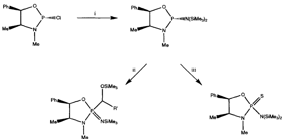
Scheme 11. Synthesis of a chiral 2-(bis-trimethylsilylamido)-1,3,2-oxazaphospholidine derived from (1 R ,2 S )-ephedrine.
