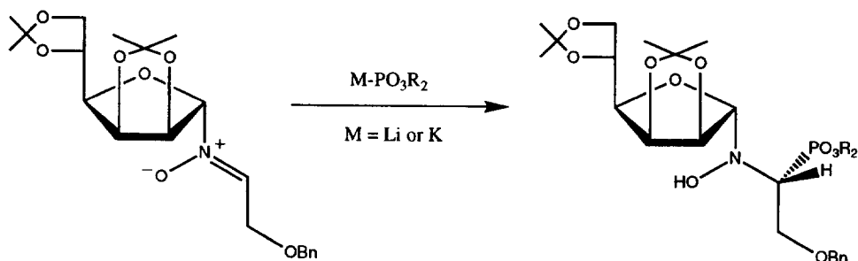
Scheme 5. Phosphonylation of nitrones.
