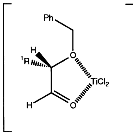
Fig. 7. Proposed Lewis acid activation of functionalised carbonyls via chelate ring formation [53].
