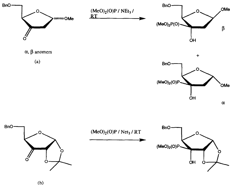
Scheme 14. Phosphonylation of keto-sugars.
