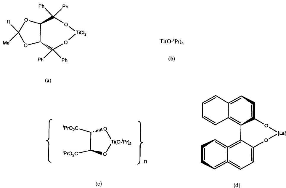
Fig. 10. Metal-based catalysts used in asymmetric variants of the Pudovik reaction.
