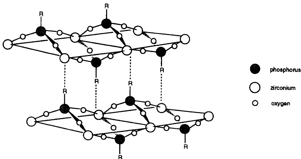
Fig. 4. Lamellar structure of metallophosphonates.
