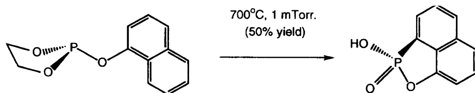
Scheme 4. Thermally induced [P–C] bond formation.
