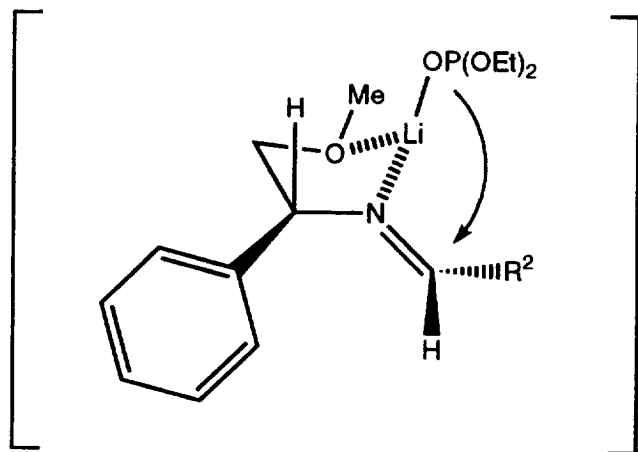
Fig. 8. Proposed intermediate in the asymmetric phosphonylation of chiral chelating functionalised imines [55].
