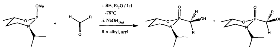
Scheme 13. Abramov phosphonylation of aldehydes via a chiral 1-methoxy-1,3,2-oxazaphospholidine.
