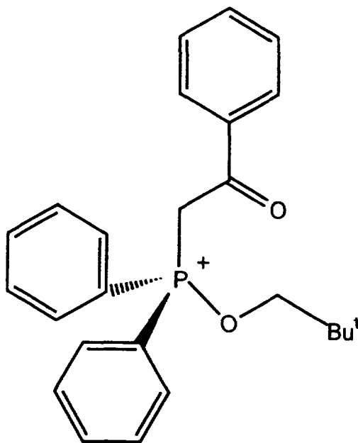
Fig. 5. Structure of neopentyloxy(phenacyl)diphenylphosphonium bromide (anion omitted for clarity).
