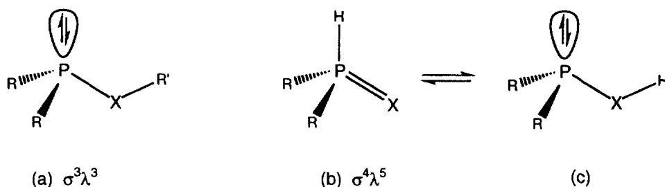
Fig. 2. Common classes of reagent in [P–C] bond-forming reactions.
