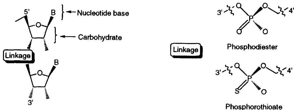
Fig. 3. Modified nucleotides.
