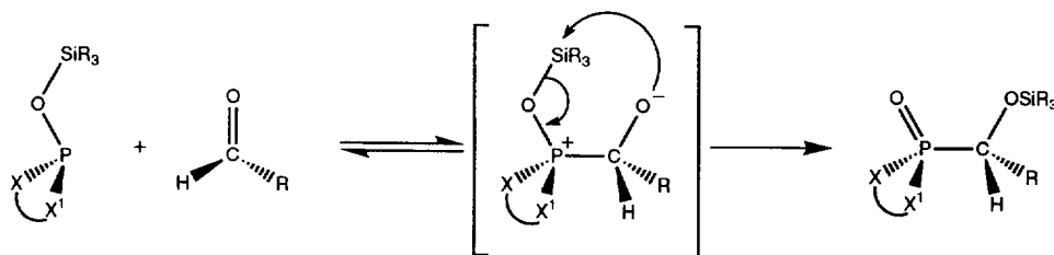
Scheme 9. A proposed mechanism of the asymmetric Abramov reaction.
