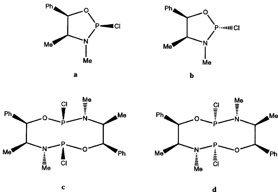
Fig. 9. Possible monomeric and dimeric forms of the chiral 2-chloro-1,3,2-oxazaphospholidine derived from (1 R ,2 S )-ephedrine.
