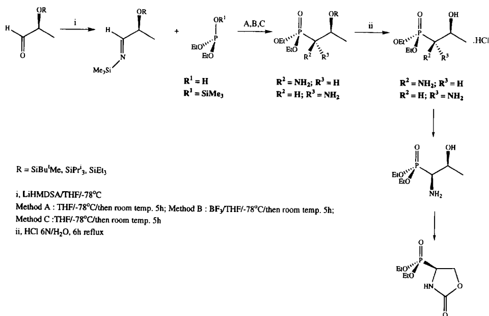
Scheme 6. Phosphonylation of chiral imines.
