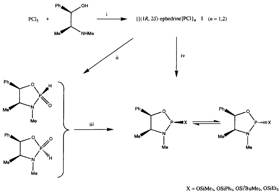
Scheme 10. Syntheses of oxazaphospholidine heterocycles.
