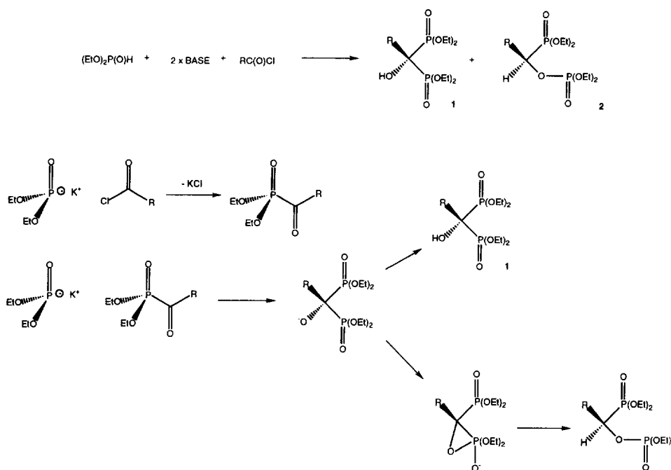
Scheme 2. Acylation of secondary phosphites and their metal salts.
