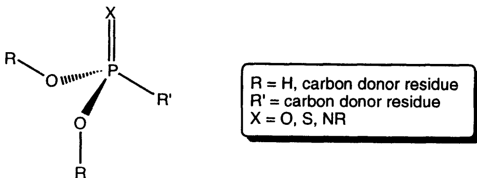
Fig. 1. Phosphonate ester topology.
