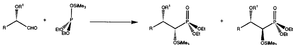
Scheme 7. Phosphonylation of chiral aldehydes.
