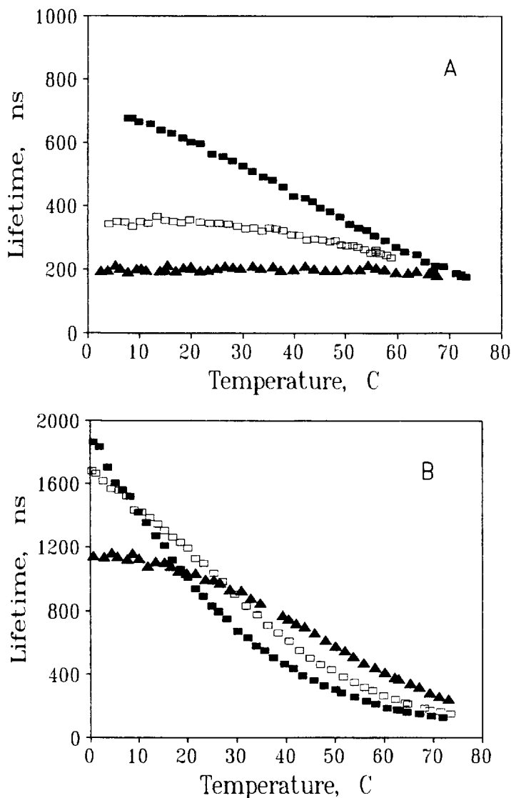
Fig. 3. Temperature dependence of luminescence lifetime in aqueous solution of [\text{Ru}(\text{L})_3]^{2+} - \text{Ag}^+ systems at ambient temperature: L=bpy (a) and L=phen (b); [\text{Ag}^+] = 0 \text{ M} (■), [\text{Ag}^+] = 0.3 \text{ M} (□) and [\text{Ag}^+] = 1.5 \text{ M} (▲).
