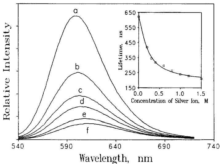
Fig. 1. Change in the uncorrected emission spectrum and the luminescence lifetime (inset) with silver ion concentration in aqueous solution of [\text{Ru}(\text{bpy})_3]^{2+} at 3 M ionic strength and ambient temperature: [\text{Ag}^+] = 0 M (a); 0.2 M (b); 0.4 M (c); 0.6 M (d); 1.0 M (e); 1.5 M (f); \lambda_{\text{exc}} = 450 nm for measurement of luminescence spectrum and \lambda_{\text{exc}} = 355 nm for lifetime measurements.
