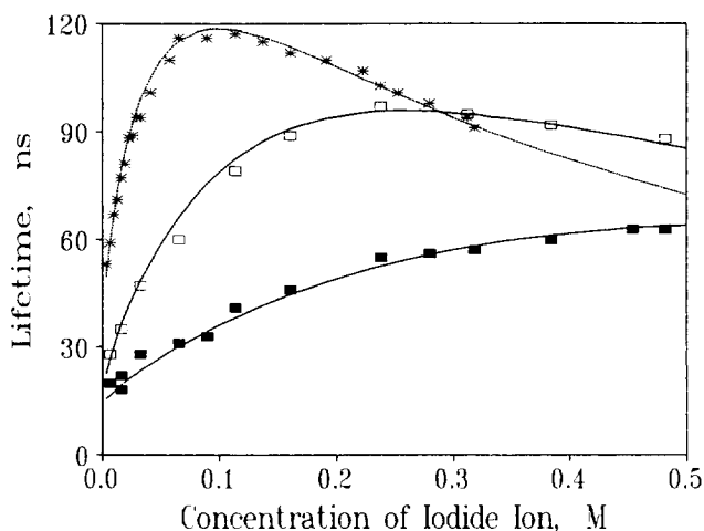
Fig. 5. Influence of ionic strength on luminescence lifetime vs. iodide ion concentration in aqueous solution of dicyanocuprate at ambient temperature, \lambda_{\text{exc}} = 266 \text{ nm} ; \mu = 0.5 \text{ M} (■); \mu = 2.5 \text{ M} (□); \mu = 5.0 \text{ M} (*) [17].
