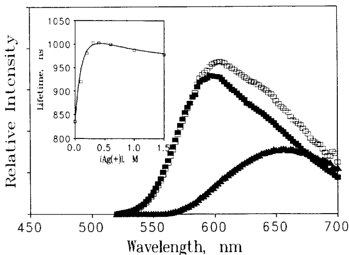
Fig. 2. The calculated luminescence spectra of ^*[Ru(phen)_3]Ag_n^{(n-2)+} species; (■) n=0 , (□) n=1 and (▲) n=2 . The inset shows the change in luminescence lifetime with silver ion concentration in aqueous solution of [Ru(phen)_3]^{2+} at 3 M ionic strength and ambient temperature; measured (□) and calculated values (—).
