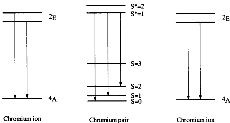
Fig. 3. Energy levels of exchange coupled chromium pairs (schematic).
