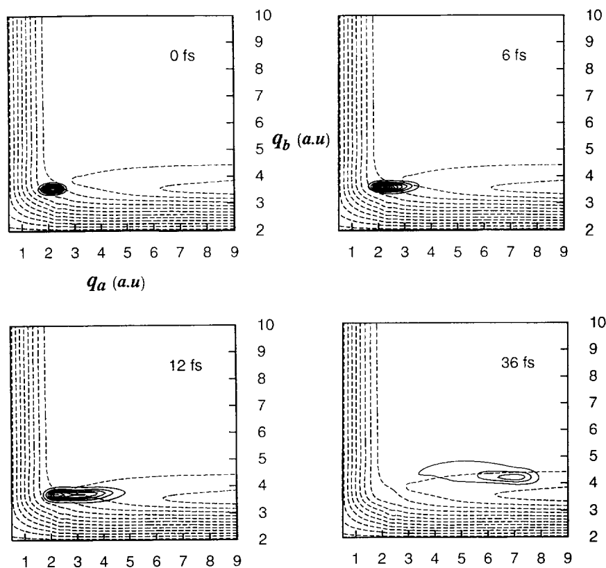
Fig. 2. Time evolution of the \Psi_{b^1A_1}(q_a, q_b, t) wave packet on the V_{b^1A_1}(q_a, q_b) PES of H 2 Fe(CO) 4 ( b^1A_1 ), from the initial state \Psi_{b^1A_1}(q_a, q_b, 0) = |0, 0\rangle_{a^1A_1} prepared by absorption a^1A_1 \rightarrow b^1A_1 [24].
