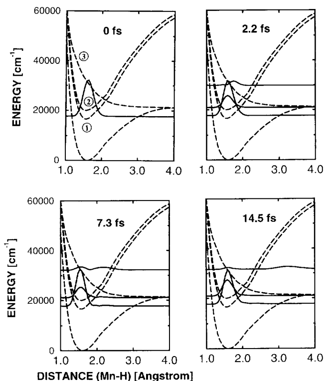
Fig. 7. Diabatic time evolution of the \Psi_{a^3A_1}(q_a, t) wave packet (continuous line) on diabatically coupled V_{a^3A_1}^d(q_a) , V_{b^3A_1}^d(q_a) , and V_{c^3A_1}^d(q_a) PECs (dashed lines labeled (1), (2) and (3)) of \text{HMn}(\text{CO})_3(\alpha\text{-diimine}) with the initial conditions \Psi_{b^3A_1}(q_a, 0) = \Psi_{c^3A_1}(q_a, 0) = 0 and the initial state \Psi_{a^3A_1}(q_a, 0) = |0, 0\rangle_{a^3A_1} , prepared by ISC.
