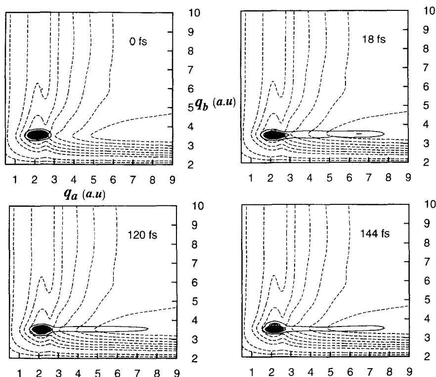
Fig. 6. Time evolution of the \Psi_{a^1B_2}(q_a, q_b, t) wave packet on the V_{a^1B_2}(q_a, q_b) PES of H_2Fe(CO)_4(^1B_2) , from the initial state \Psi_{a^1B_2}(q_a, q_b, 0) = |0, 0\rangle_{a^1A_1} prepared by absorption a^1A_1 \rightarrow a^1B_2 [24].
