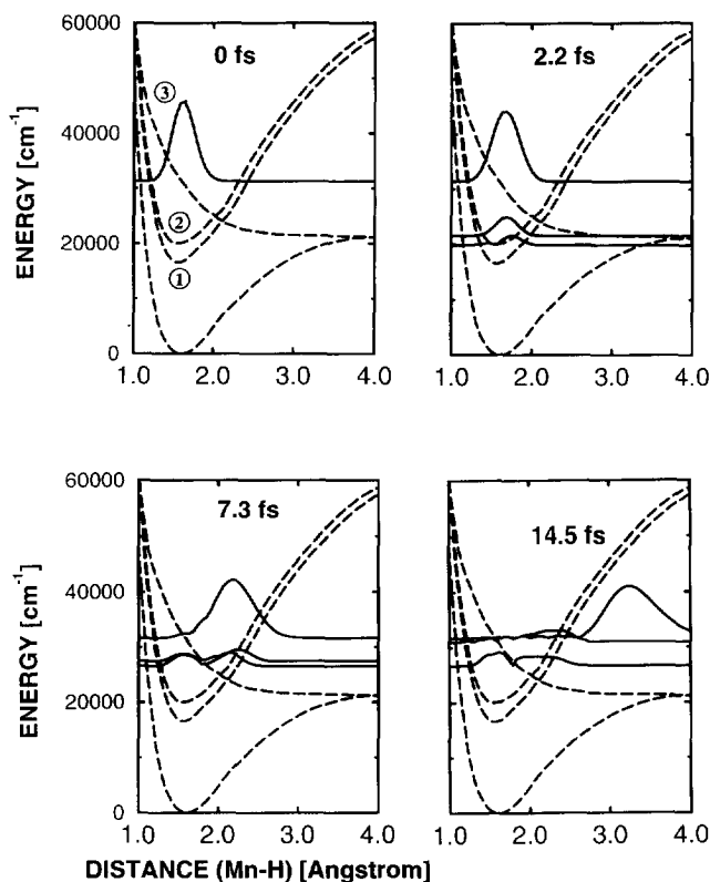
Fig. 8. Diabatic time evolution of the \Psi_{c^3A_1}(q_a, t) wave packet on diabatically coupled V_{a^3A_1}^d(q_a) , V_{b^3A_1}^d(q_a) , and V_{c^3A_1}^d(q_a) PECs (dashed lines labeled (1), (2) and (3)) of \text{HMn(CO)}_3(\alpha\text{-diimine}) with the initial conditions \Psi_{a^3A_1}(q_a, 0) = \Psi_{b^3A_1}(q_a, 0) = 0 and the initial state \Psi_{c^3A_1}(q_a, 0) = |0, 0\rangle_{a^1A_1} , prepared by ISC.
