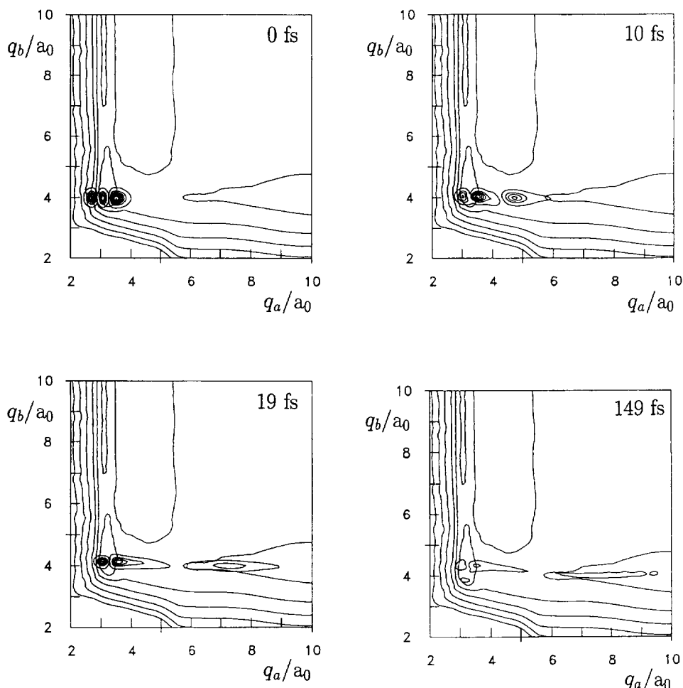
Fig. 11. Time evolution of the \Psi_{1E}(q_a, q_b, t) wave packet on the V_{1E}(q_a, q_b, t) PES of \text{HCo(CO)}_4(^1E) from the initial state \Psi_{1E}(q_a, q_b, 0) = |2, 0\rangle_{1A_1} , prepared by a two-photon laser IR + UV strategy.
