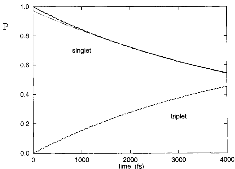
Fig. 10. ISC ^1E \rightarrow ^3A_1 in HCo(CO)_4 , induced by Co-CO_{ax} vibrations. The probabilities P(^1E) and P(^3A_1) for observing HCo(CO)_4 in its ^1E and ^3A_1 states are shown by continuous and dashed lines respectively.
