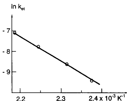
Fig. 10. Arrhenius plot for the rate constant of the thermal electron transfer activation of dioxygen by \text{BQ}[\text{Pt}(\text{mnt})_2] in propylene carbonate at 142–182°C.
