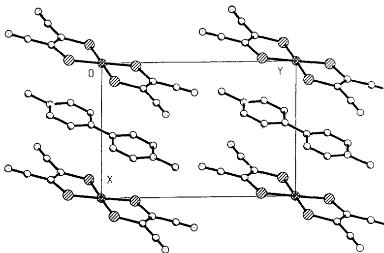
Fig. 2. Solid-state structure of the ion pair MV[Pd(mnt)_2] .
