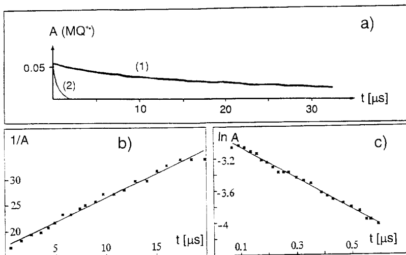
Fig. 7. Laser flash photolysis ( \lambda_{exc} = 347 nm) of MQ[Pt(mnt)_2] in argon (1) and air (2) saturated DMSO solution; (a) decay of MQ^{\bullet+} measured at \lambda = 380 nm; (b) corresponding second order; (c) first-order kinetic plots.
