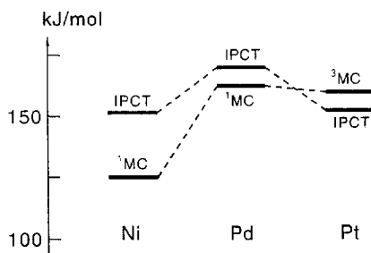
Fig. 8. Energy of lowest excited states for MQ[M(mnt)_2] , M = Ni, Pd, Pt .
