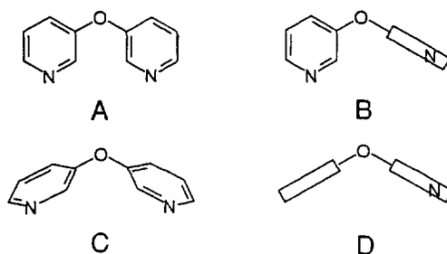
Fig. 5. A–D conformers for 3,3'-oxybispyridine.
