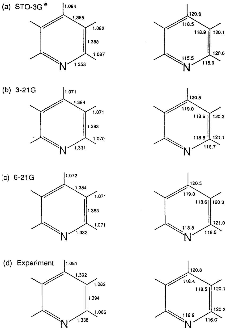
Fig. 2. Pyridine geometry optimized using (a) STO-3G, (b) 3-21G and (c) 6-21G sets, and (d) experimental structure determined by Sorensen et al. [52]. Reproduced with permission from reference [49].
