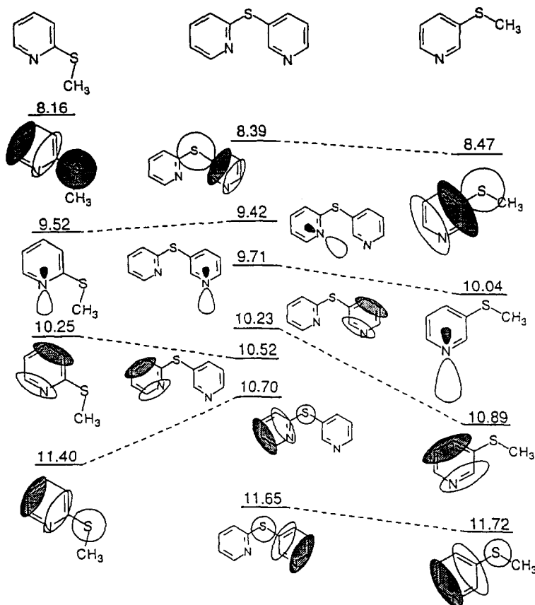
Fig. 11. Correlation diagram of the experimental IEs of 2,3'-thiobispyridine with those of 2- and 3-methylthiopyridine. Only significant contributions to the MOs are shown. Reproduced with permission from reference [23].
