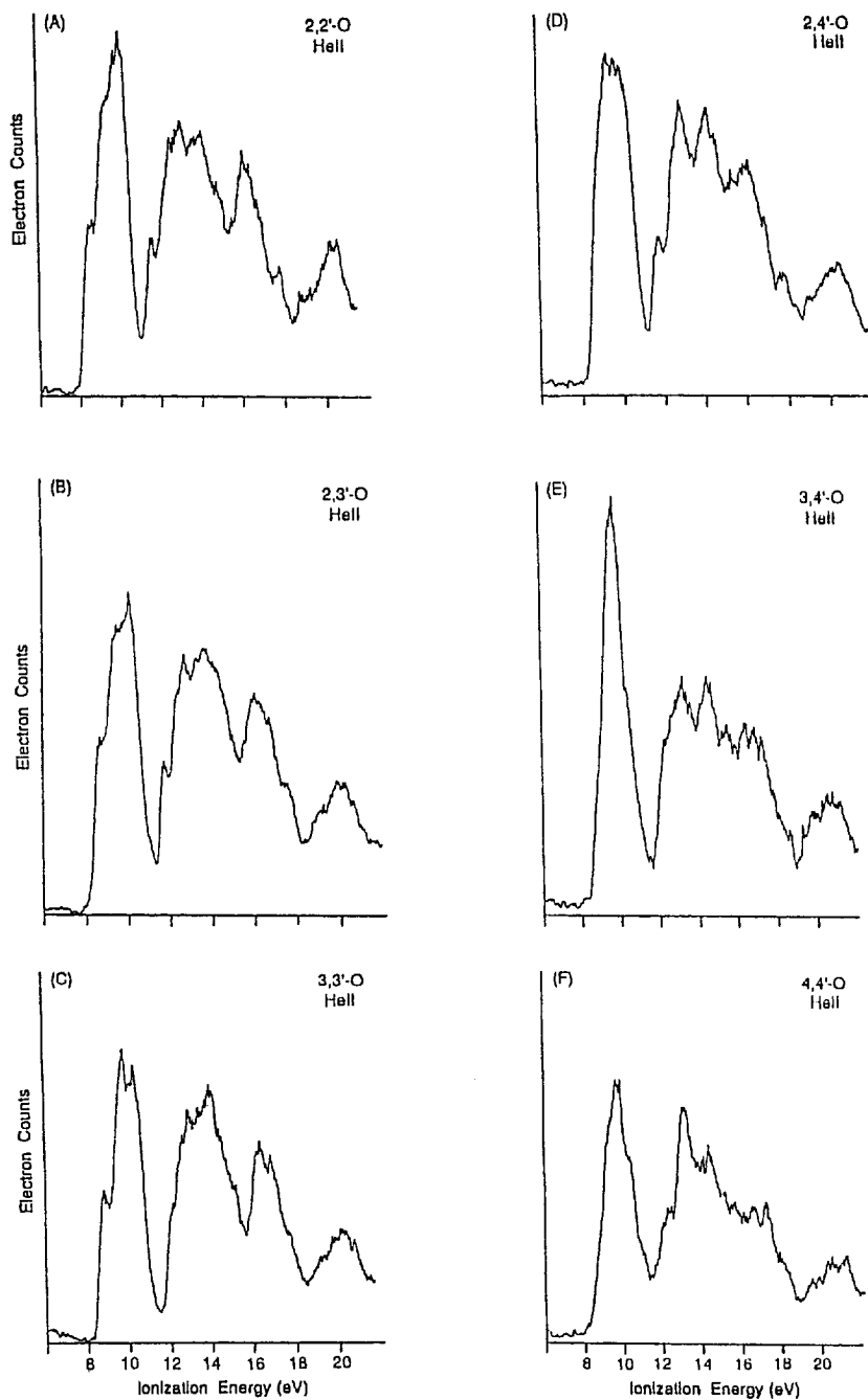
Fig. 7. HeII spectra of (a) 2,2'-oxybispyridine; (b) 2,3'-oxybispyridine; (c) 3,3'-oxybispyridine; (d) 2,4'-oxybispyridine; (e) 3,4'-oxybispyridine; (f) 4,4'-oxybispyridine. Reproduced with permission from reference [22].
