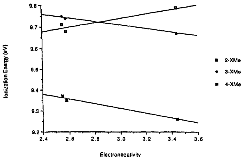
Fig. 14. Plot of the calculated \Delta\text{SCF-CI } n_N IEs vs. Allred electronegativities for the methylchalcogenopyridines, along with the lines of best fit from the regression analyses: \square , 2-methylchalcogenopyridines, with \text{IE}(n_N) = 9.419 + 0.108 and electronegativity R^2 = 0.915 ; \blacklozenge , 3-methylchalcogenopyridines, with \text{IE}(n_N) = 9.966 - 0.086 and electronegativity R^2 = 0.993 ; \blacksquare , 4-methylchalcogenopyridines, with \text{IE}(n_N) = 9.955 - 0.115 and electronegativity R^2 = 0.980 .
