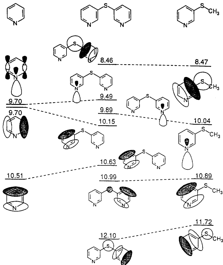
Fig. 10. Correlation diagram of the experimental IEs of 3,3'-thiobispyridine with those of pyridine and 3-methylthiopyridine. Only significant contributions to the MOs are shown. Reproduced with permission from reference [23].
