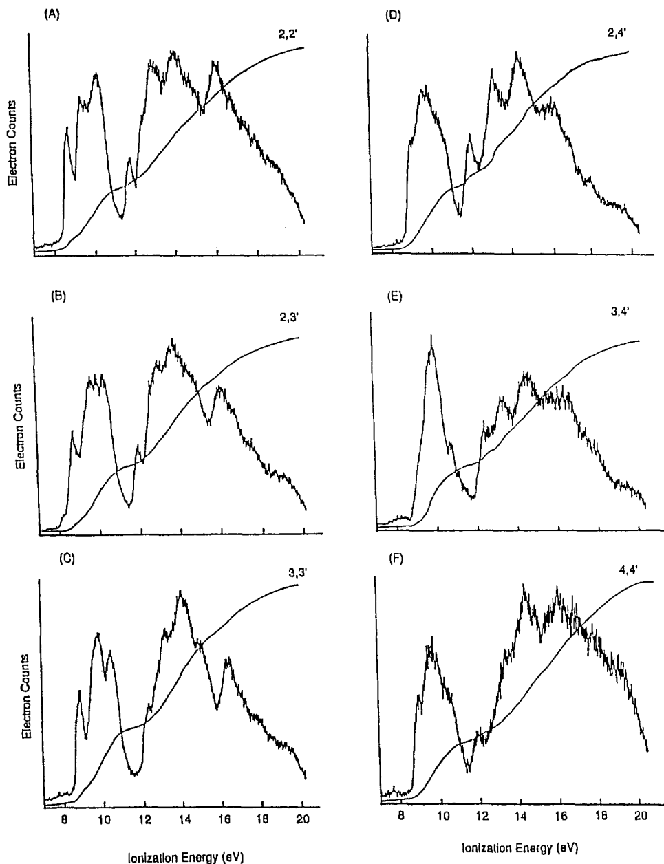
Fig. 6. HeI spectra of (a) 2,2'-oxybispyridine; (b) 2,3'-oxybispyridine; (c) 3,3'-oxybispyridine; (d) 2,4'-oxybispyridine; (e) 3,4'-oxybispyridine; (f) 4,4'-oxybispyridine. Reproduced with permission from reference [22].
