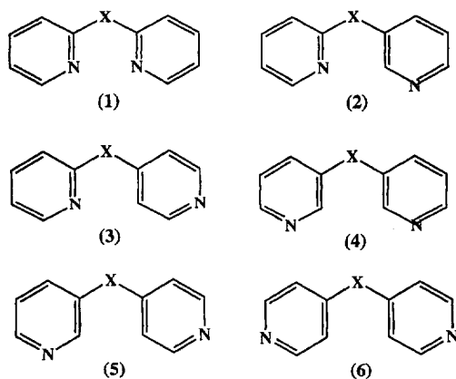
Fig. 1. Structural formulae of the six isomers of the chalcogenobispyridines.
