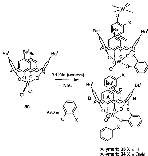
Scheme 12.
