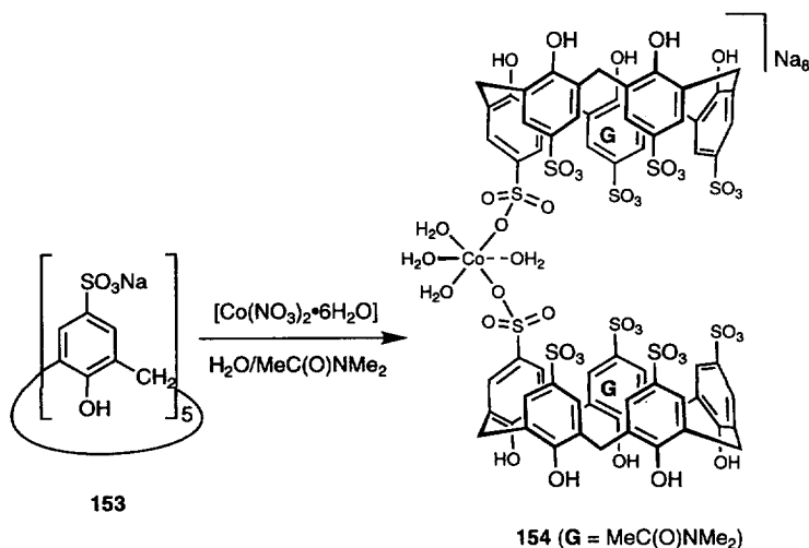
Scheme 32.
