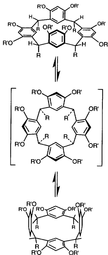
Scheme 40.
