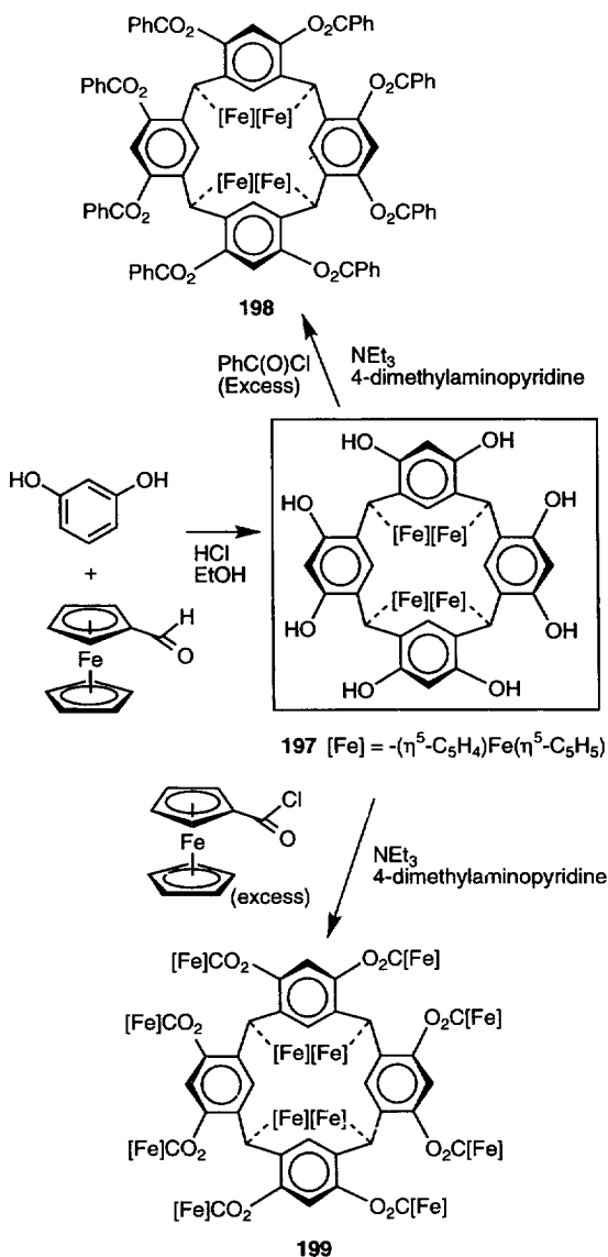
Scheme 39.
