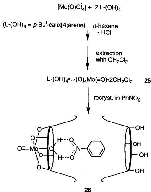
Scheme 7.
