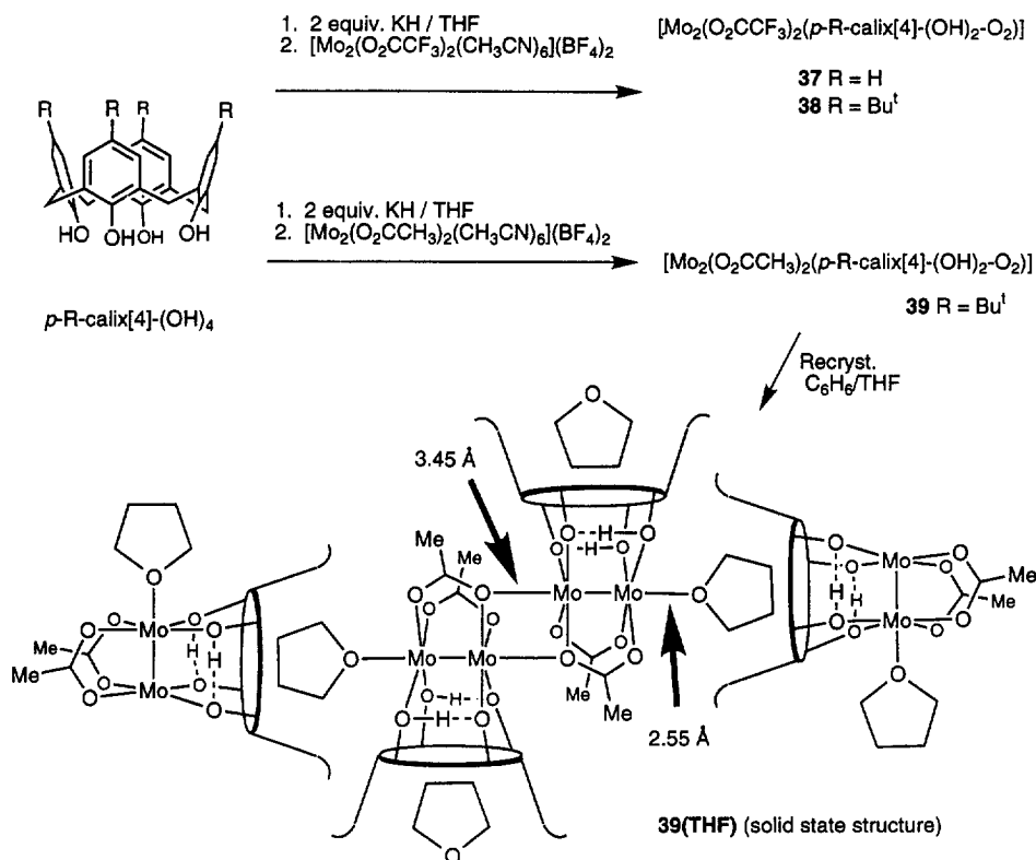
Scheme 13.
