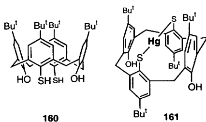
Scheme 33.
