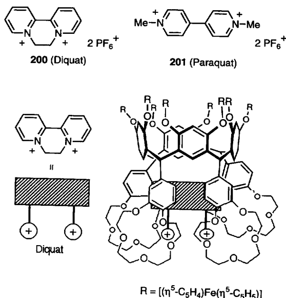
Scheme 41.
