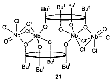
Scheme 5.
