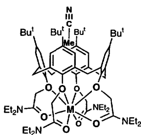
147 (CH 3 CN) M = Fe II
