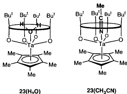
Scheme 6.
