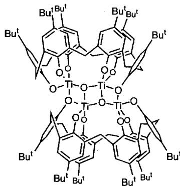
43 (OH atoms not located)
