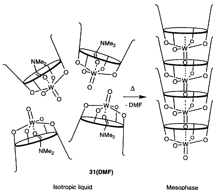
Scheme 11.
