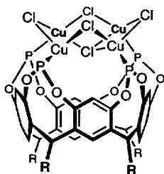
116 R = CH_2CH_2Ph ( PhP groups not drawn)
