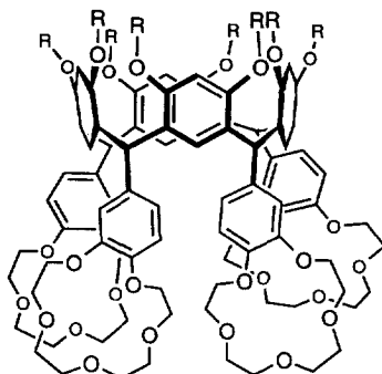
188 R = -C(O)( \eta^5 -C 5 H 4 )Fe( \eta^5 -C 5 H 5 )
