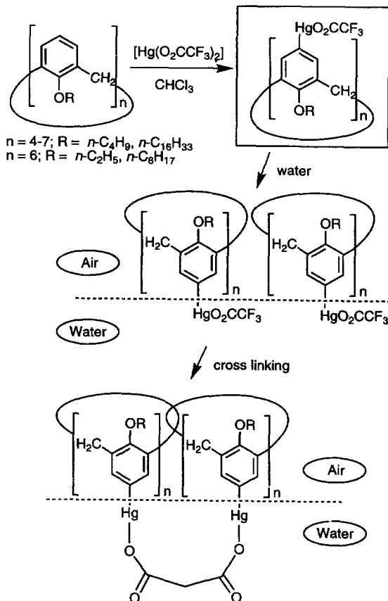
Scheme 35.
