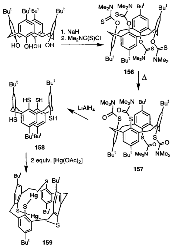
Scheme 33.
