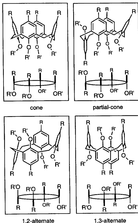
Scheme 1.
