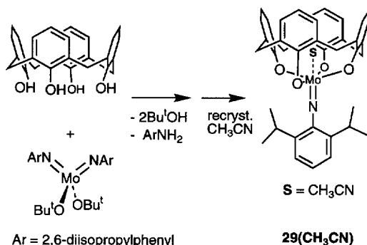
Scheme 9.
