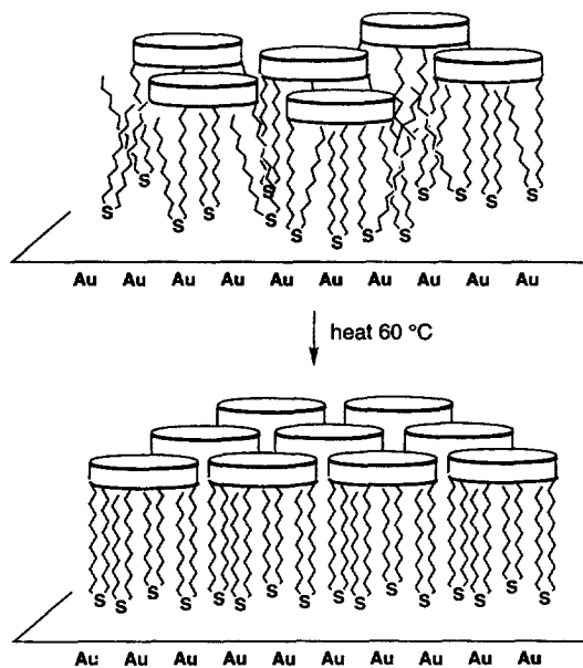
Scheme 34.
