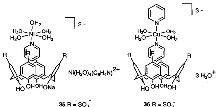
Scheme 12.
