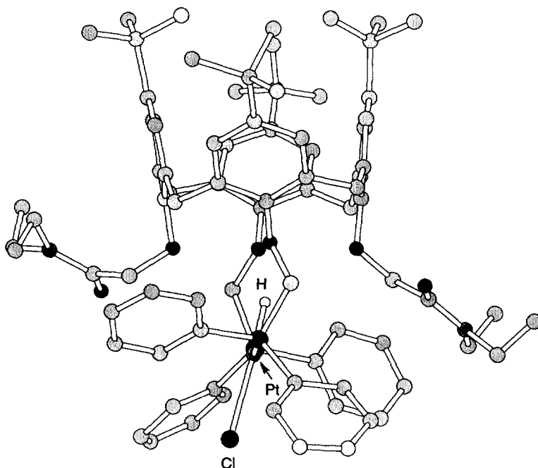
Fig. 2. Molecular structure of trans -[PtHClL 127 ] ( 136 ).
