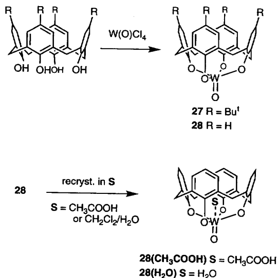
Scheme 8.
