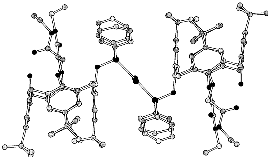
Fig. 1. Molecular structure of trans -[PdCl 2 L 2 85 ] ( 101 ).
