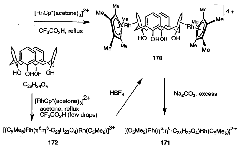
Scheme 36.
