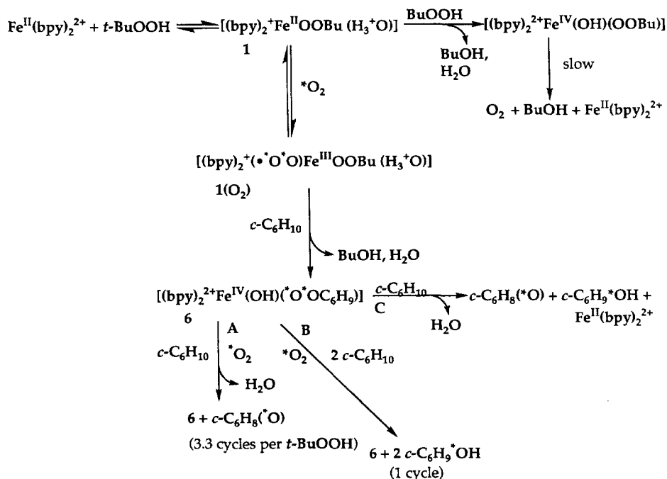
Scheme 2. Proposed pathways and intermediates for the metal/hydroperoxide-induced activation of \text{O}_2 for the ketonization of cyclohexane ( c\text{-C}_6\text{H}_{10} ).
