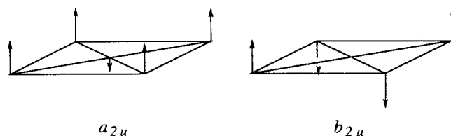
Fig. 24. The a_{2u} and b_{2u} bending modes in square planar coordination.
