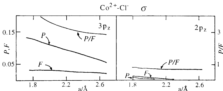
Fig. 16. The markedly smaller P:F ratios for inner orbitals [52].
