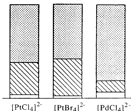
Fig. 28. Relative contributions of the three ungerade bonding modes (open for a_{2u} , hatched for b_{2u} and shaded for e_u ) to the intensity in the ligand-field spectra (integrated over all ' d-d ' bands) for [\text{PtCl}_4]^{2-} , [\text{PtBr}_4]^{2-} and [\text{PdCl}_4]^{2-} .
