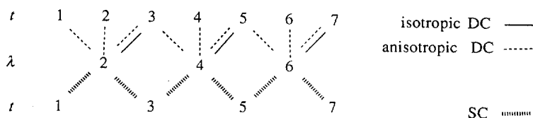
Fig. 7. Possible values of t for SC and DC models.
