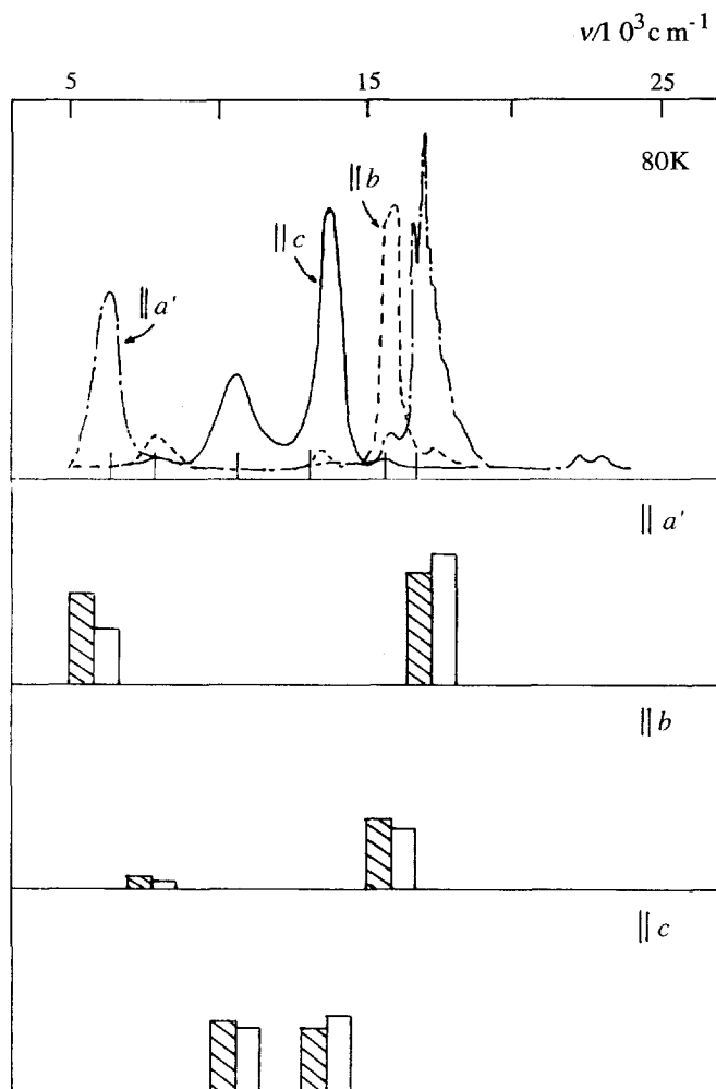
Fig. 25. Observed and calculated (hatched) intensities for \text{CoP}_2\text{Cl}_2 .
