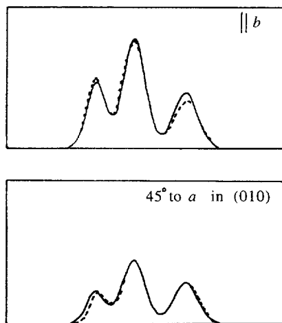
Fig. 29. Reproduction of spectral traces in NMPH ( 16 ).
