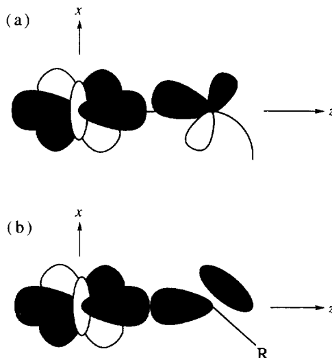
Fig. 18. Misdirected valency: (a) for bent bonding, perhaps due to chelation; and (b) from the effects of the non-dative ligand lone pair.
