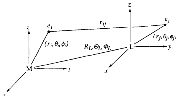
Fig. 4. Coordinates for metal and ligand electrons.
