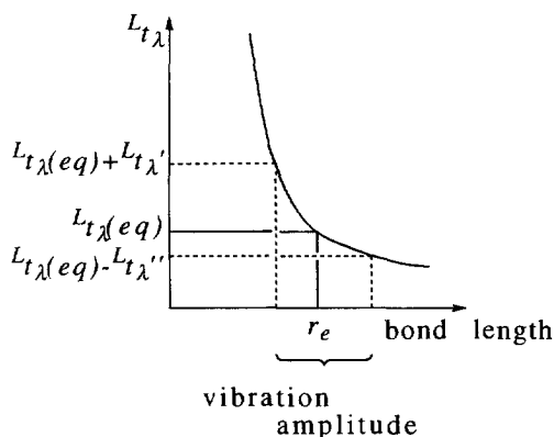
Fig. 21. The variation of {}^L t_{\lambda} values in stretching modes.
