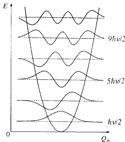
Fig. 1. Vibrational hermite polynomials.
