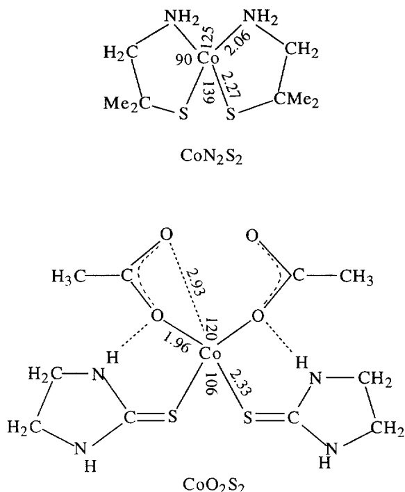
Fig. 31. Chromophores 8 and 9.
