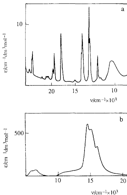
Fig. 8. (a) Electronic ' f - f ' spectrum of a saturated aqueous solution of \text{Nd}^{3+} ions; (b) electronic ' d - d ' spectrum of a solution of [\text{CoCl}_4]^{2-} .
