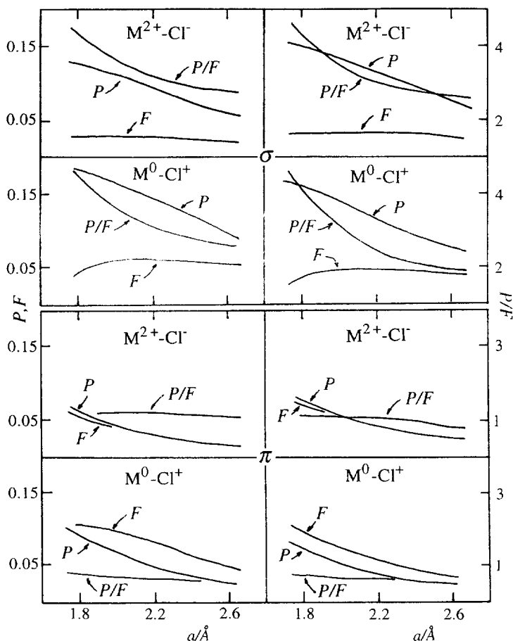
Fig. 14. Trends in P and F integrals, and in their ratios as functions of charge distribution and bond length for \sigma and \pi interactions, after [52].
