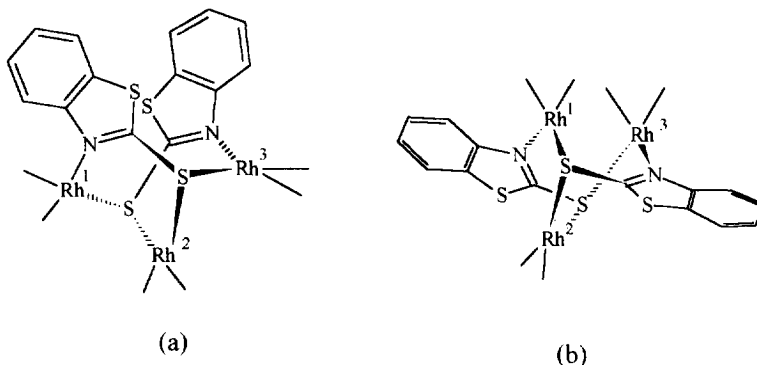
idealised [Rh_3(\mu_3\text{-bztz}2S)_2] conformers (XLIV)
