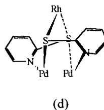
('M 3 (μ 3 -py2S) 2 ' conformers)
