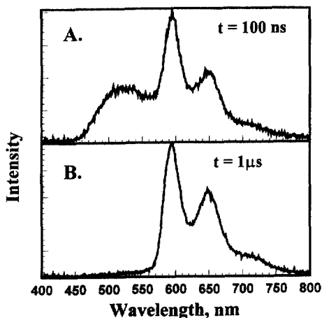
Fig. 3. Gated emission spectra of [(\text{CO})_3\text{Re}(\text{AN})(\text{sty\_bpy})]^+ in 4:1 EtOH:MeOH at 77 K obtained (A) 100 ns following excitation and (B) 1 \mu\text{s} following 337 nm excitation. Gate width 100 ns.
