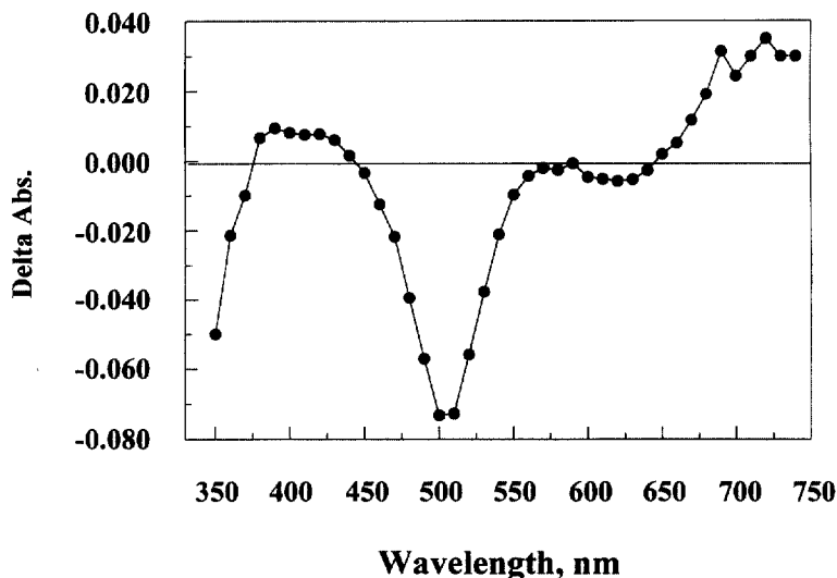
Fig. 7. Excited state absorption spectrum of \{[(\text{bpy})_2\text{Ru}]_2\text{bbdb}\}^{4+} in \text{CH}_3\text{CN} 200 ns following excitation at 532 \text{ nm} .
