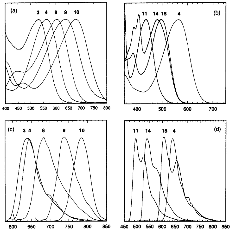
Fig. 1. Normalized absorption and emission bands for Pt(dimimine)(dithiolate) complexes: (a) solvatochromic absorption bands for Pt(diimine)(tdt) complexes in dichloromethane; (b) solvatochromic absorption bands for Pt(dbbpy)(dithiolate) complexes in dichloromethane; (c) emission bands for Pt(diimine)(tdt) complexes in frozen butyronitrile at 77 K; (d) emission bands for Pt(dbbpy)(dithiolate) complexes in frozen butyronitrile at 77 K.
