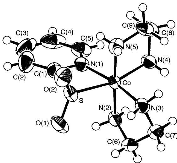
Fig. 3. An ORTEP drawing for the complex cation, [Co(pysi- N,S )(en) 2 ] 2+ ( 3 ), in cocrystal 3/5 . The sulfinate site of 5 is omitted for clarity. The thermal ellipsoids are drawn at 50% probability.
