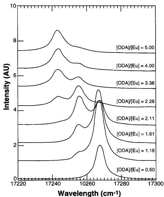
Fig. 2. {}^7F_0 \rightarrow {}^5D_0 Eu(III) excitation spectra for solutions containing various [Eu(III)]:[oxydiacetate] ratios. [Eu(III)] {}_T = 0.020 M. Adapted from ref. [55].
