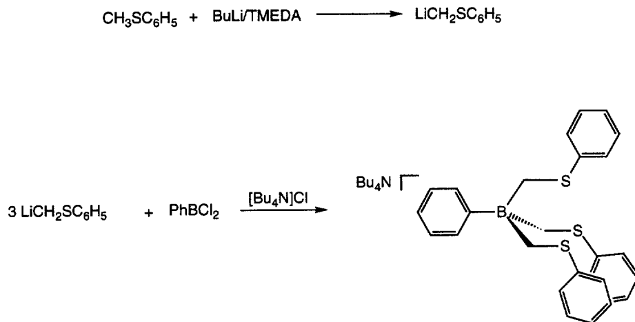
Scheme 1. Ligand synthesis.
