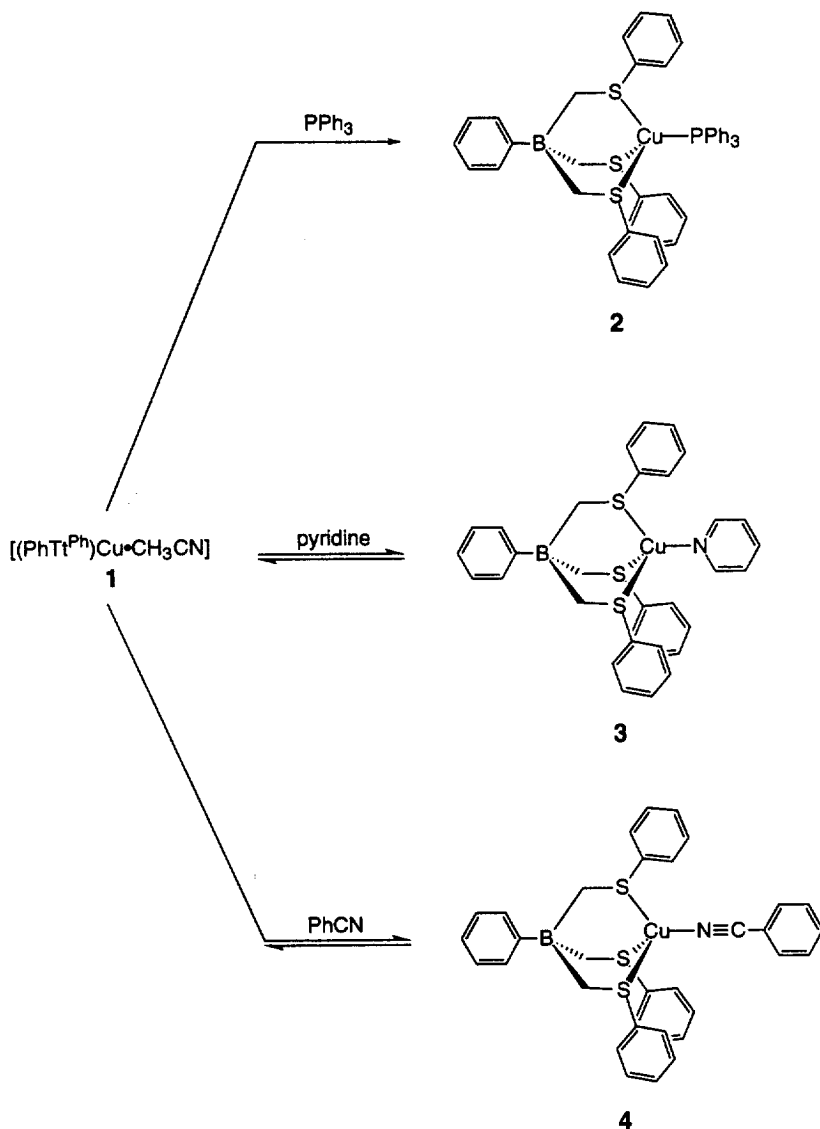
Scheme 2. Substitution reactions.
