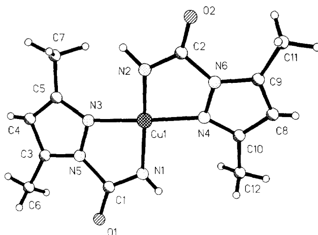
Fig. 1. Molecular structure of [\text{Cu}(\text{dmpz} \cdot \text{NCO})_2] ( 1a ).
