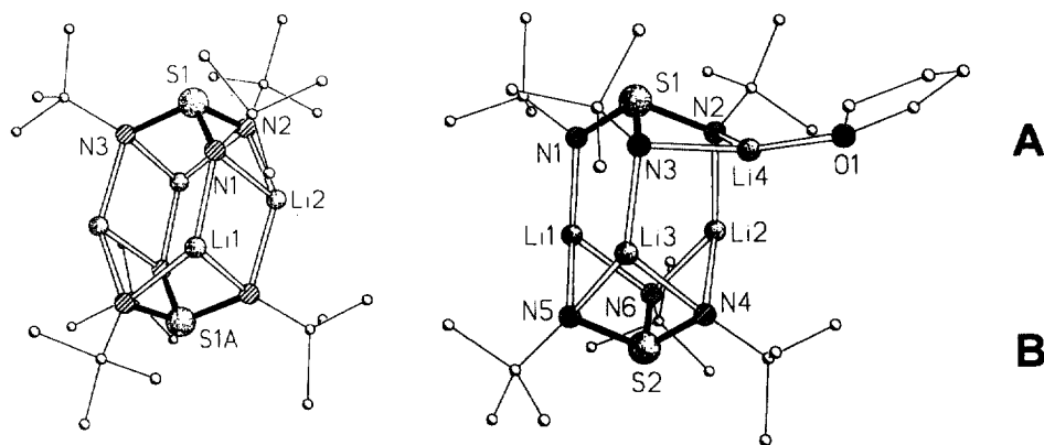
Fig. 3. Solid state structures of [\{\text{Li}(\text{N}'\text{Bu})_3\text{S}\}_2] and [\text{thfLi}_4\{(\text{N}'\text{Bu})_3\text{S}\}_2] .
