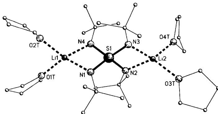
Fig. 9. Solid state structure of [\text{thf}_4\text{Li}_2(\text{N}'\text{Bu})_4\text{S}] .
