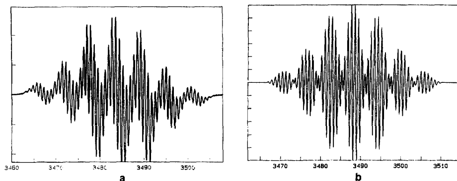
Fig. 4. Experimental ESR-spectrum (a) from oxidized [\text{Li}_4\{(\text{N}^t\text{Bu})_3\text{S}_2\}] in hexane solution in comparison to the calculated spectrum of [\text{Li}_3\{(\text{N}^t\text{Bu})_3\text{S}_2\}]^\bullet (b).
