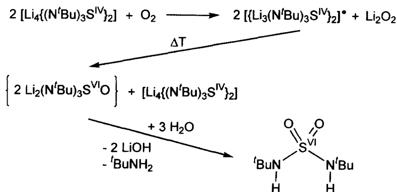
Scheme 2. Tentative mechanism for the oxidation of [\text{Li}_4\{(\text{N}^t\text{Bu})_3\text{S}\}_2] by \text{O}_{2(\text{g})} .
