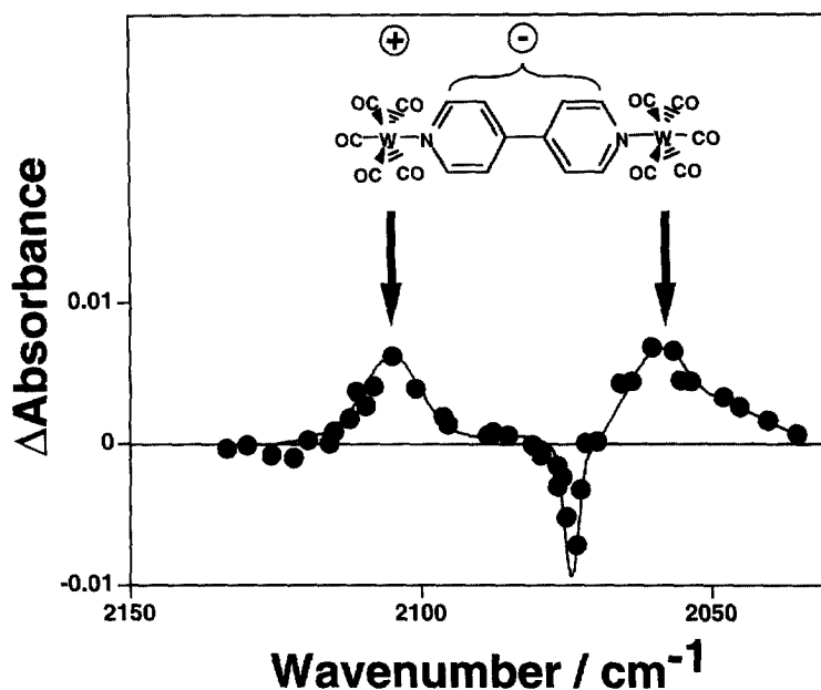
Fig. 5. TRIR spectrum of [(\text{CO})_5\text{W}(4,4'\text{-bpy})\text{W}(\text{CO})_5] obtained 100 ns following 355 nm photolysis.
