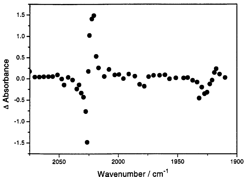
Fig. 2. TRIR spectrum of [\text{ClRe}(\text{CO})_3(\text{dppz})] in \text{CH}_2\text{Cl}_2 obtained 100 ns after 355 nm photolysis.
